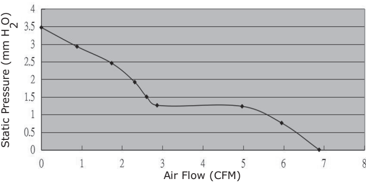
CFM-4020CF-055-212
