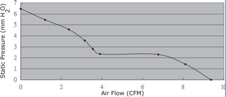
CFM-4020CF-075-306
