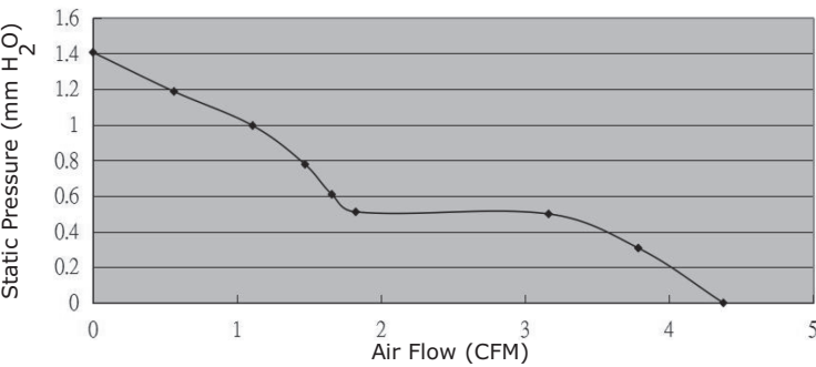
CFM-4020CF-035-114
