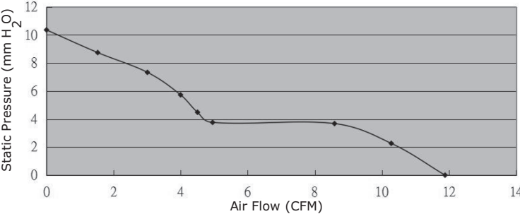
CFM-4020CF-095-342
