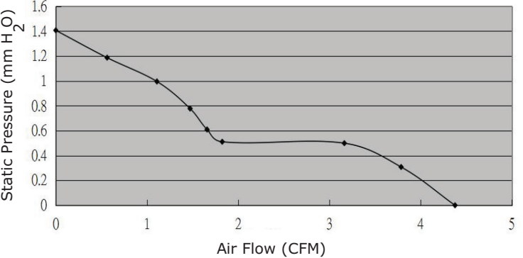
CFM-4020CF-135-114
