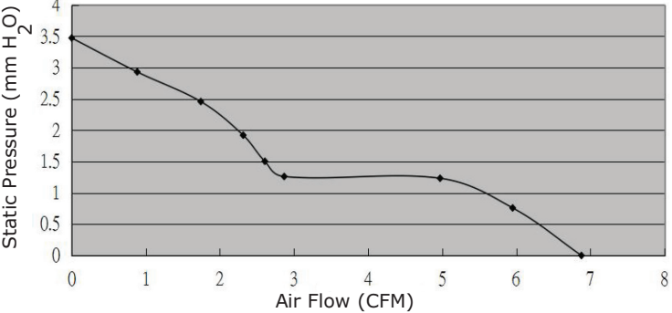
CFM-4020CF-155-212
