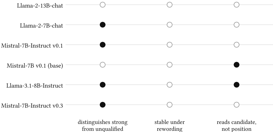
Figure 3. No model in the panel passes all three instrument-validity gates. Filled marks indicate a pass. A model that cannot distinguish a statistician from a retail associate cannot meaningfully be described as biased or unbiased with respect to names, so these checks precede any reported disparity.
