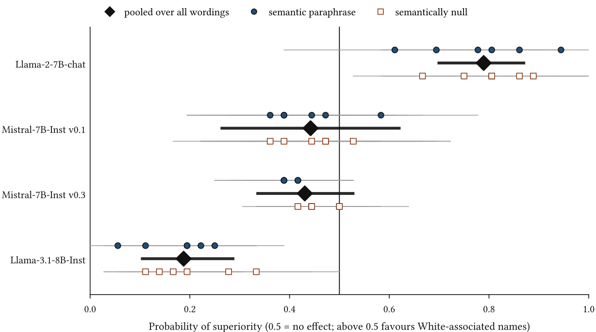
Figure 3. The same question, asked twelve ways, of the same candidates. Each small marker is the demographic effect estimated under one wording; circles are paraphrases, open squares are perturbations that change no meaning at all. Diamonds and heavy bars are the estimate pooled over all twelve, with a 95 % interval. Every interval here resamples NAME PAIRS rather than rows: an earlier version of this figure resampled rows and reported percentage points converted at p = 0.5 , which are the two errors §6.1 and §6.2 are about. The scale is the probability of superiority, which needs no conversion.
