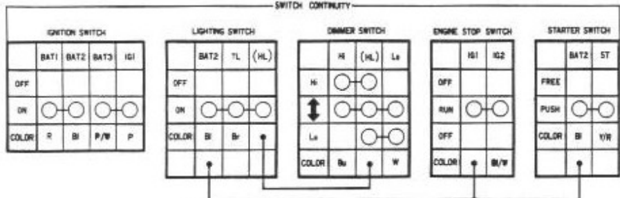
SWITCH CONTINUITY
