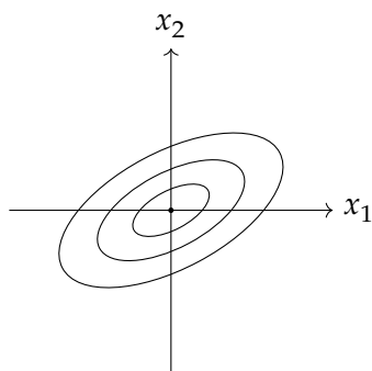
positive covariance
