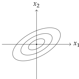
positive covariance
