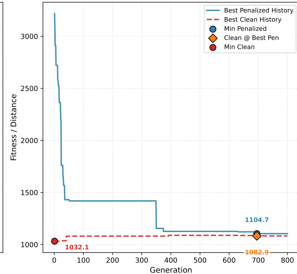
( \mu + \lambda ) Evolution Strategy
