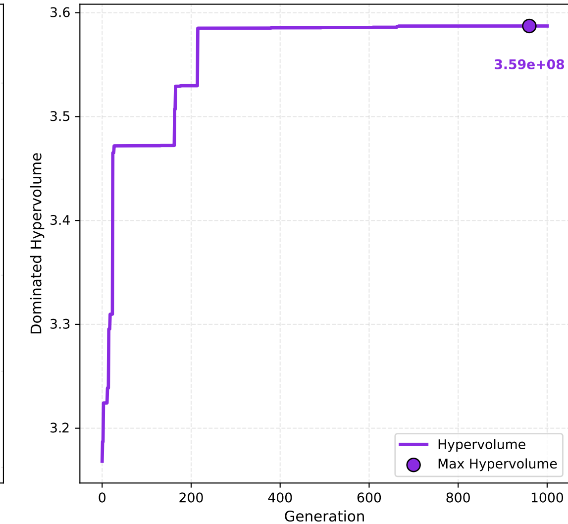
NSGA-II (Hypervolume)
