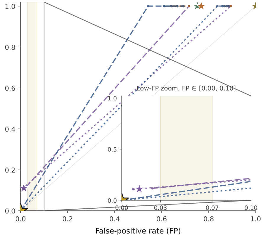
B. Recommender — MovieLens-25M, horizons h=40/50/60
