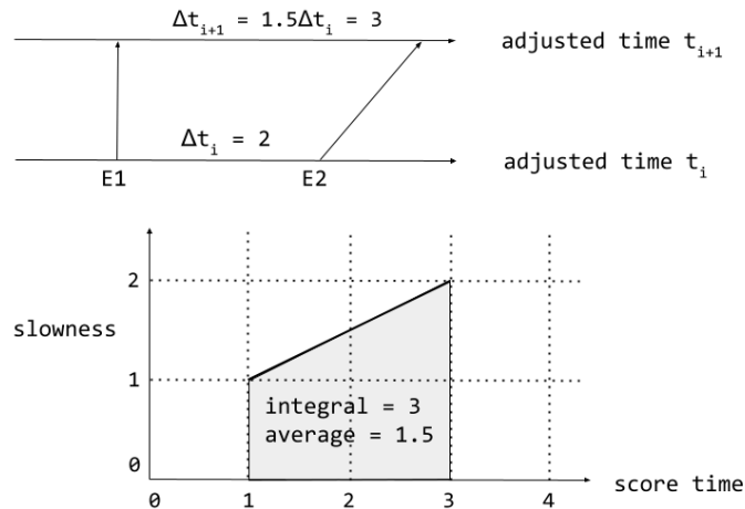
Figure 5. Example of tempo adjustment. Events E1 and E2 have score times 1 and 3, and adjusted times determined by earlier transformations. In transformation i , the interval in adjusted time between the events is scaled by the average value of the slowness (inverse tempo) function between their score times.
