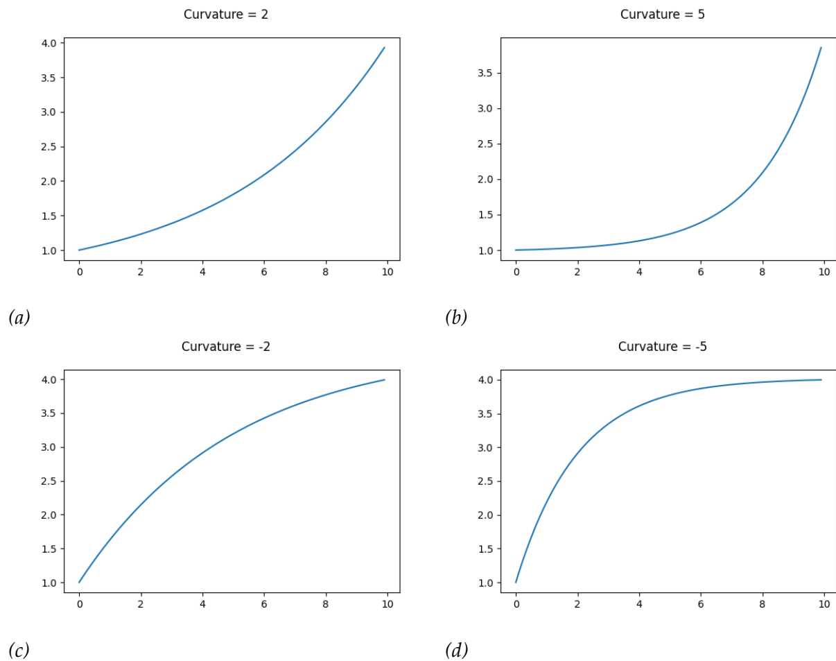
Figure 3. Shifted-exponential primitives with different curvatures.
