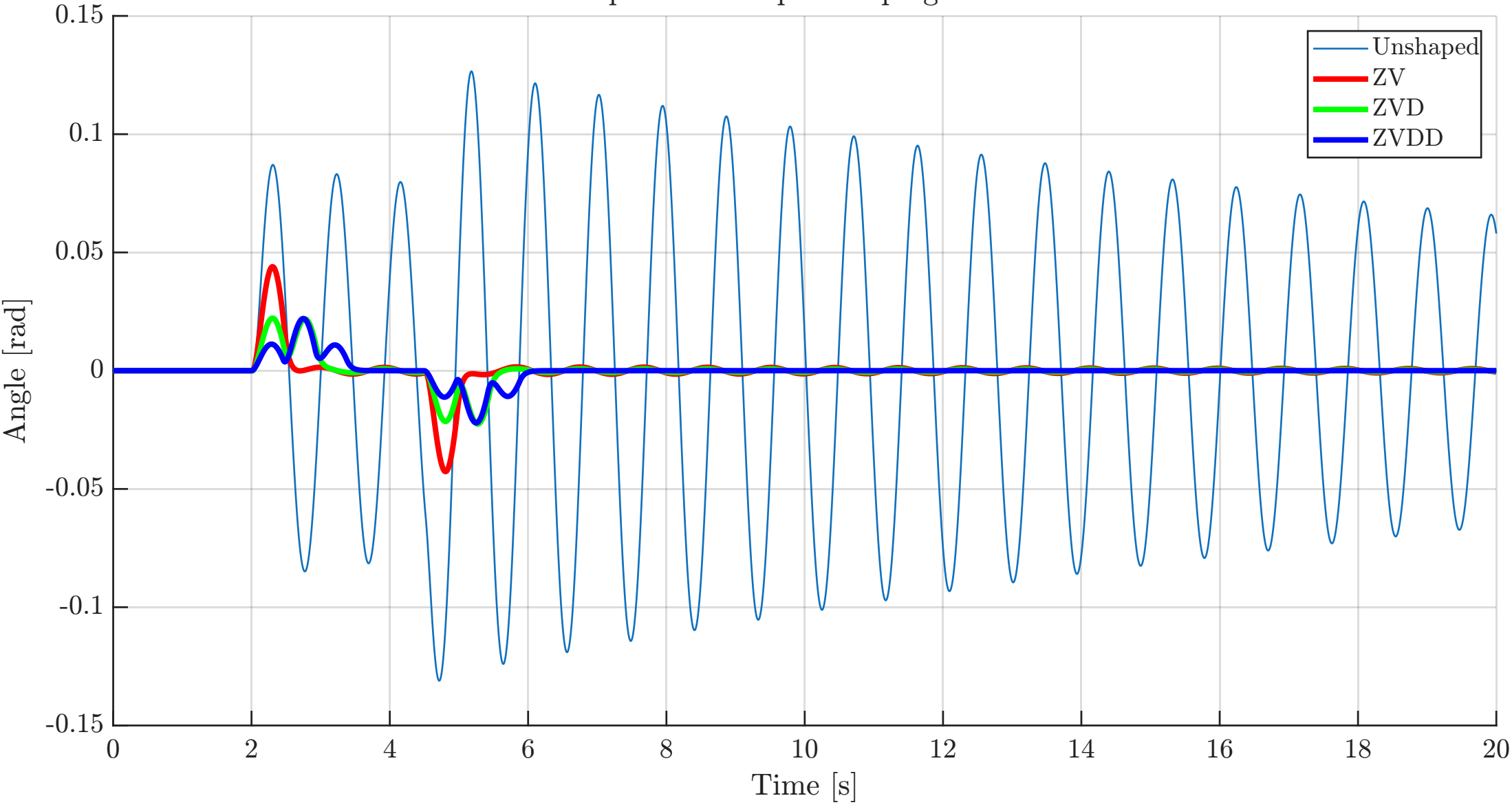
Comparison of Input Shaping Methods
