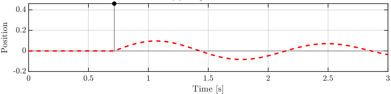
(c) Superposition (ZV - zero residual vibration)
