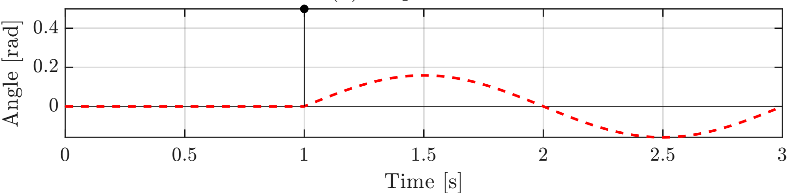
(c) Superposition (ZV - zero residual vibration)
