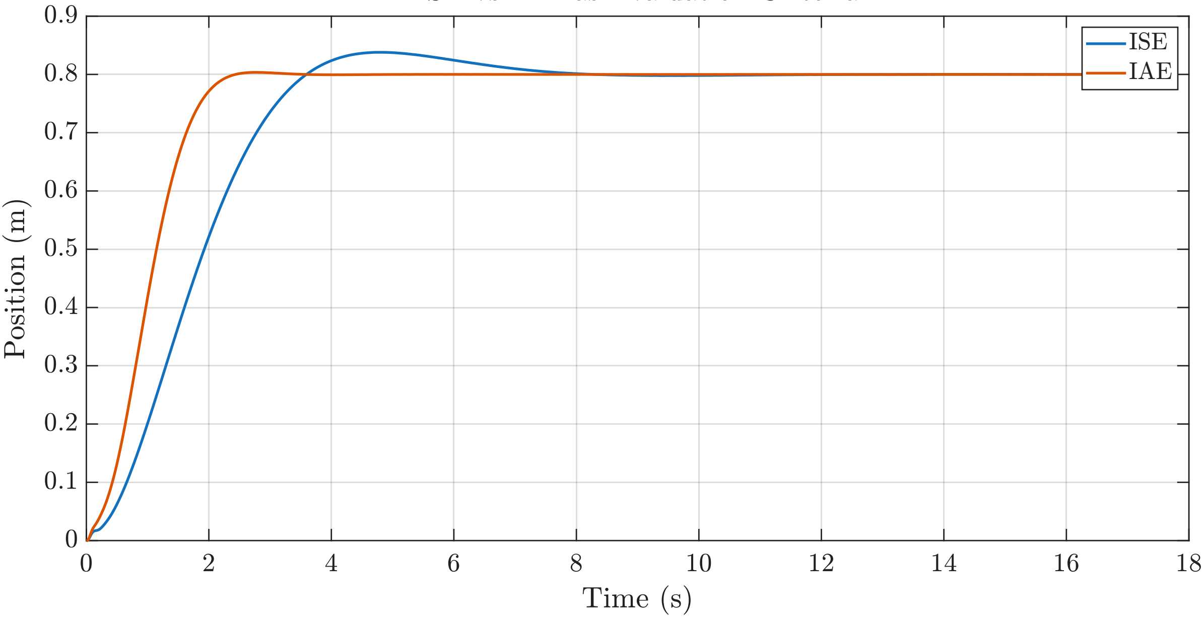
ISE vs IAE as Evaluation Criteria
