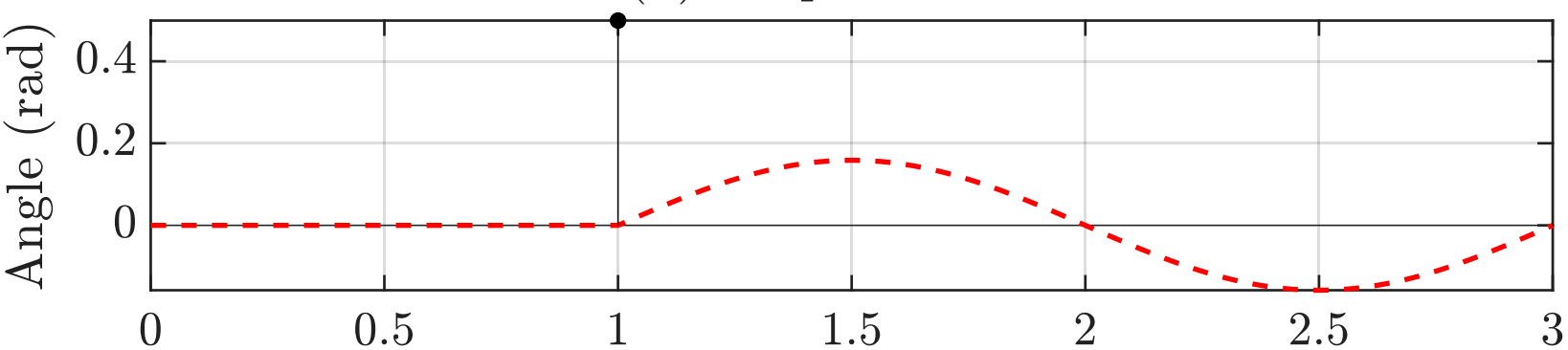
(b) Response to A_2
