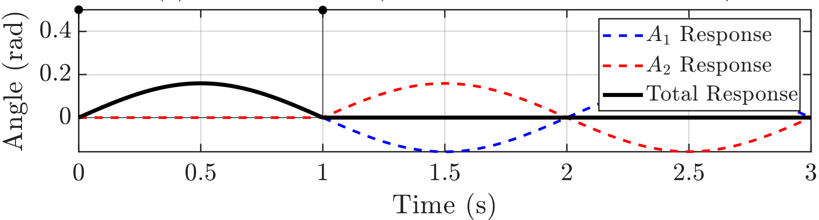
(c) Superposition (ZV - zero residual vibration)
