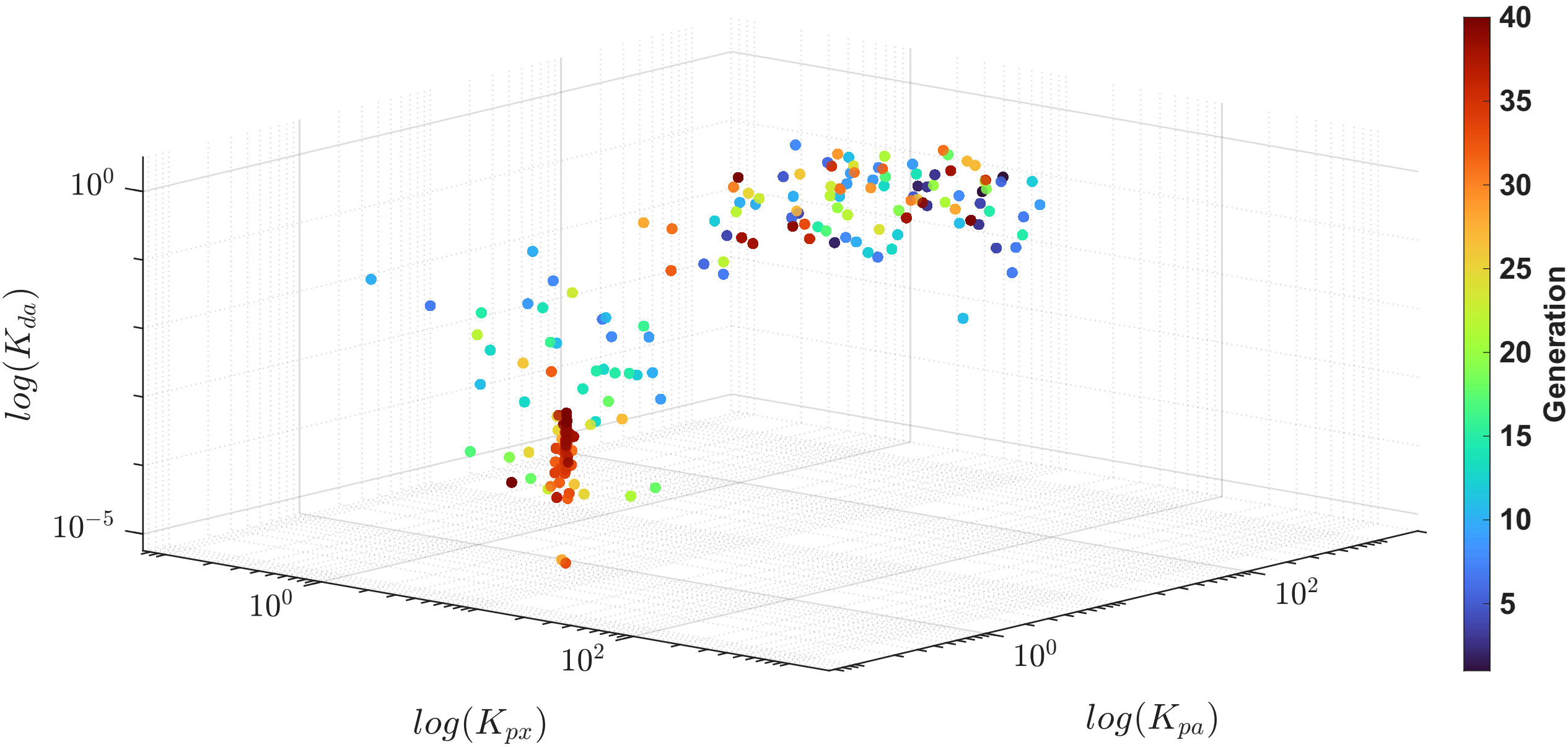
PSO Particle Evolution
