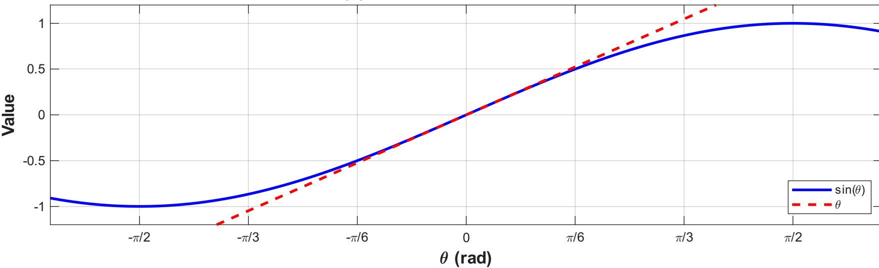
\sin(\theta) and Linear Approximation
