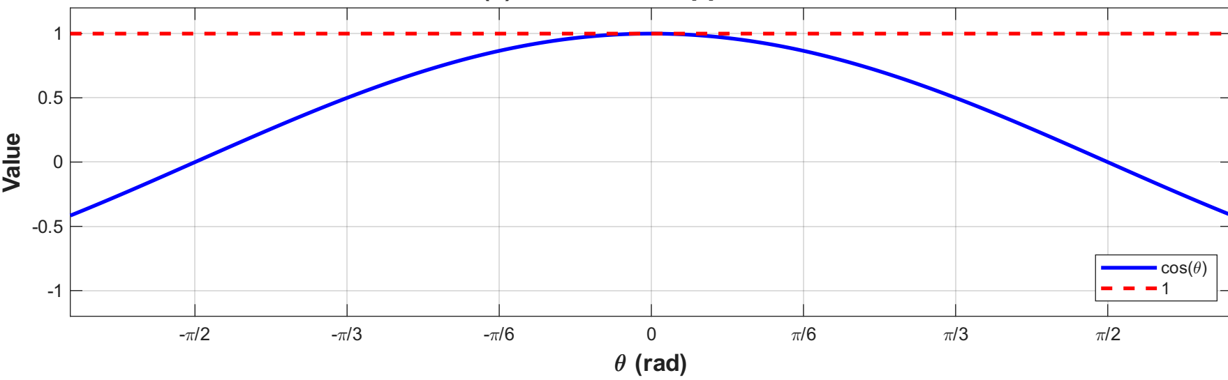
\cos(\theta) and Linear Approximation
