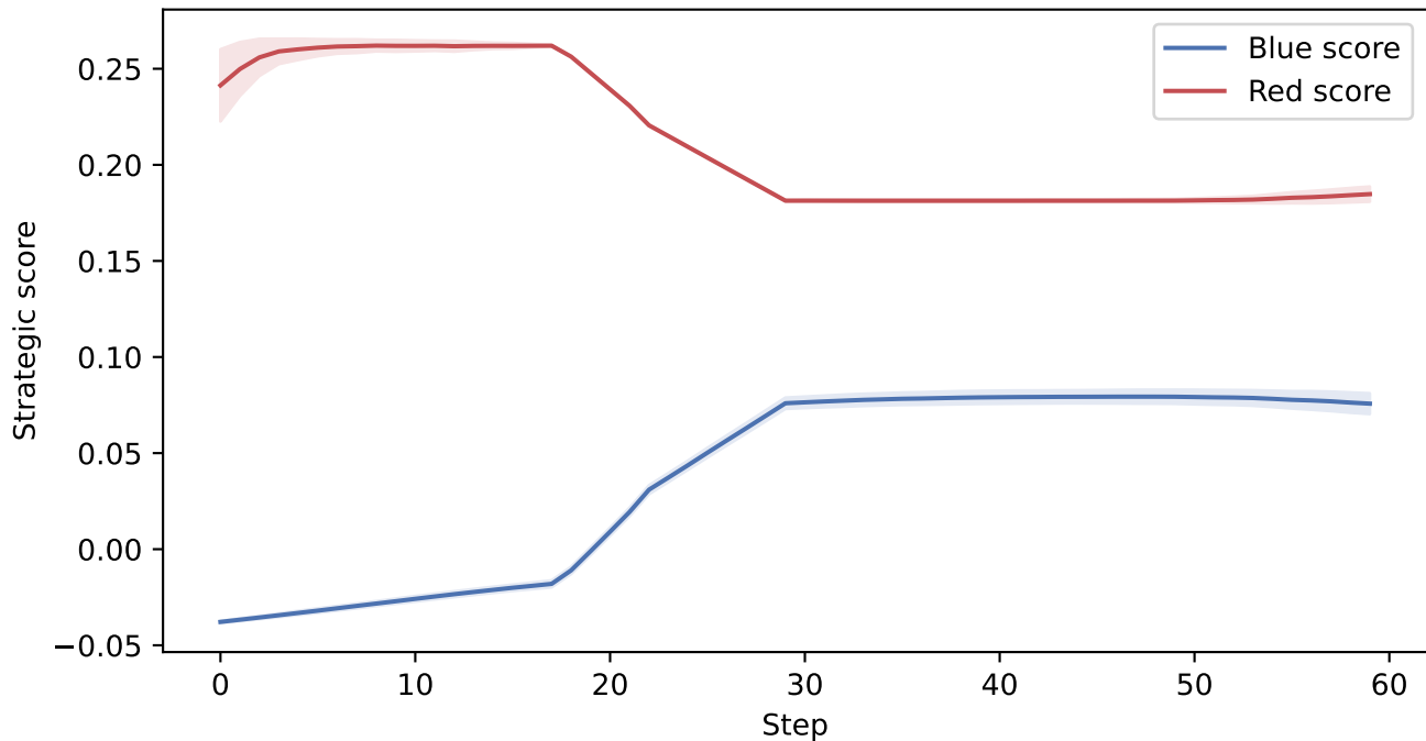
Mean Strategic Score Trajectories
