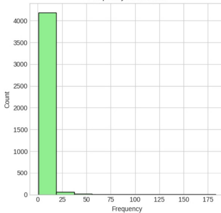
Frequency Distribution
