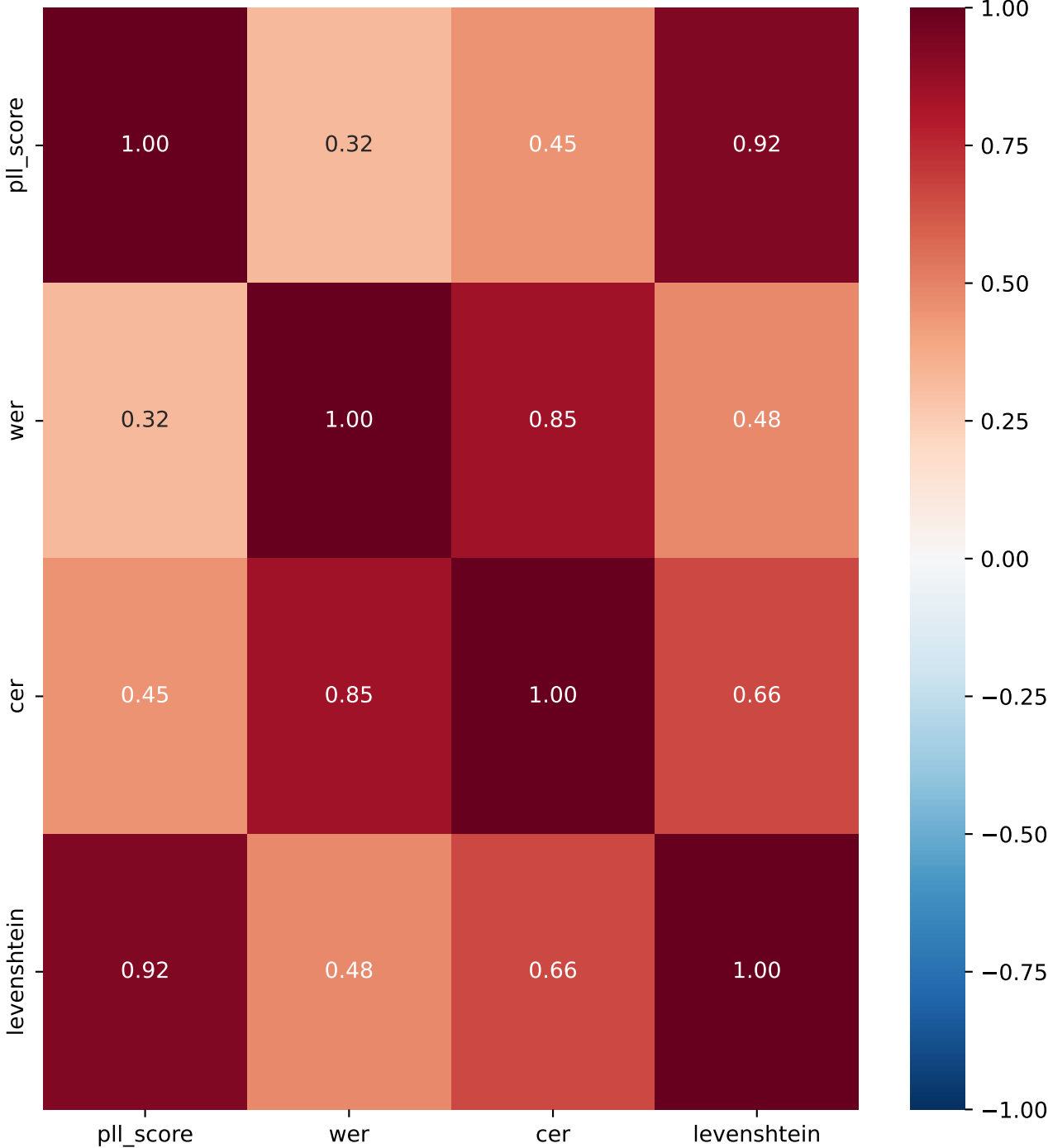
Pooled Pearson matrix
