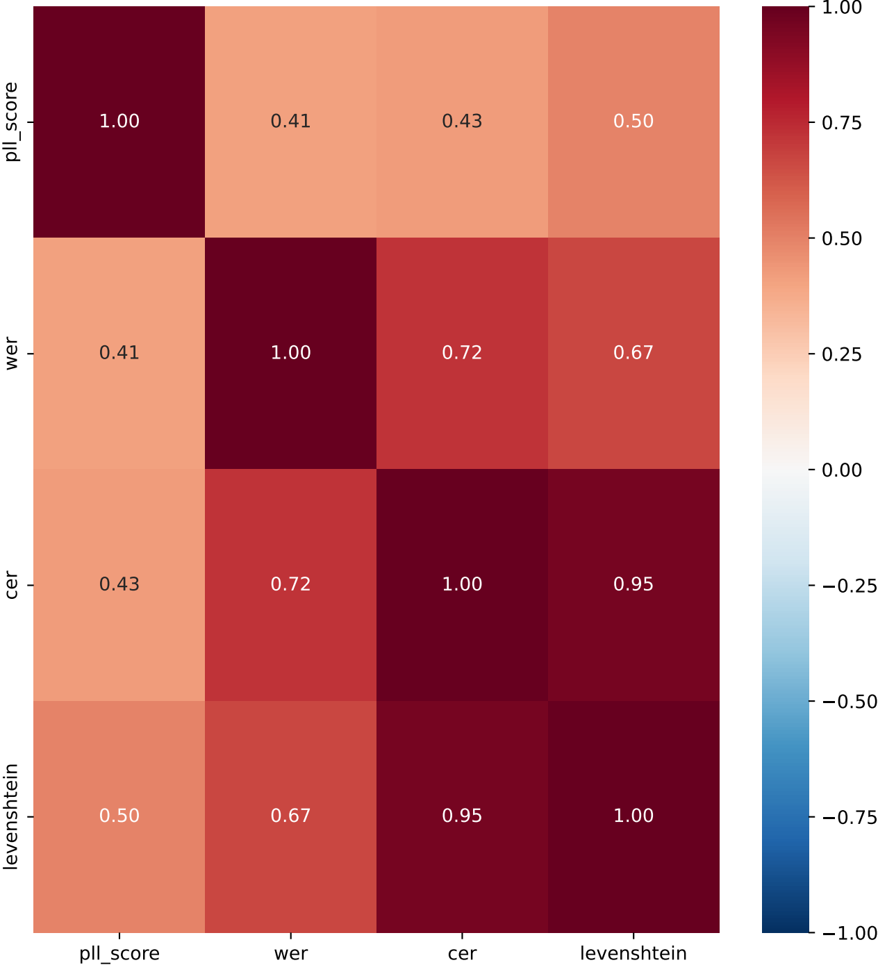
Equal-weight mean Pearson matrix
