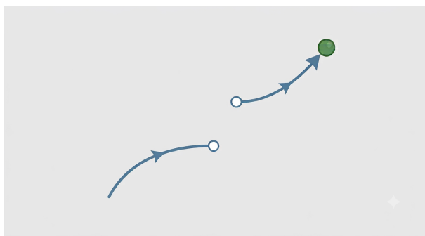
Figure 2.4: Cartoon schematic of a particle (green) moving along a discontinuous trajectory (blue) with discontinuity represented by open circles.
