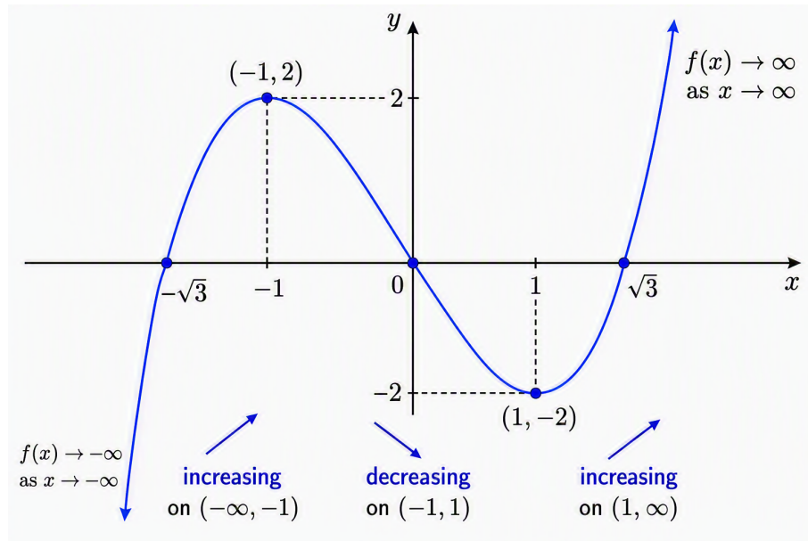
Figure 5.1: Example of curve sketching the function f(x) = x^3 - 3x .
