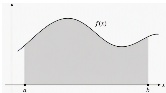
(a) Shaded region representing area under curve of function f(x) over interval [a, b] .
