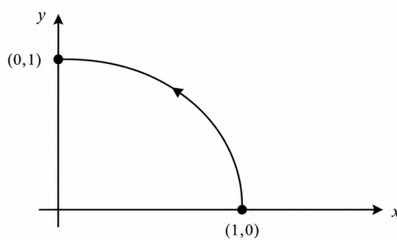
(b) Illustration of curve given in Example 5.25.
