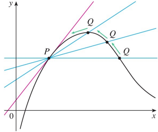
(b) Schematic of line PQ approximating the tangent line (red) as x \rightarrow a .
