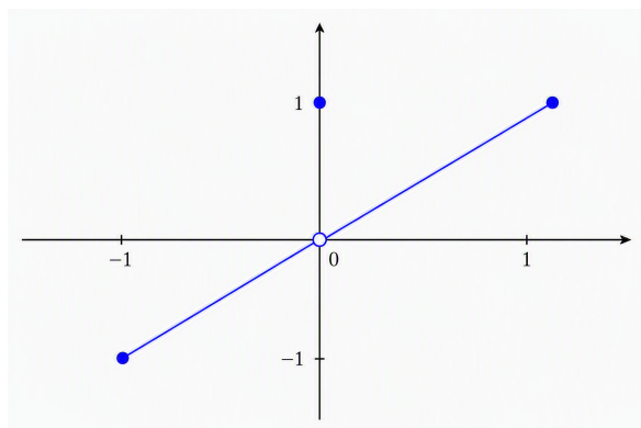
(a) Plot of the function from Example 2.21.
