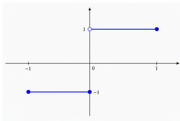
(b) Plot of the function from Example 2.22.
