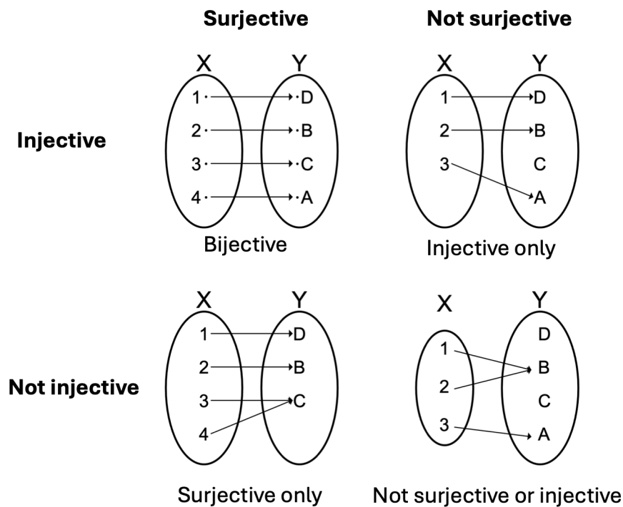
Figure 1.2: Diagram illustrating the different types of functions, with examples represented by arrows mapping elements of domain X to elements of codomain Y . Columns split examples by whether the function is surjective or not, while rows split examples by whether the function is injective or not. Top left gives an example of a bijective function (both surjective and injective), off diagonals are examples of functions that are only surjective or injective, and bottom right gives an example of a function that is neither. Adapted from Wikipedia, Original: Schapel; vectorized by Samuel Mediani.
