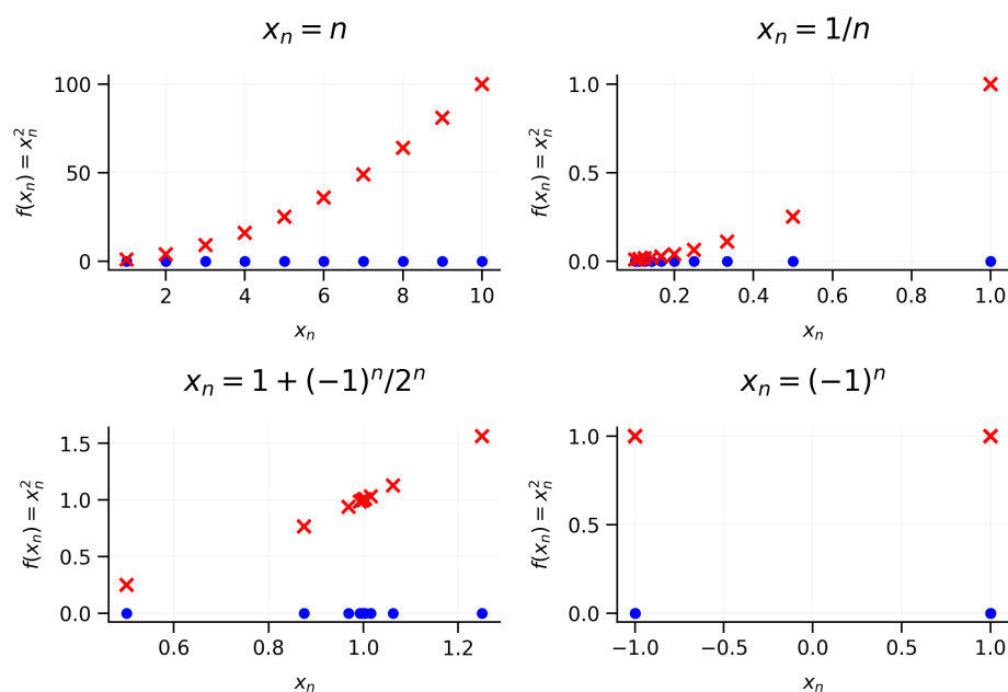
Figure 2.2: Visualisation of the first ten terms in sequences (x_n)_{n=1}^{\infty} and (f(x_n))_{n=1}^{\infty} , where the latter is obtained by applying the function f(x) = x^2 to the examples described in text. In this representation, the blue dots corresponding to the values x_n are now plotted on the x-axis (real interval) and the corresponding values of f(x_n) are now plotted as red crosses on the y-axis.
