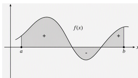
(b) Positive (labelled “+”) and negative (labelled “-”) contributions to area.
