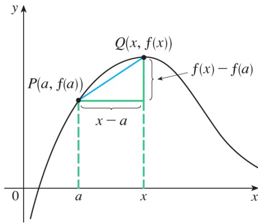
(a) Illustration of curve given by y = f(x) with calculation of the slope of the line PQ .
