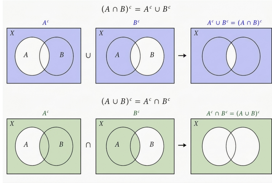
Figure 1.1: Diagram illustrating De Morgan's Laws, involving subsets A, B \subset X and their complements in X . The shaded regions denote the corresponding sets.
