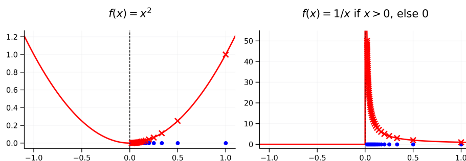
Figure 2.3: Visualisations of continuity and discontinuity defined using convergent sequences. On the left, the function f : [-1, 1] \rightarrow \mathbb{R} given by f(x) = x^2 is plotted in red, with blue dots representing the sequence given by x_n = 1/n and red crosses denoting corresponding values of f(x_n) . Although just one sequence is plotted in this case, it should be clear that any other converging to 0 in [-1, 1] would generate red crosses that similarly converge to f(0) = 0 , since the function is continuous at 0. On the right, the function f : [-1, 1] \rightarrow \mathbb{R} given in Example 2.19 is plotted in red, with blue dots representing the sequence given by x_n = 1/n and red crosses denoting corresponding values of f(x_n) . In this case, we see that the red crosses do not converge to f(0) = 0 since the function is not continuous at 0.
