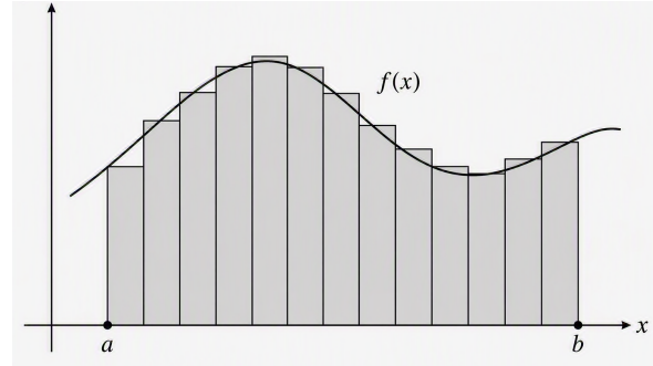
(b) Partitioning area under curve y = f(x) into rectangular regions. More than in panel (a).
