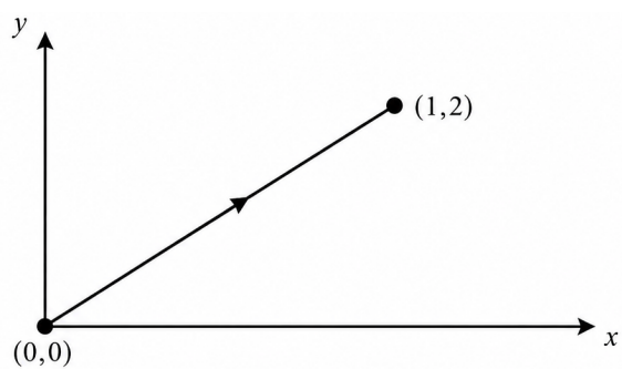
(a) Illustration of curve given in Example 5.24.
