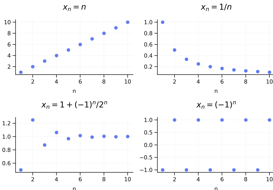
Figure 2.1: Figure illustrating the behaviour of sequences of real numbers corresponding to examples described in text, from n = 1, 2, \dots, 10 . The blue dots correspond to the values of x_n (y-axis) at the corresponding values of n (x-axis).
