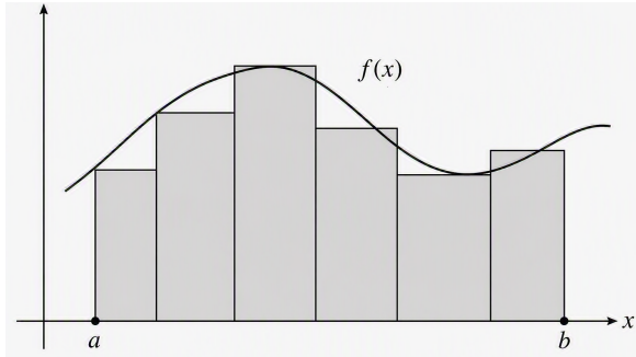
(a) Partitioning area under curve y = f(x) into rectangular regions. Fewer than in panel (b).
