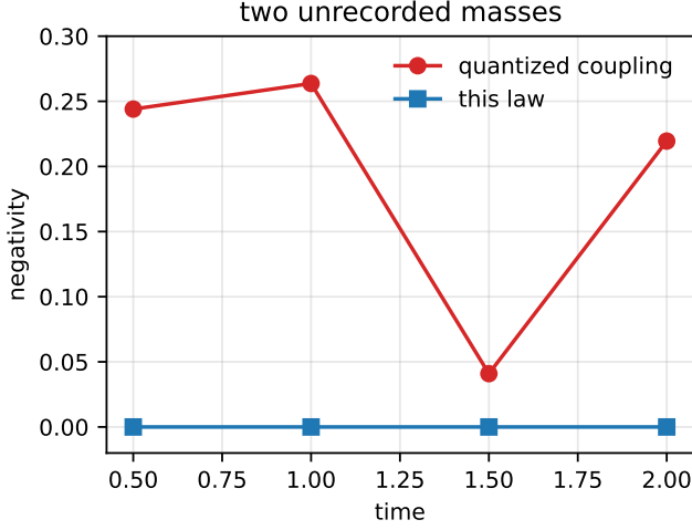
FIG. 2. Two unrecorded masses: negativity under this law’s mean-field form (flat at 1.770e-16 ) against a quantized two-body coupling applied to the same initial state (reaching concurrence 0.5274), which serves as the control.
