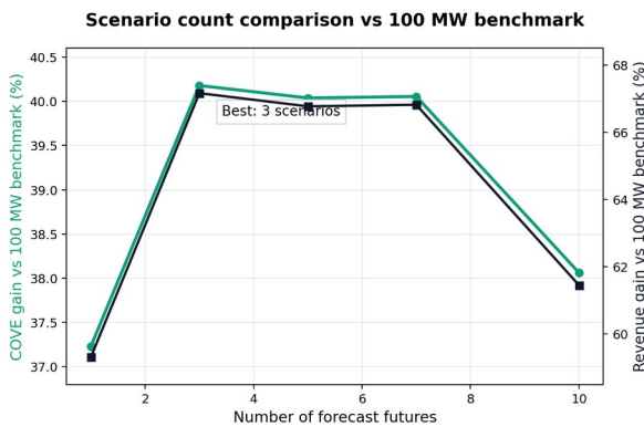
Fig. 13. Scenario count comparison against the 100-MW benchmark.
