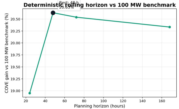
Fig. 9. Deterministic horizon sweep using the 100-MW benchmark as the primary comparison.
