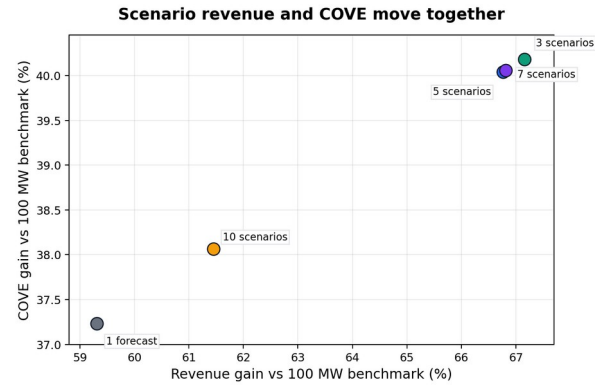
Fig. 15. Revenue and COVE gains move together for the stronger scenario cases.
