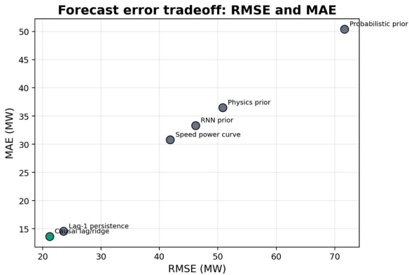
Fig. 6. RMSE and MAE comparison across forecast methods.
