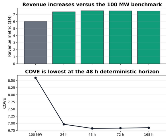
Fig. 11. Deterministic revenue and COVE by horizon.
