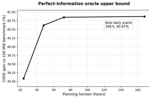
Fig. 18. Perfect-information daily oracle upper bound.
