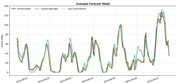
Fig. 7. Example week showing actual power and causal forecasts.
