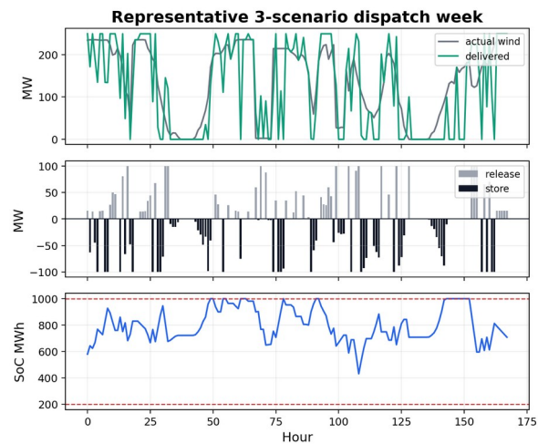
Fig. 17. Representative week for the three-scenario dispatch case.
