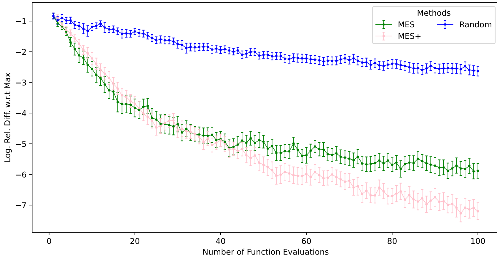
6 Dimensions. Noiseless. Post Mean.
