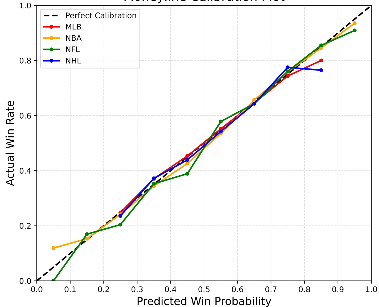
Moneyline Calibration Plot
