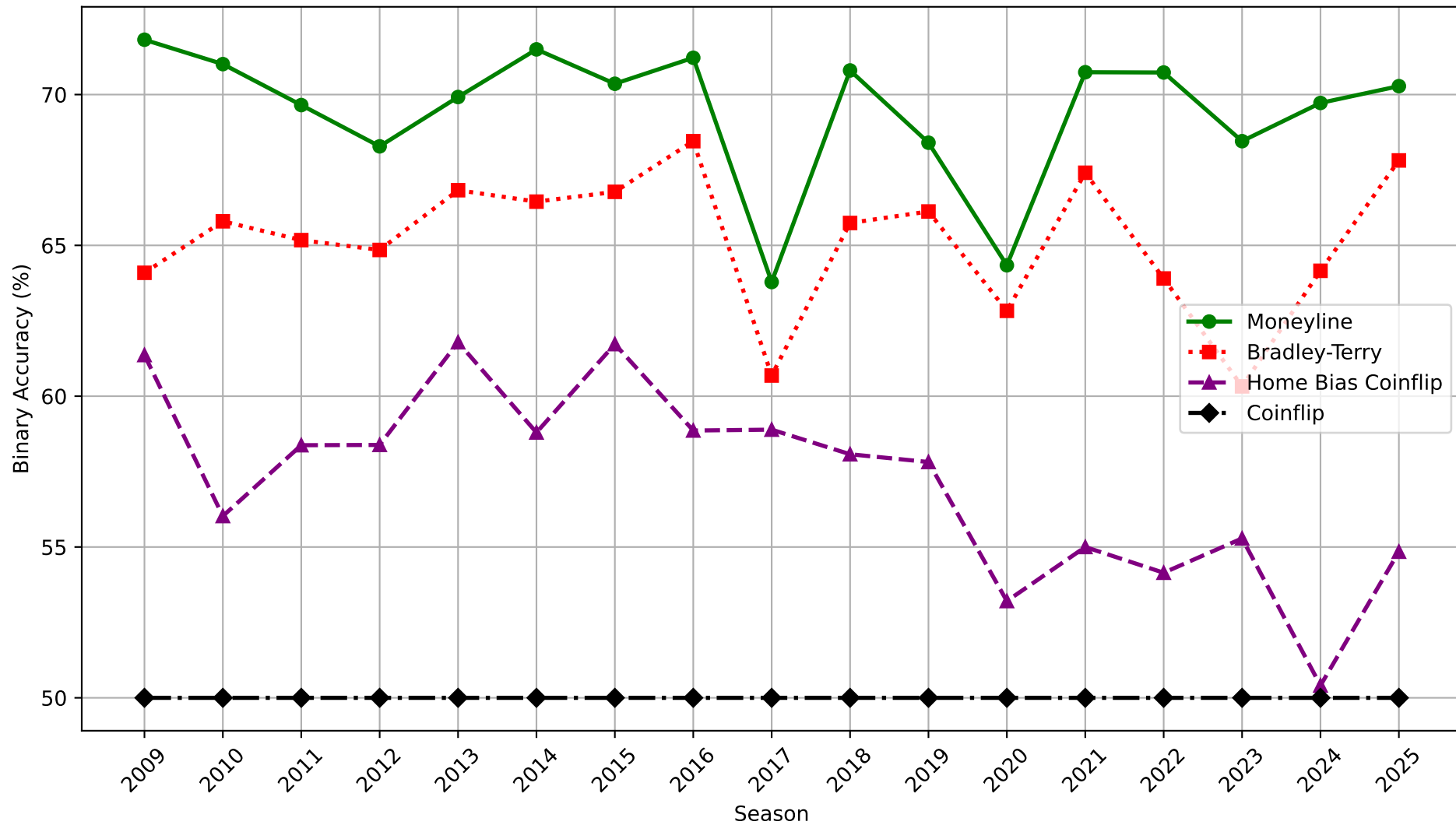
NBA - Binary Accuracy by Season
