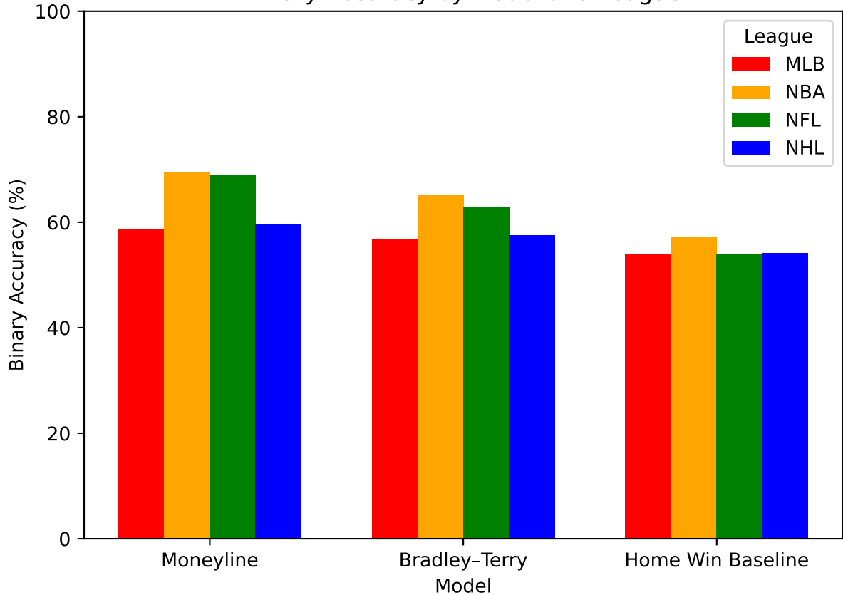
Binary Accuracy by Model and League
