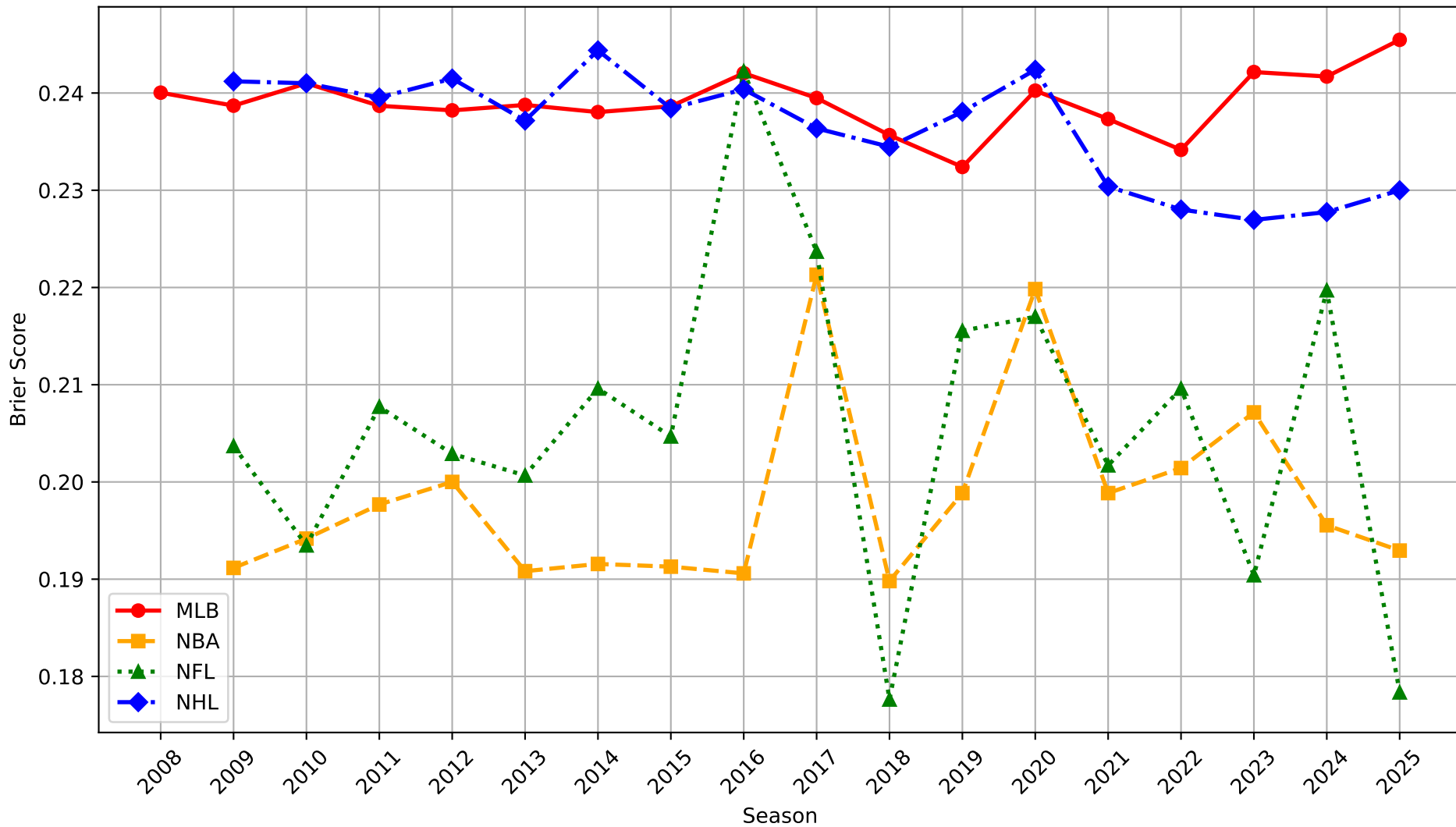
Moneyline Brier Scores by Season
