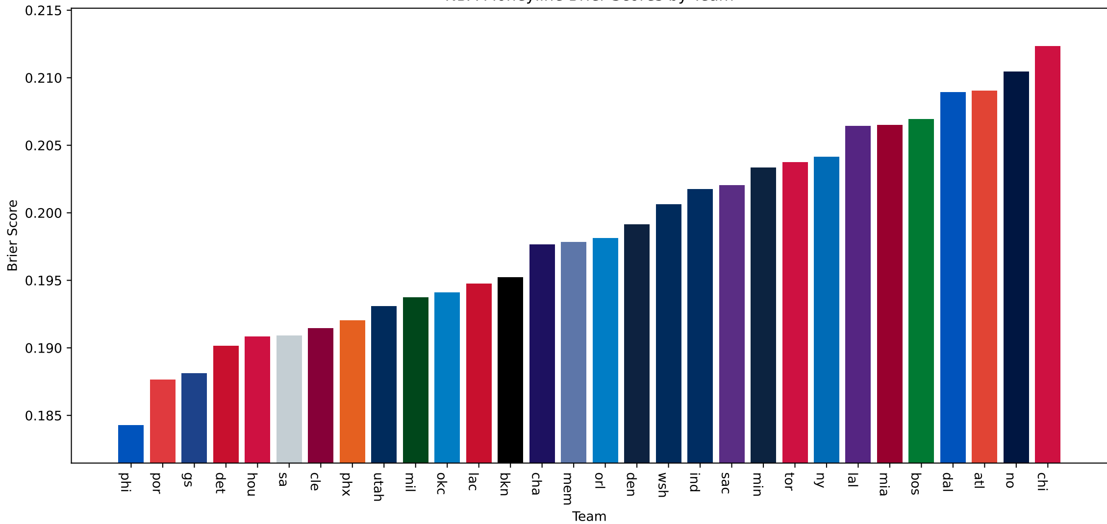
NBA Moneyline Brier Scores by Team
