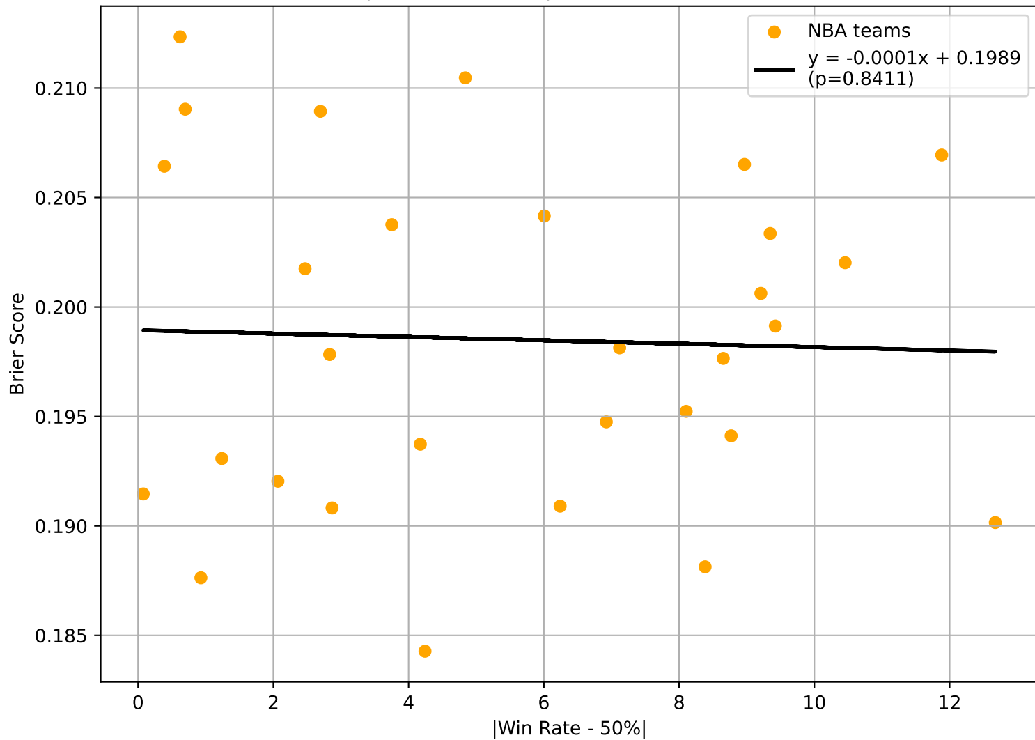
NBA: |Win Rate - 50%| vs Moneyline Brier Score
