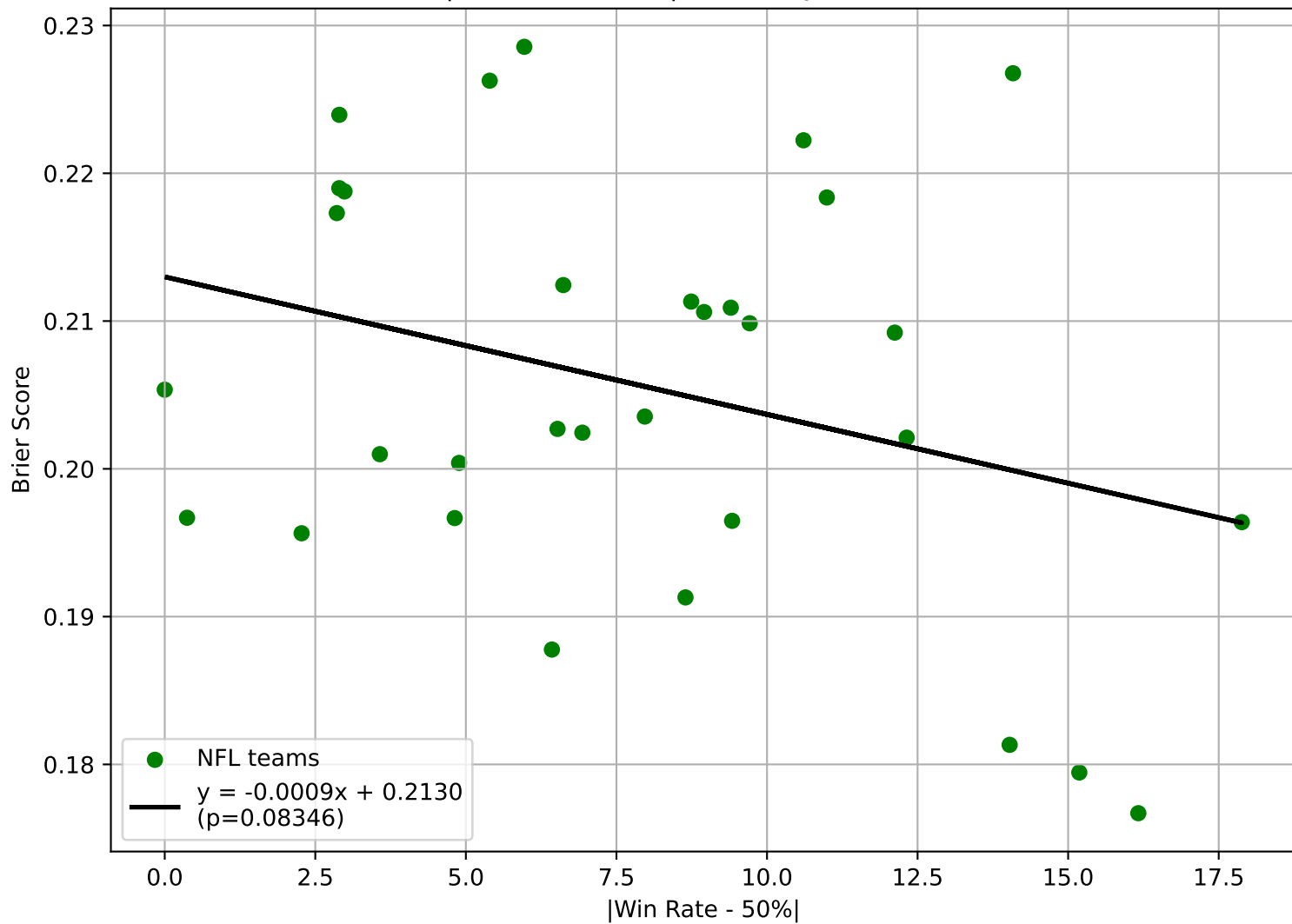
NFL: |Win Rate - 50%| vs Moneyline Brier Score
