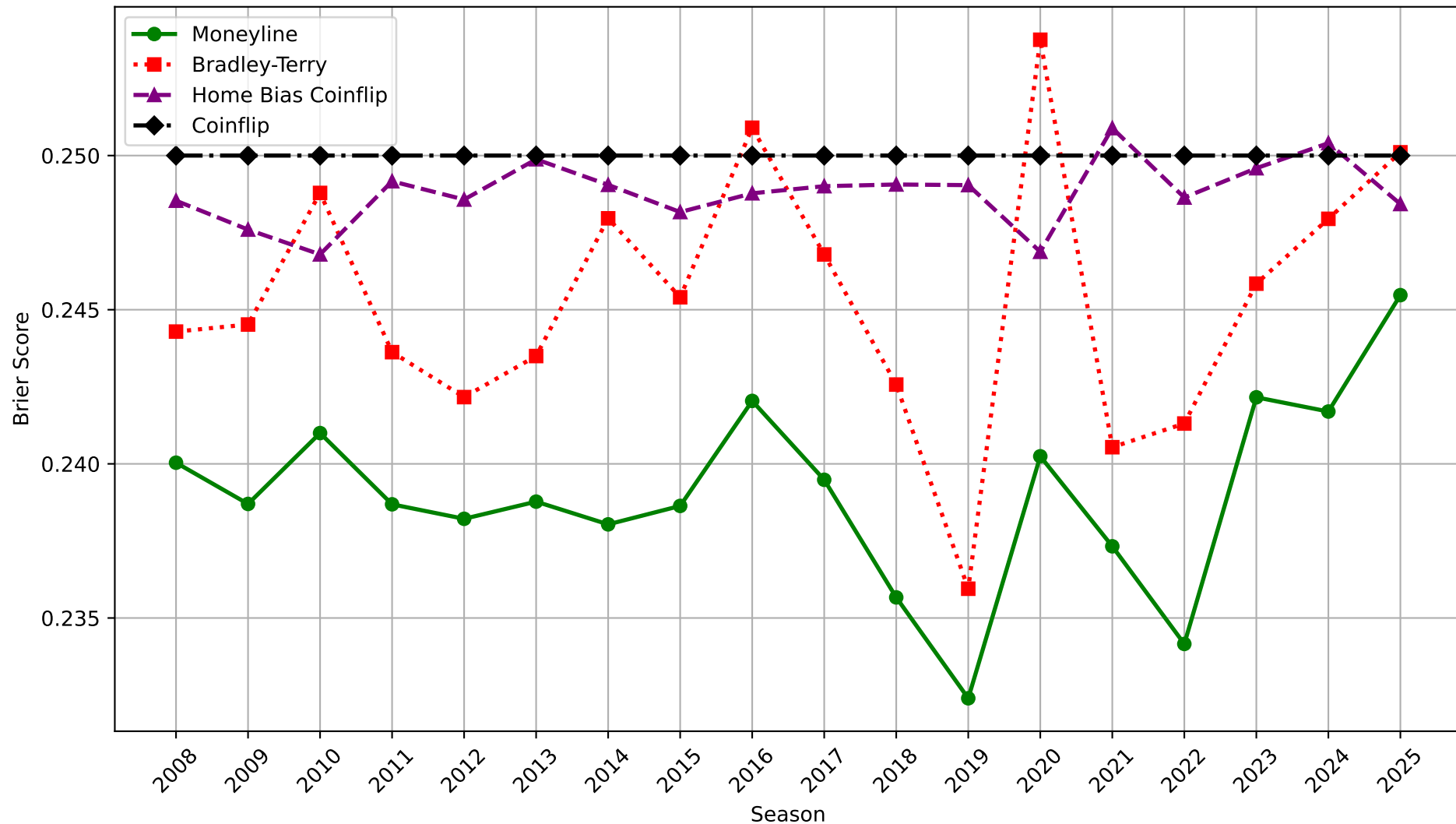
MLB - Brier Scores by Season
