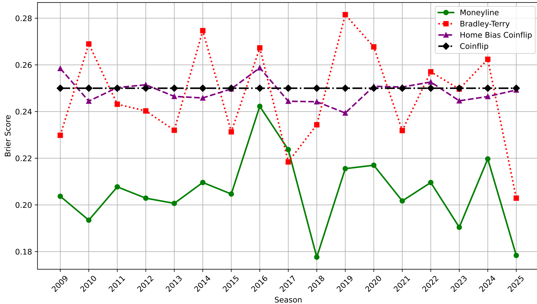
NFL - Brier Scores by Season
