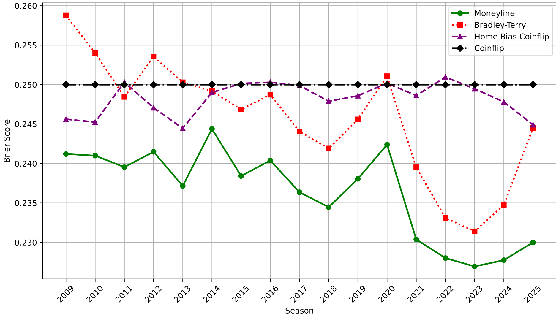
NHL - Brier Scores by Season
