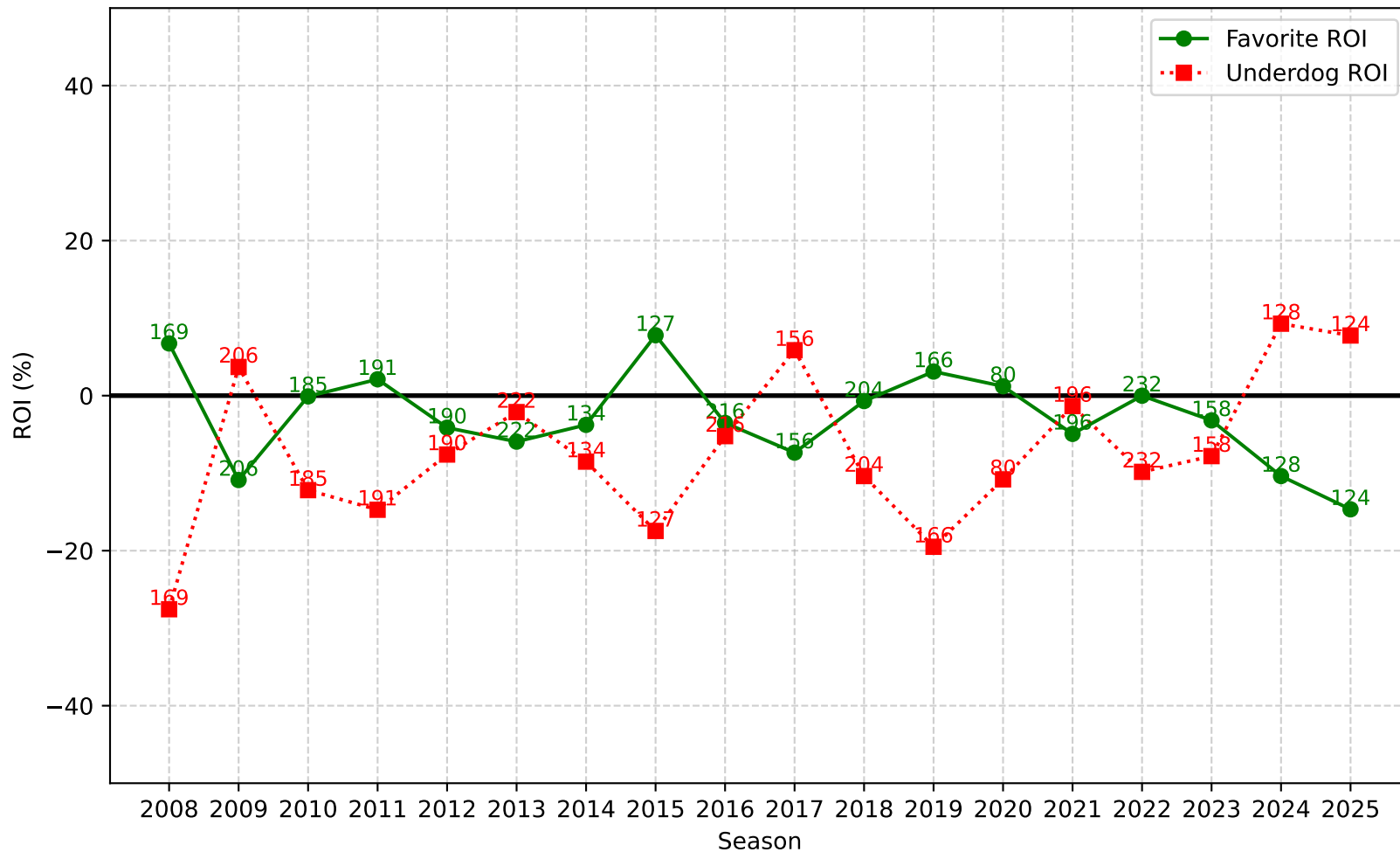
Bradley-Terry 60-70% Bin Favorite vs Underdog ROI by Season
