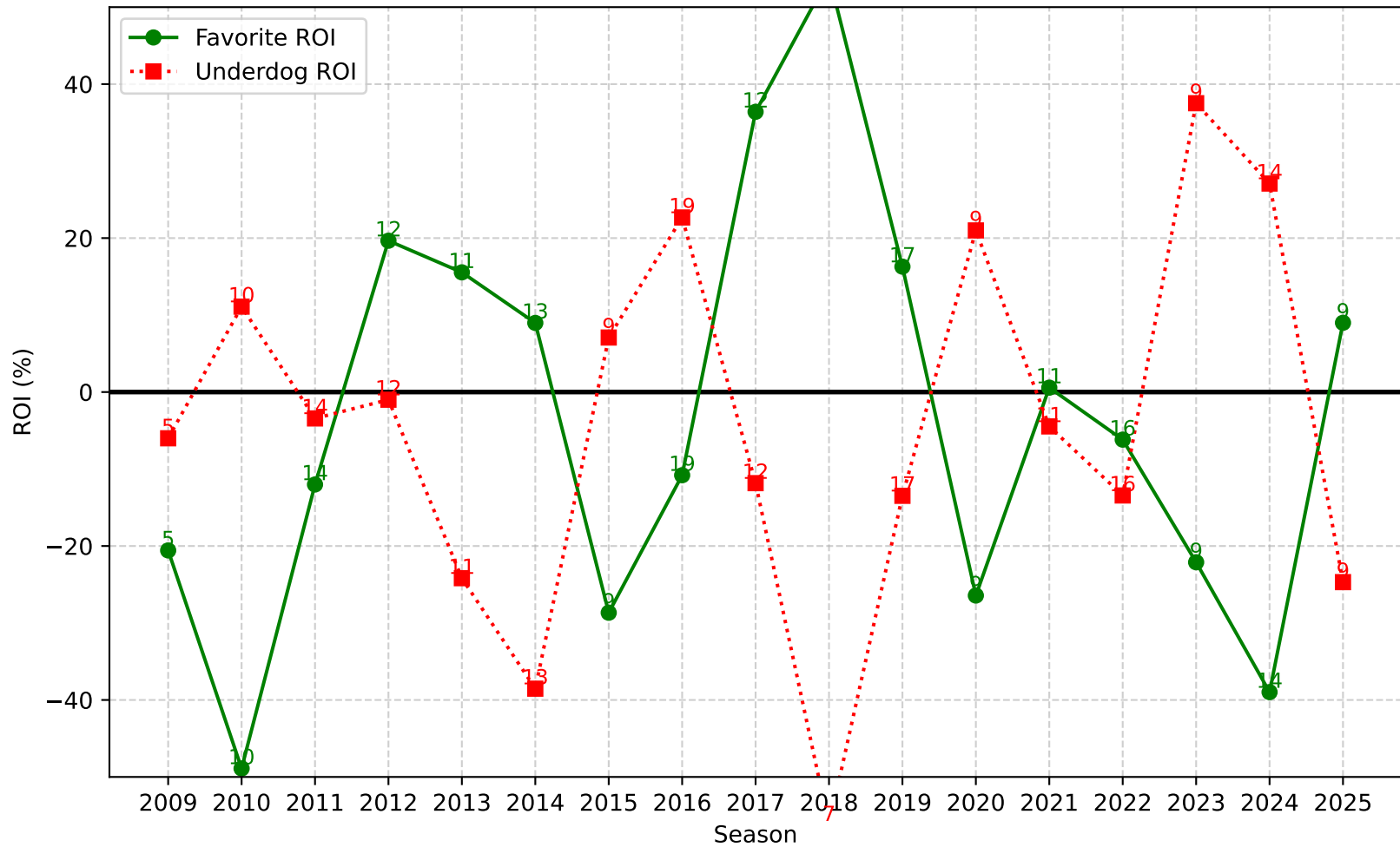
Bradley-Terry 40-50% Bin Favorite vs Underdog ROI by Season
