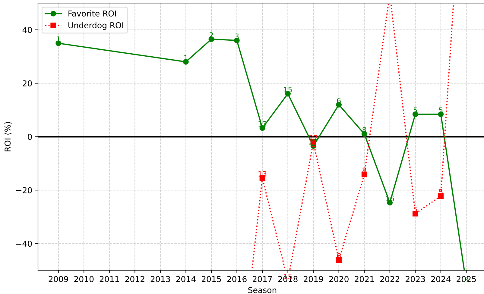
Moneyline 20-30% Bin Favorite vs Underdog ROI by Season
