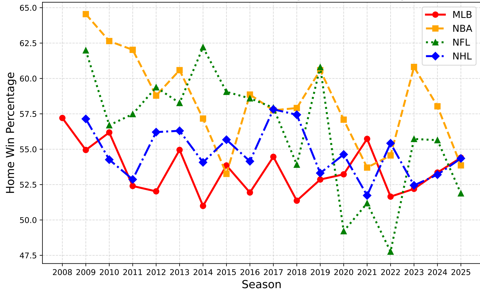
Seasonal Home Win Percentage (First Half Only)
