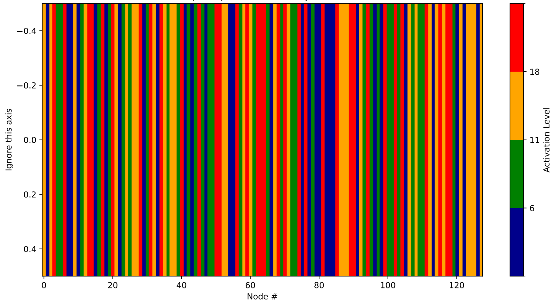
Heatmap - Layer 14 (Probability 3072-3200)
