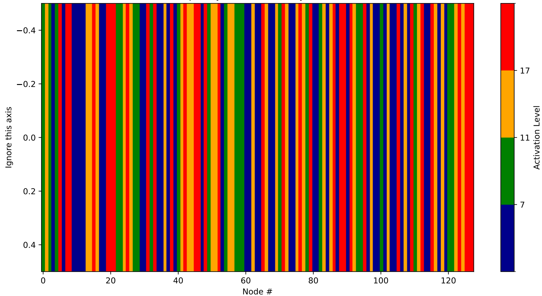
Heatmap - Layer 21 (Probability 2944-3072)
