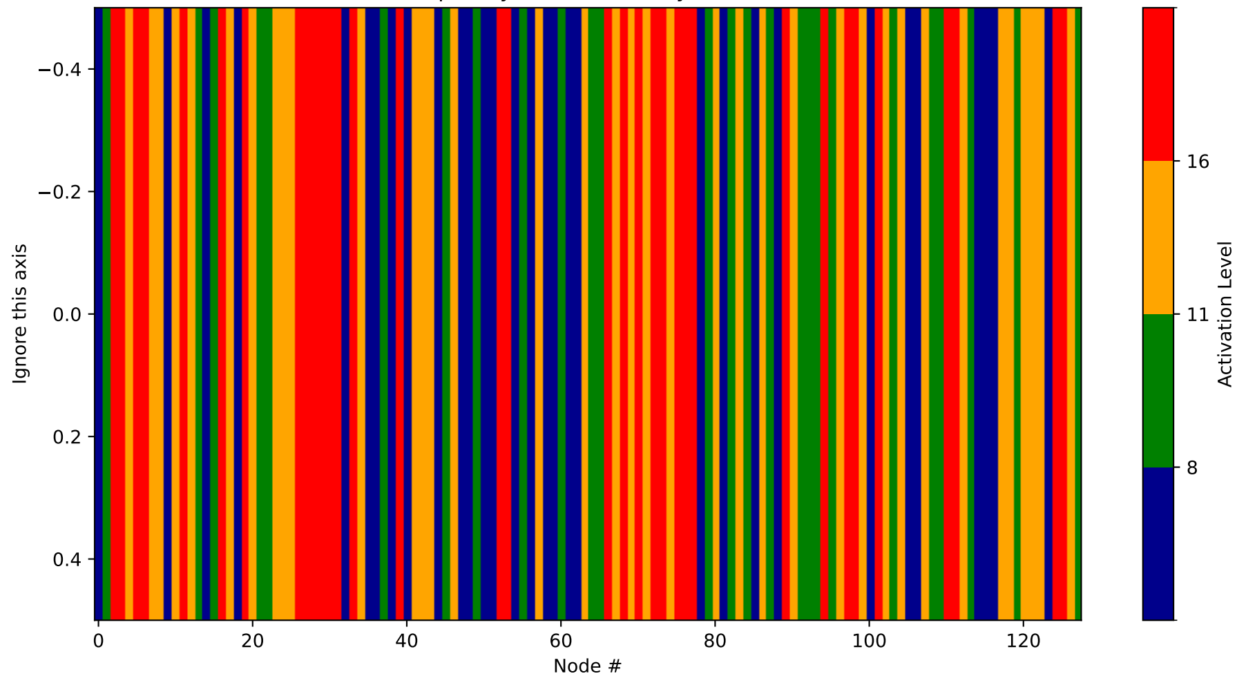
Heatmap - Layer 2 (Probability 3712-3840)
