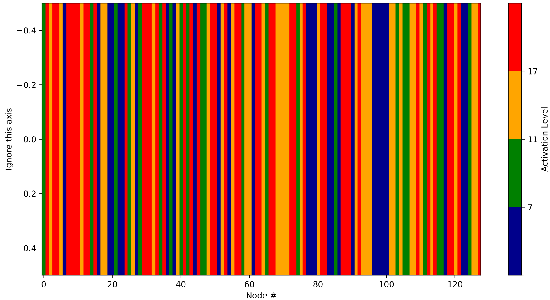
Heatmap - Layer 25 (Probability 2176-2304)
