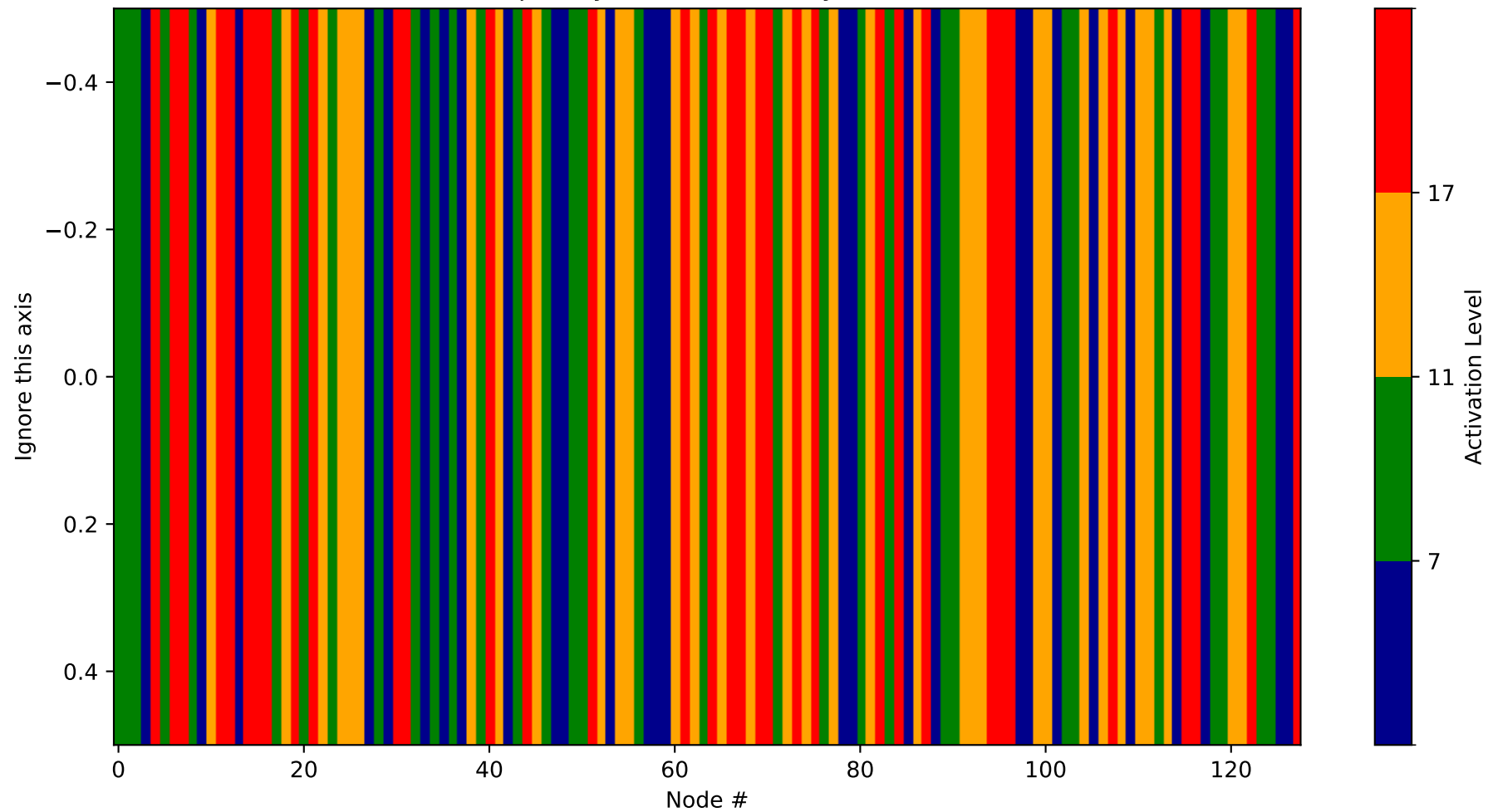
Heatmap - Layer 24 (Probability 1152-1280)
