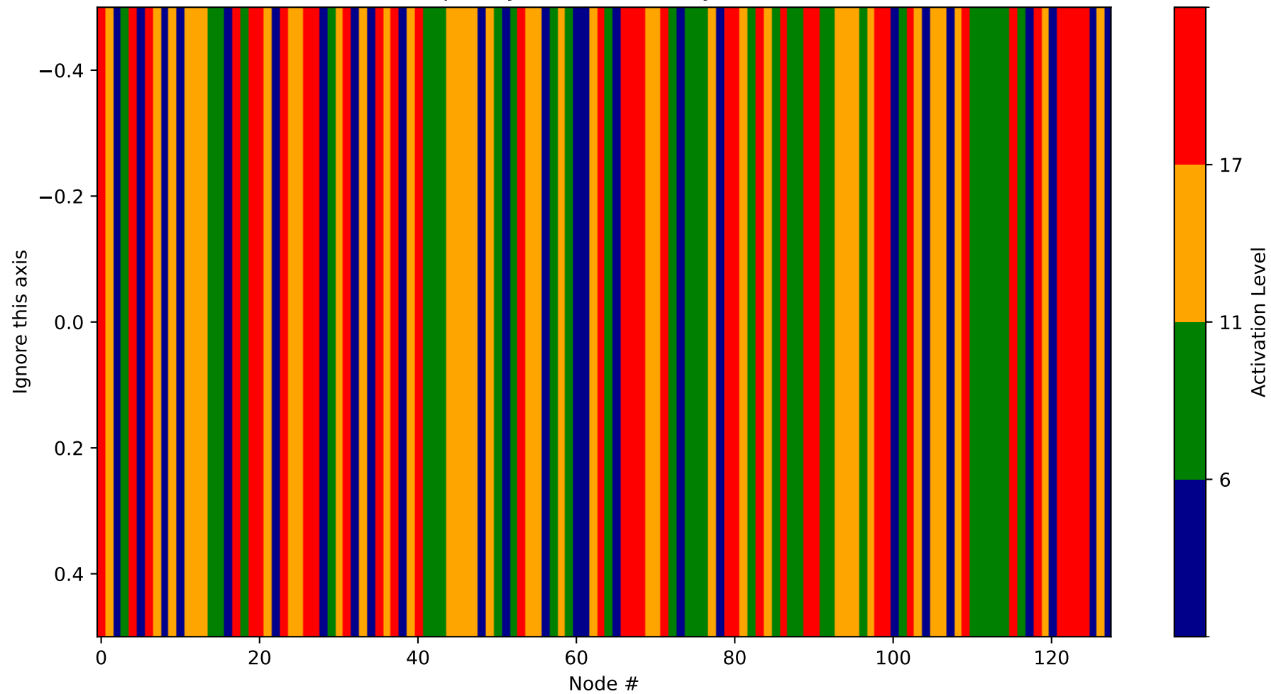
Heatmap - Layer 15 (Probability 1536-1664)
