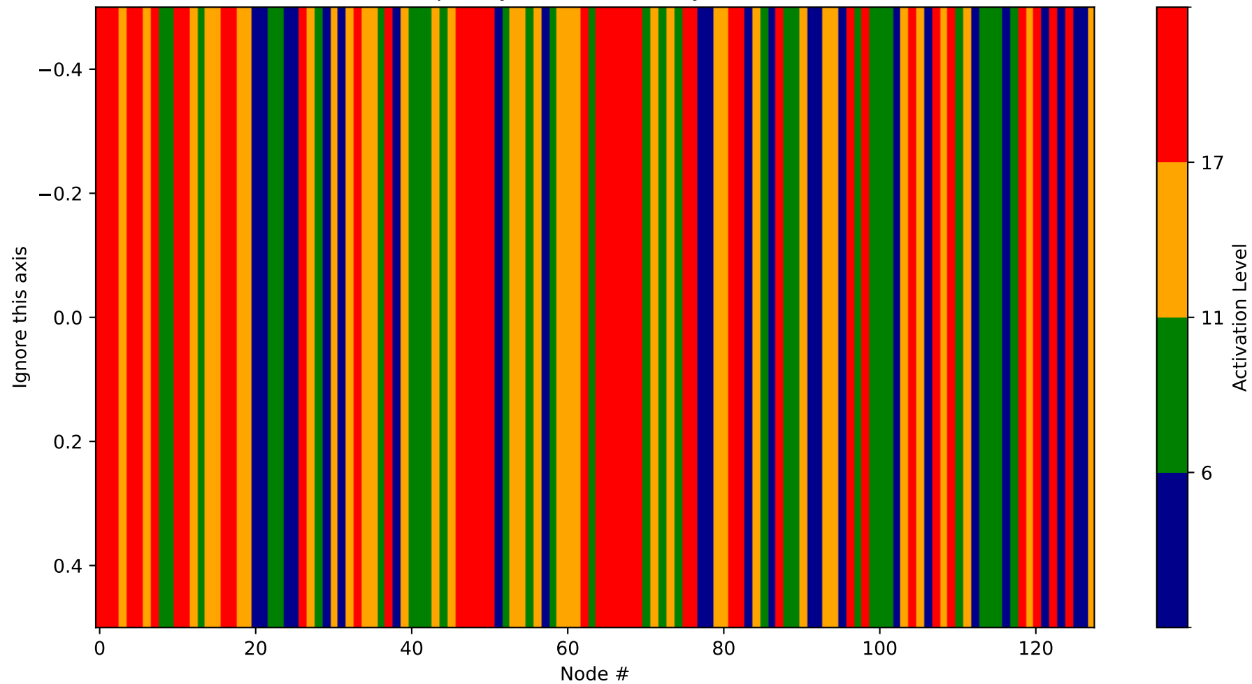
Heatmap - Layer 13 (Probability 3328-3456)
