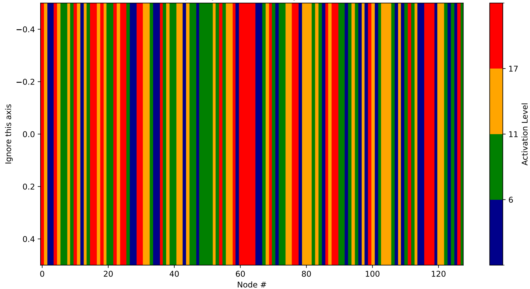
Heatmap - Layer 11 (Probability 3200-3328)
