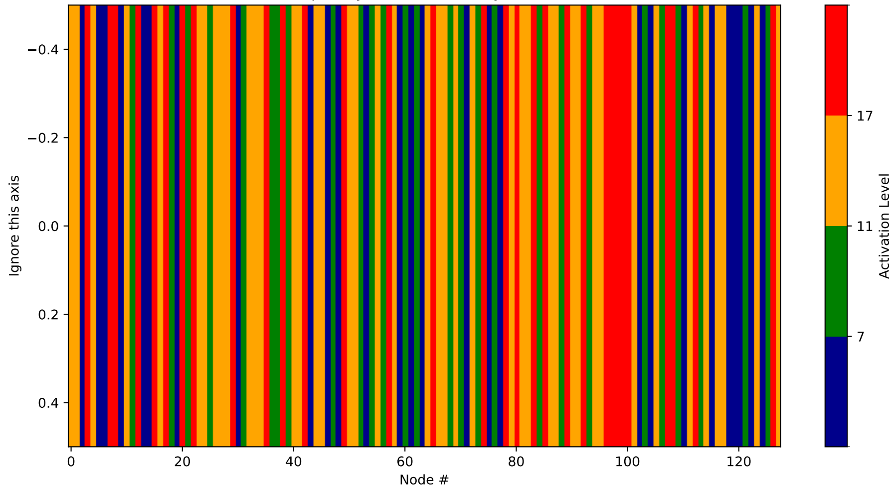
Heatmap - Layer 21 (Probability 1024-1152)
