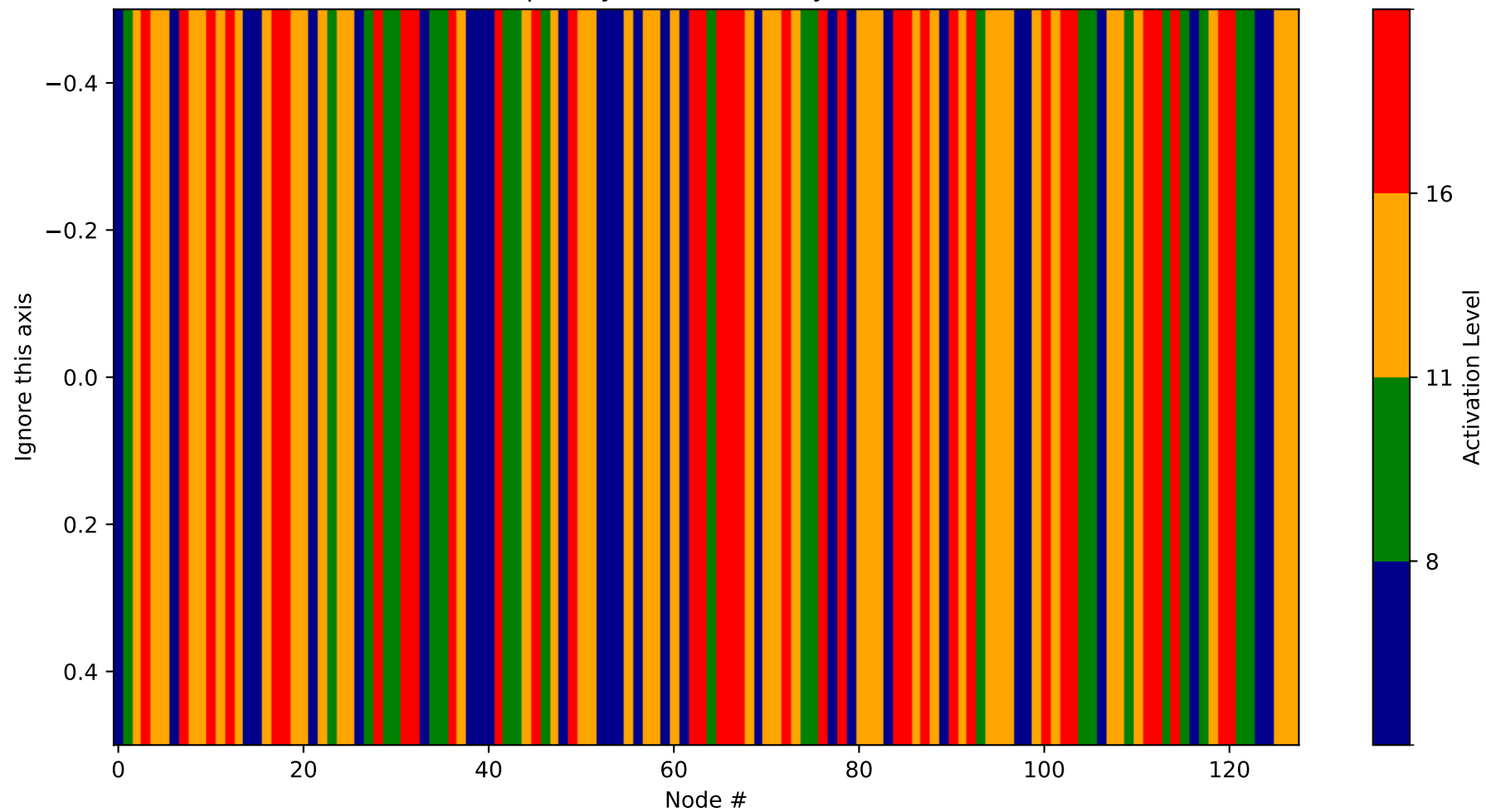
Heatmap - Layer 3 (Probability 1920-2048)
