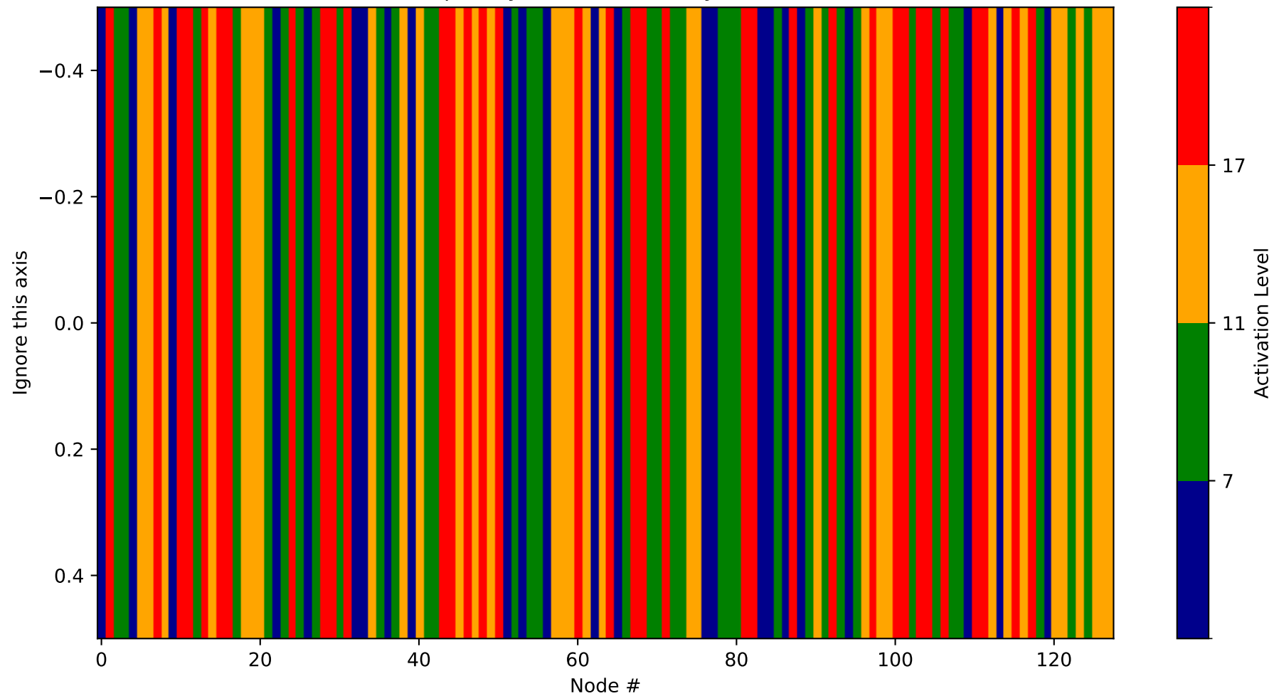
Heatmap - Layer 28 (Probability 3072-3200)
