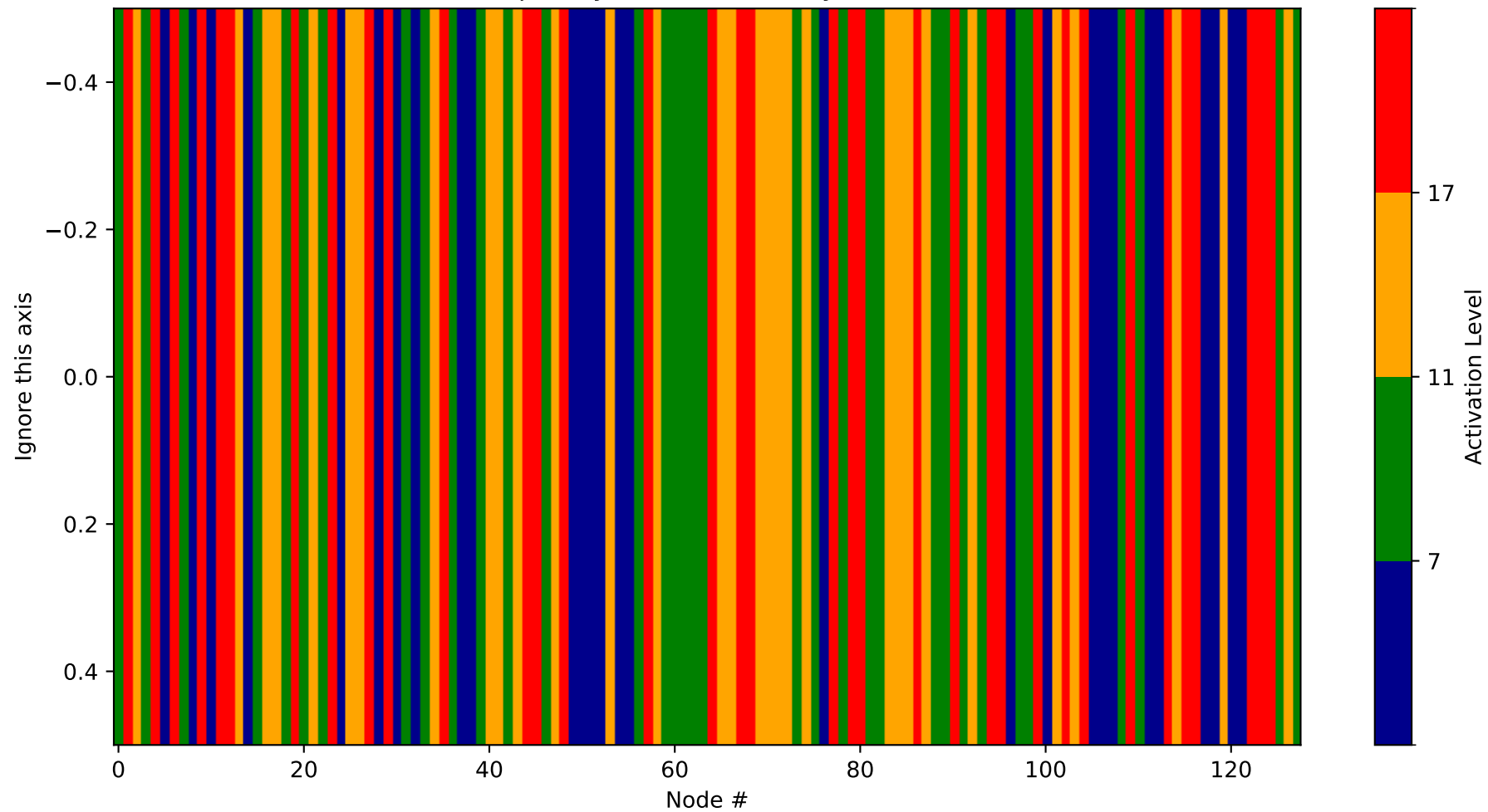
Heatmap - Layer 22 (Probability 1536-1664)
