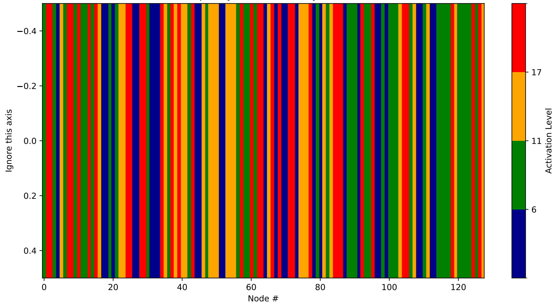
Heatmap - Layer 29 (Probability 512-640)
