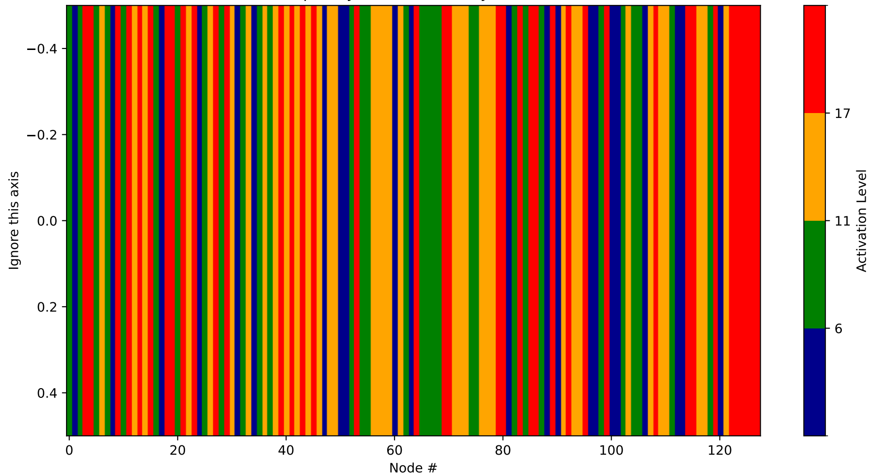
Heatmap - Layer 30 (Probability 1536-1664)
