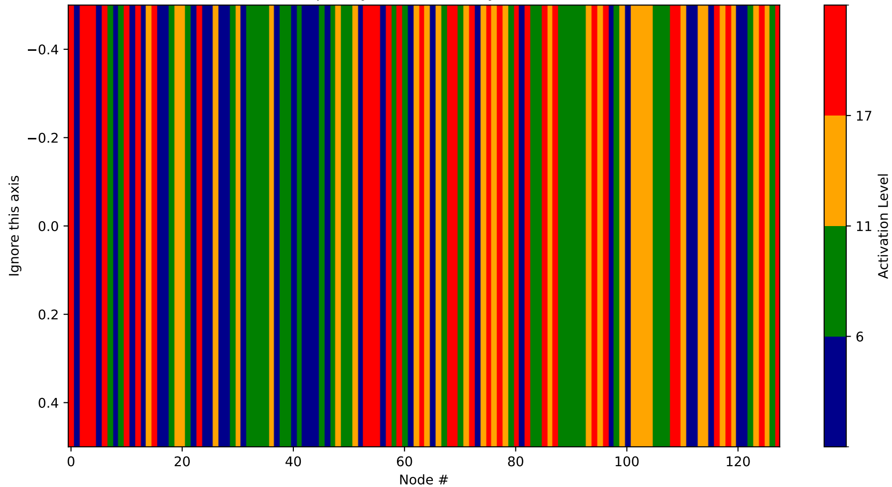
Heatmap - Layer 9 (Probability 3968-4096)
