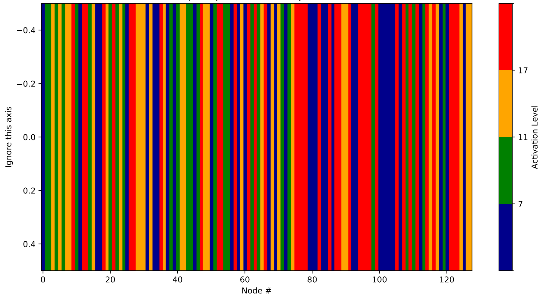
Heatmap - Layer 28 (Probability 3968-4096)
