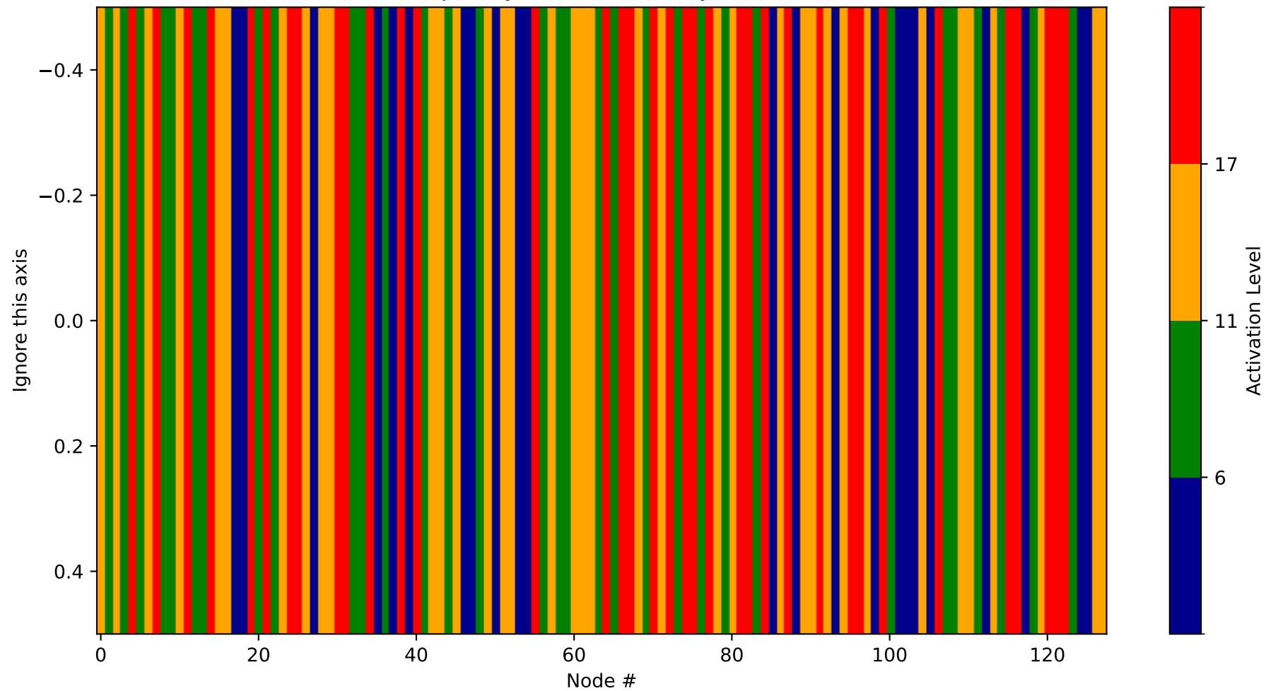
Heatmap - Layer 18 (Probability 1152-1280)
