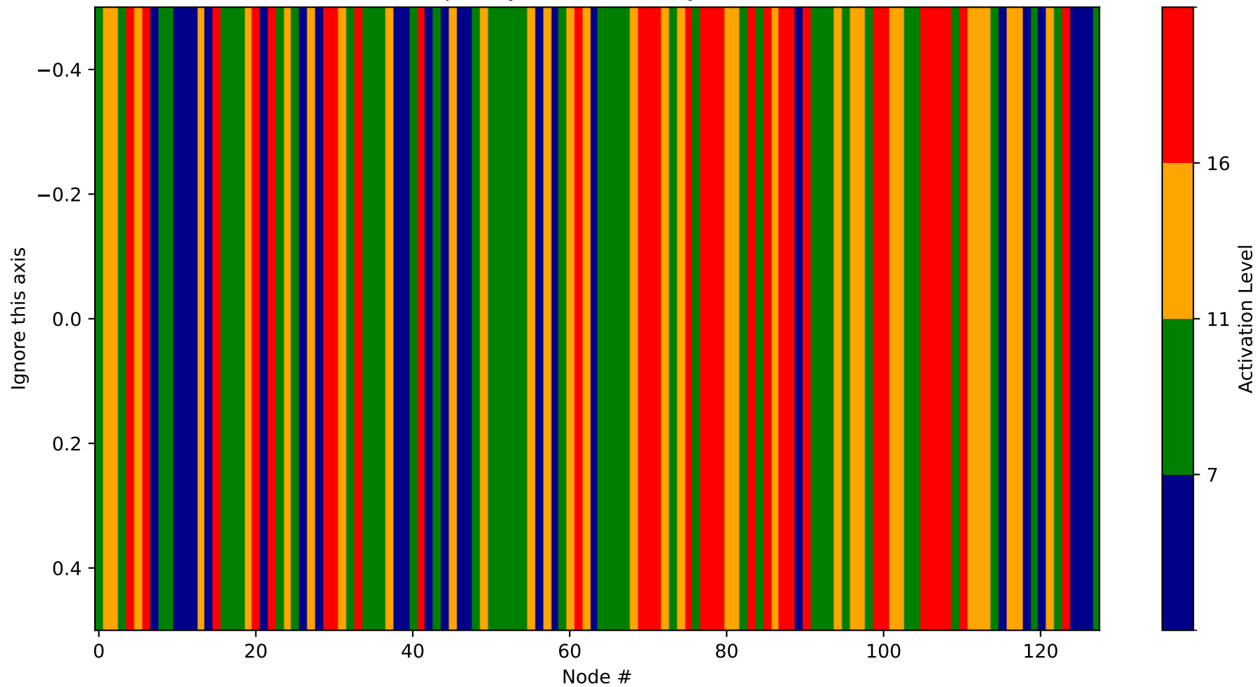
Heatmap - Layer 4 (Probability 3840-3968)
