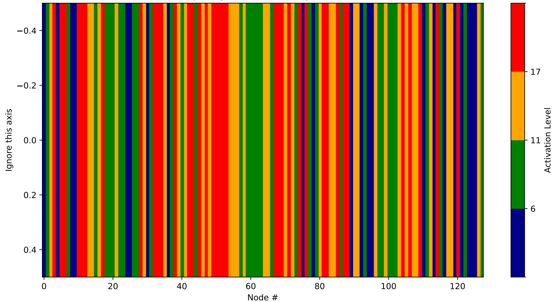
Heatmap - Layer 18 (Probability 3328-3456)
