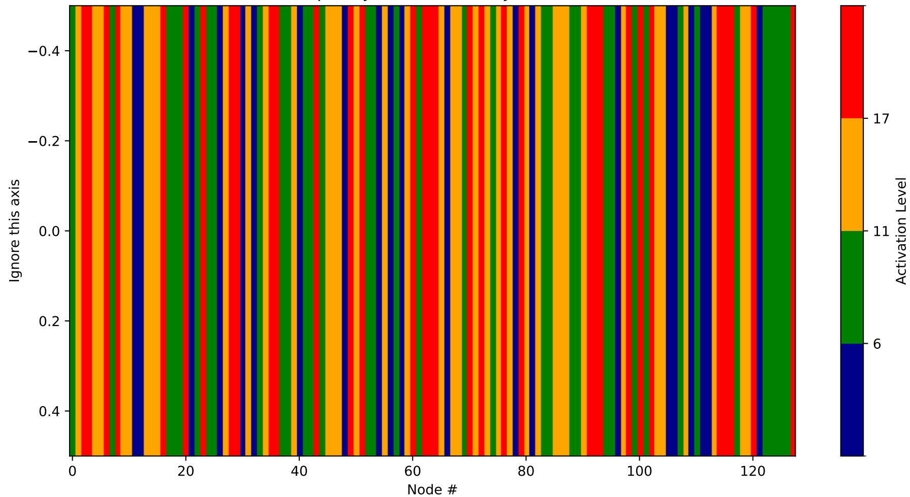
Heatmap - Layer 11 (Probability 2816-2944)
