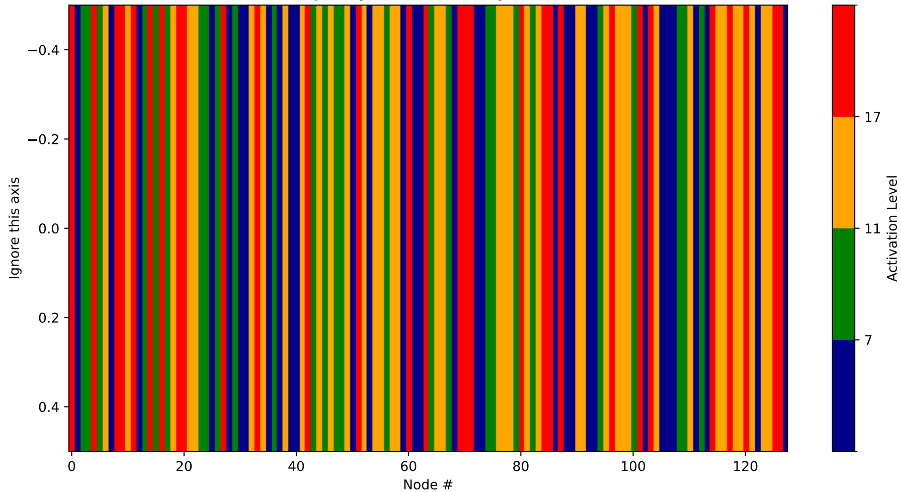
Heatmap - Layer 24 (Probability 1920-2048)
