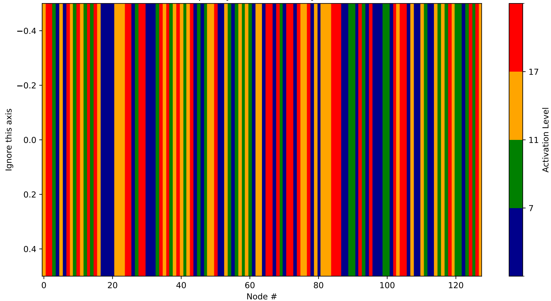
Heatmap - Layer 28 (Probability 512-640)
