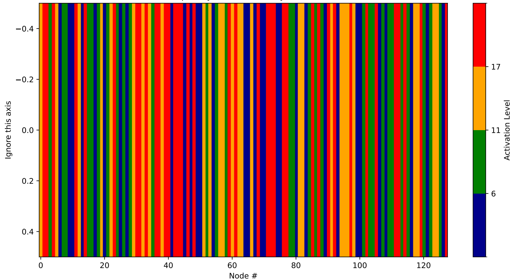
Heatmap - Layer 8 (Probability 2304-2432)
