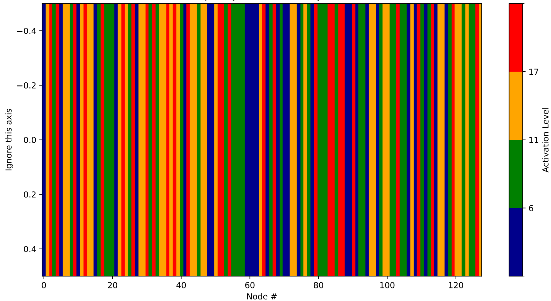
Heatmap - Layer 29 (Probability 0-128)
