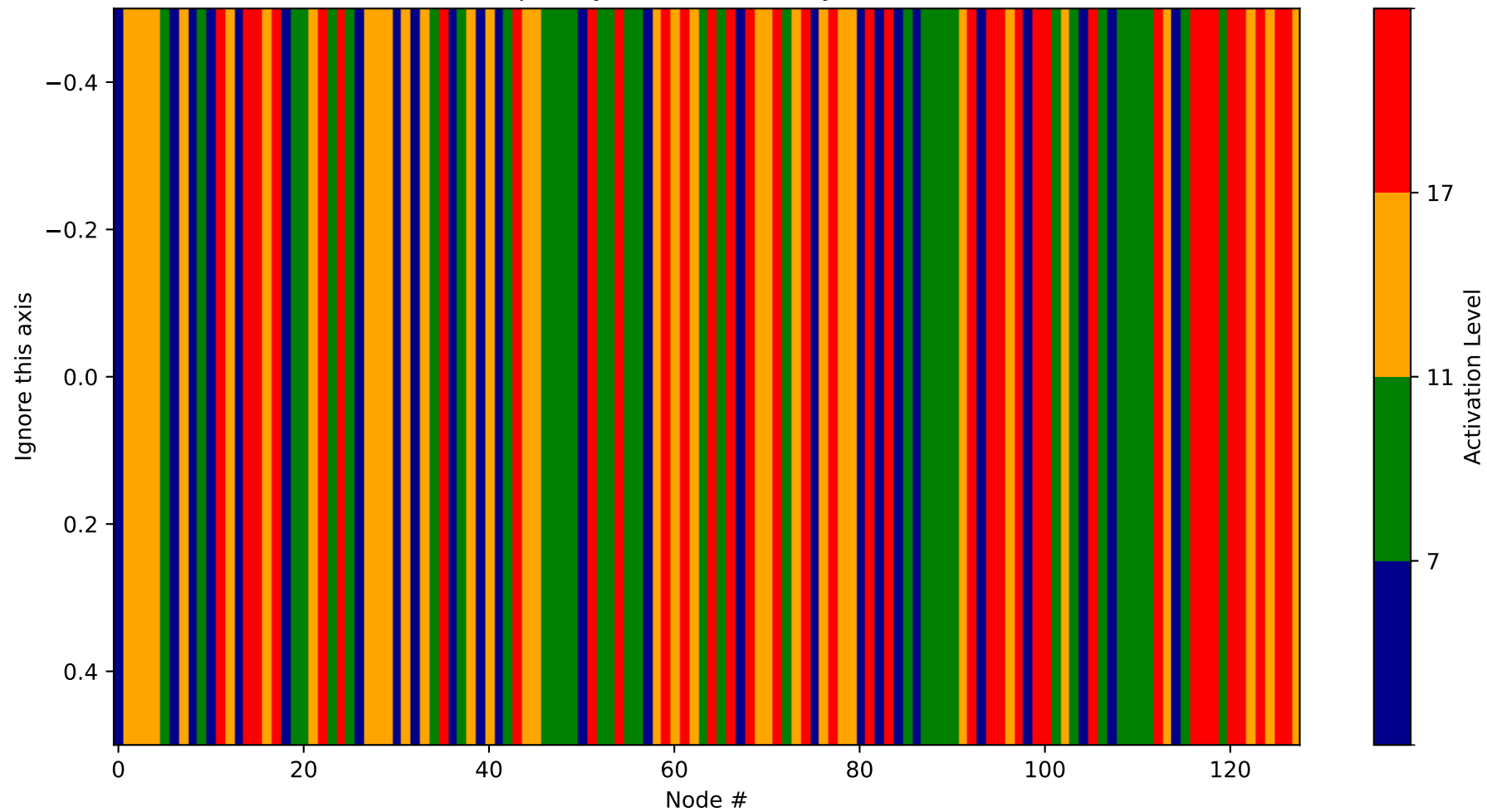
Heatmap - Layer 25 (Probability 1408-1536)
