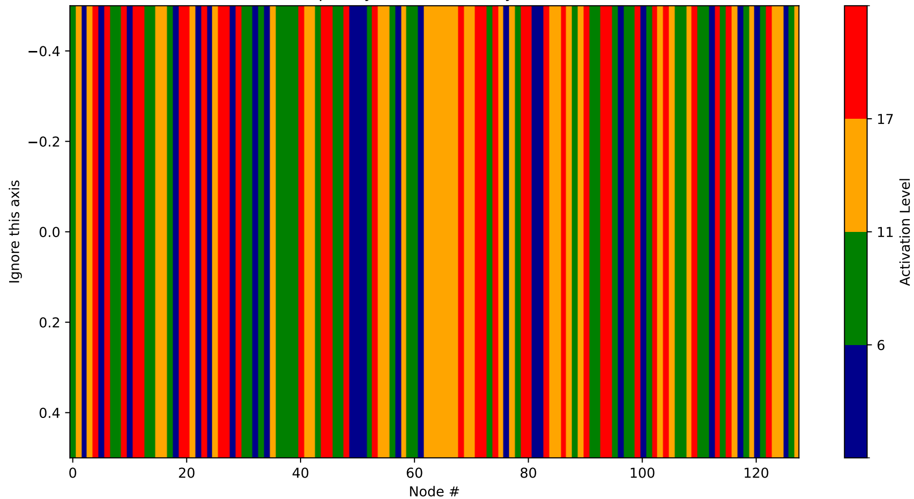
Heatmap - Layer 18 (Probability 1536-1664)
