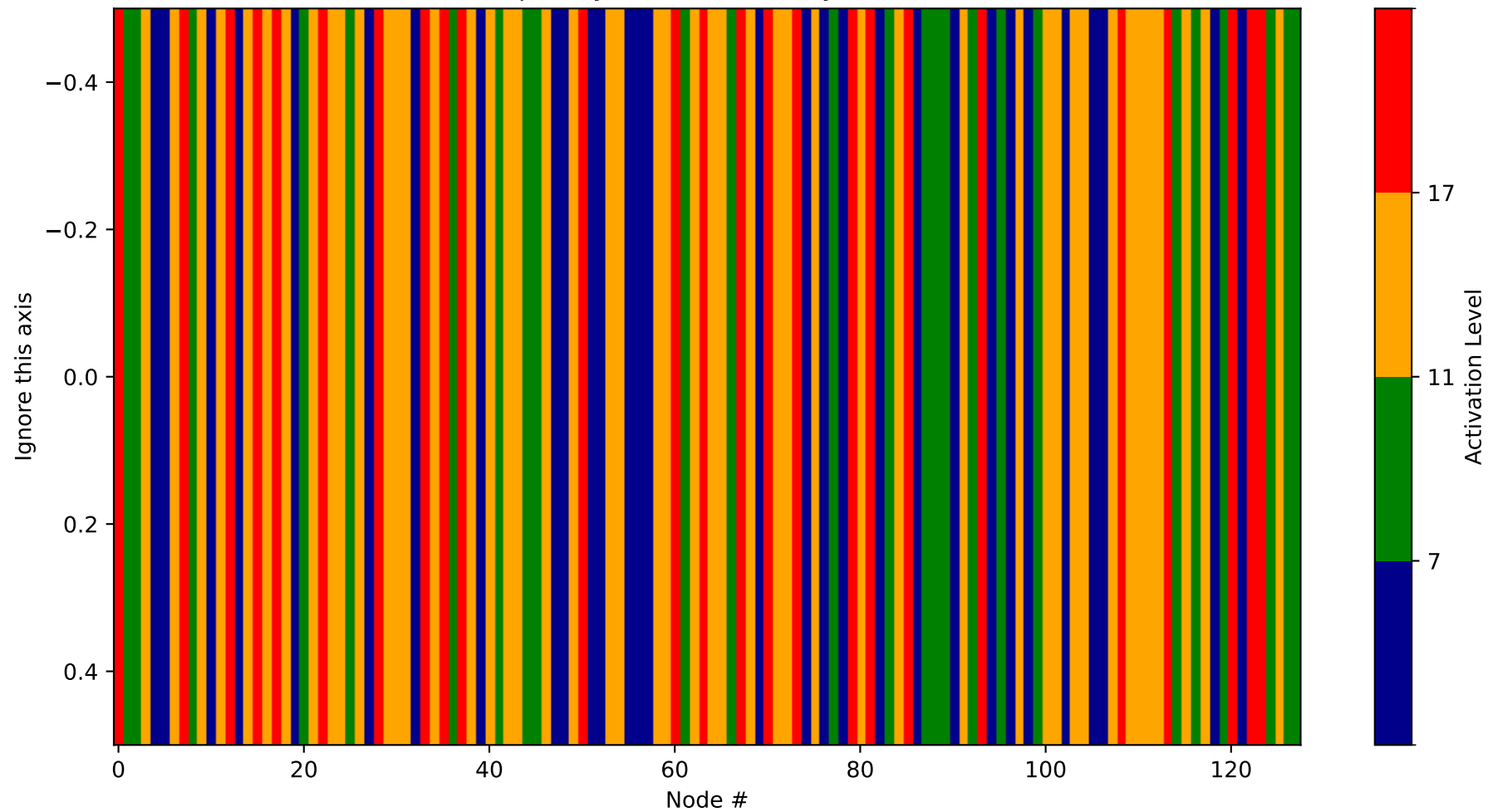
Heatmap - Layer 28 (Probability 2560-2688)
