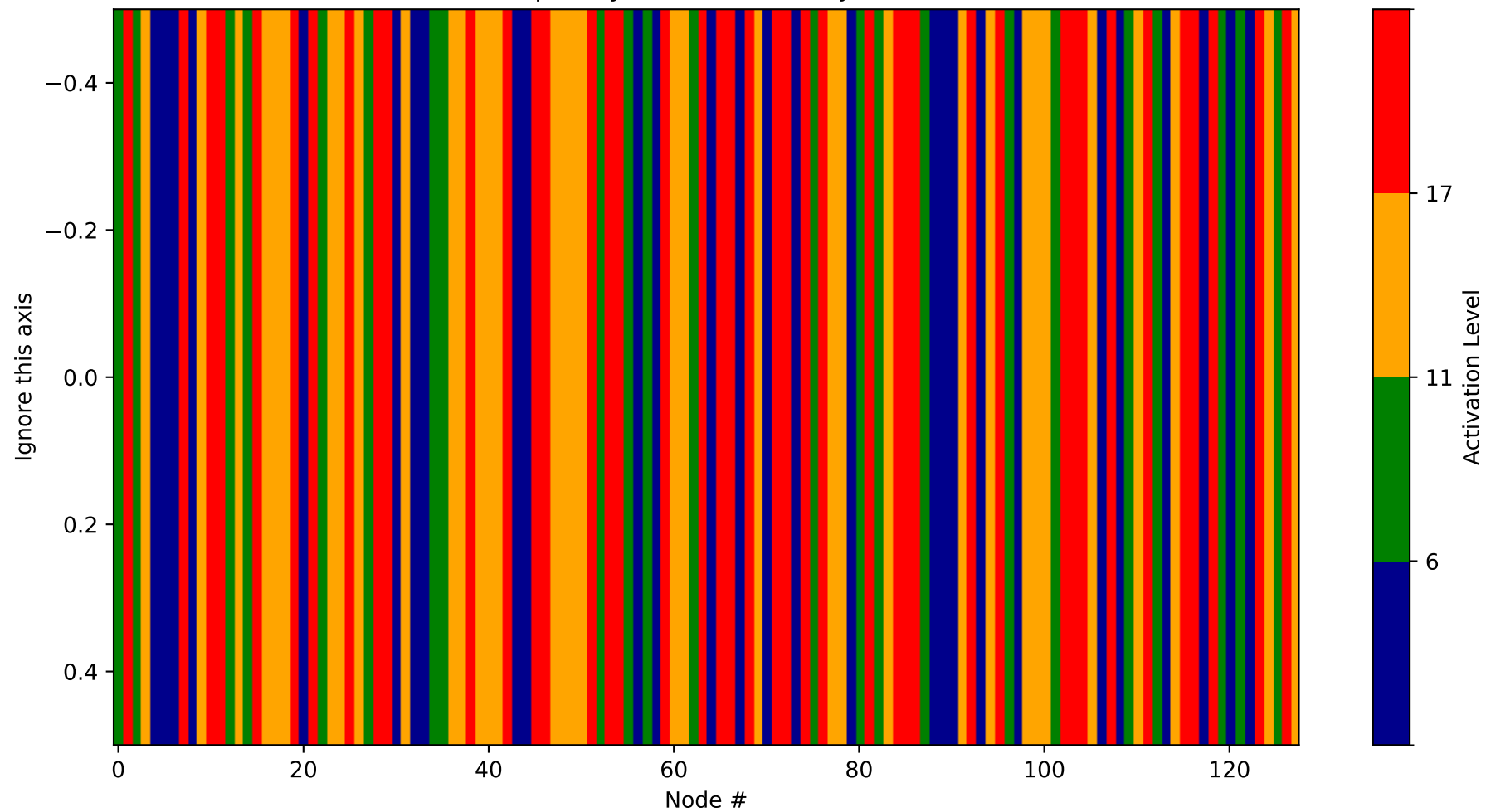
Heatmap - Layer 18 (Probability 512-640)
