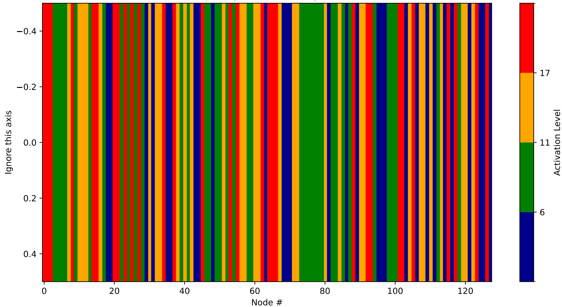
Heatmap - Layer 7 (Probability 768-896)
