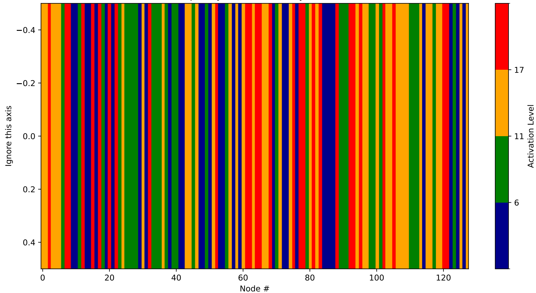
Heatmap - Layer 16 (Probability 896-1024)
