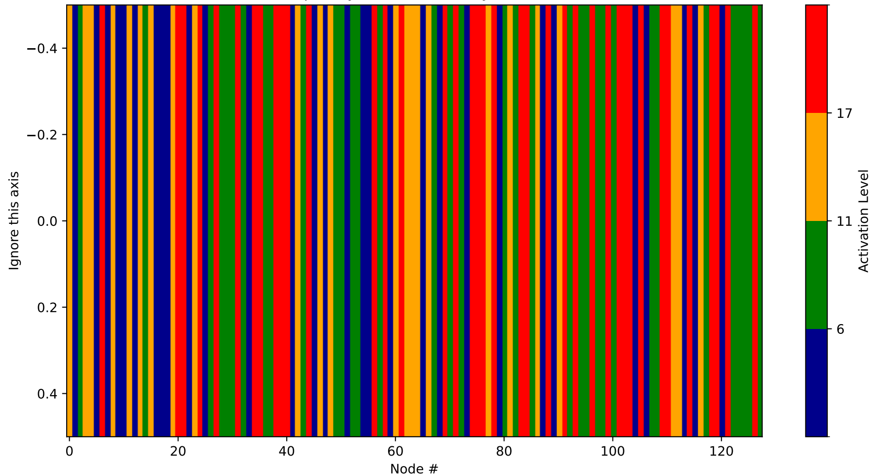
Heatmap - Layer 17 (Probability 3840-3968)
