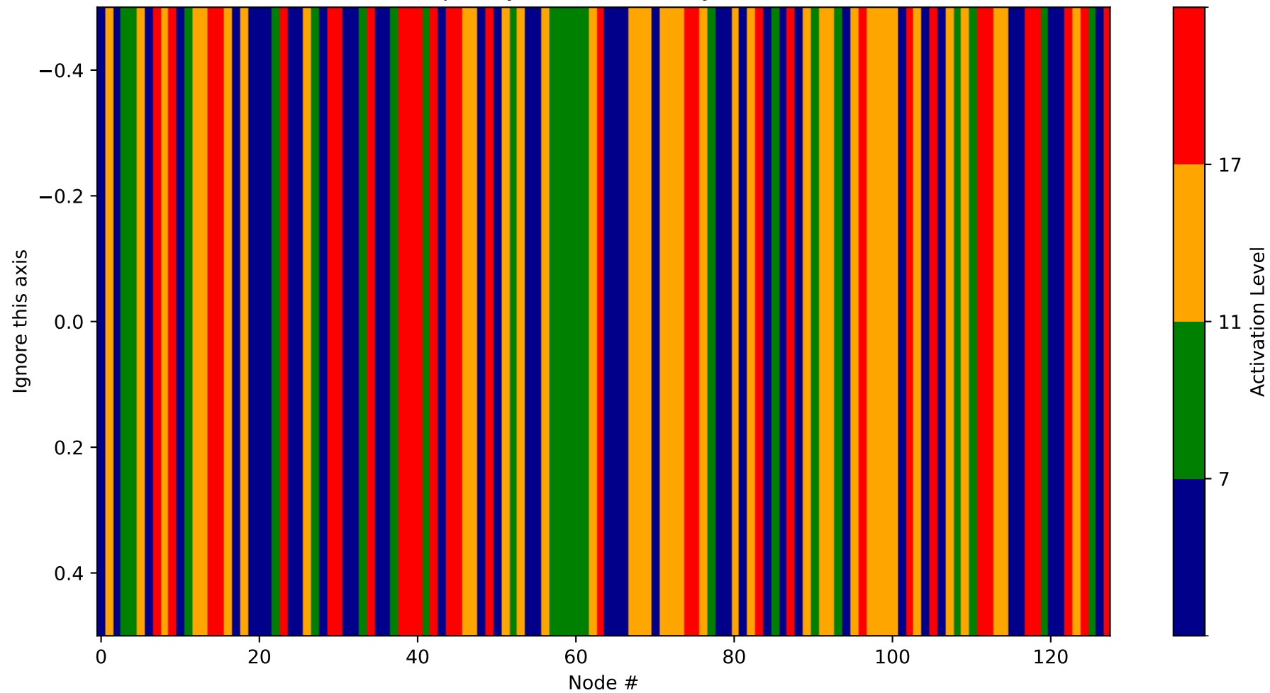
Heatmap - Layer 23 (Probability 2304-2432)
