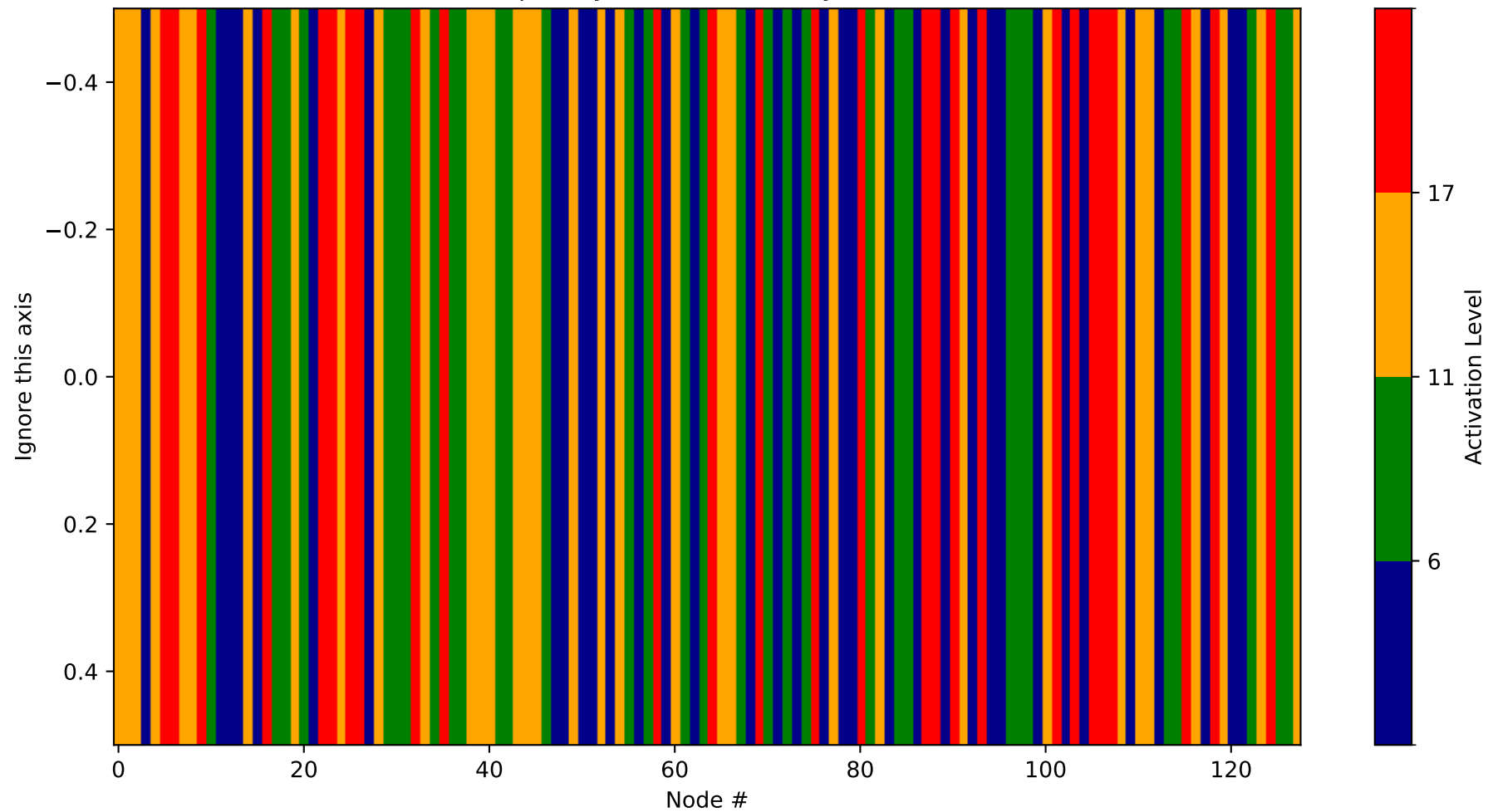
Heatmap - Layer 19 (Probability 1280-1408)
