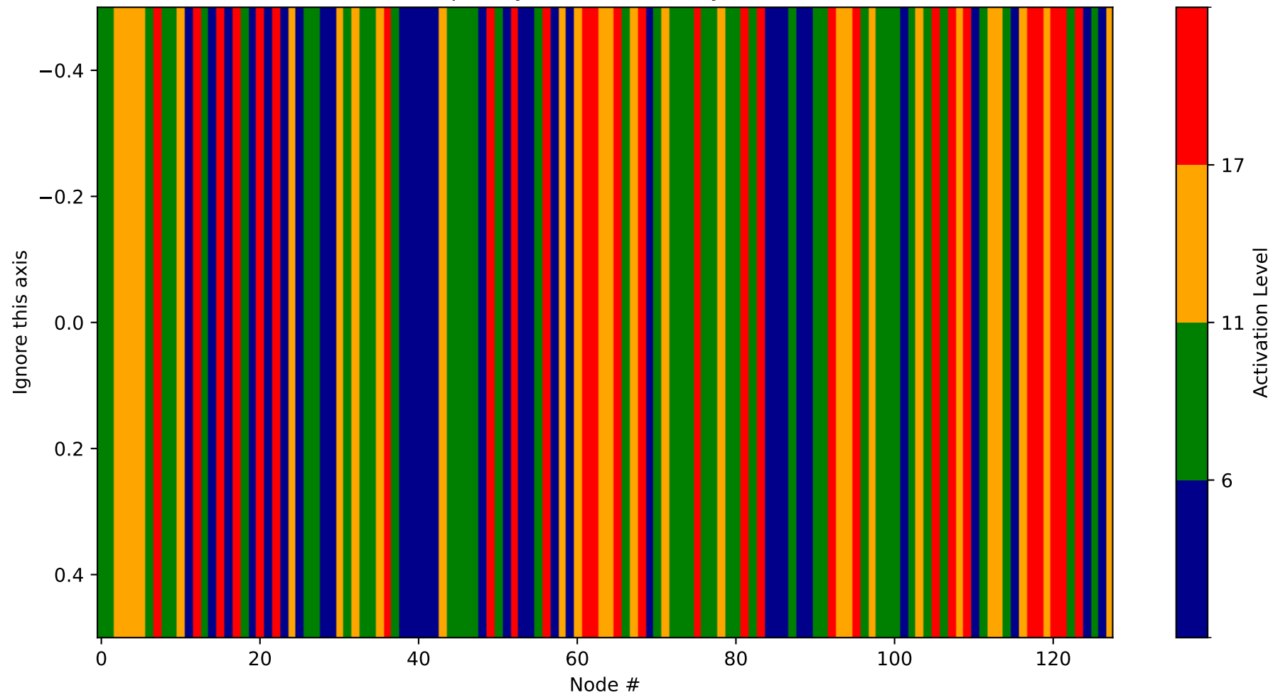
Heatmap - Layer 15 (Probability 896-1024)
