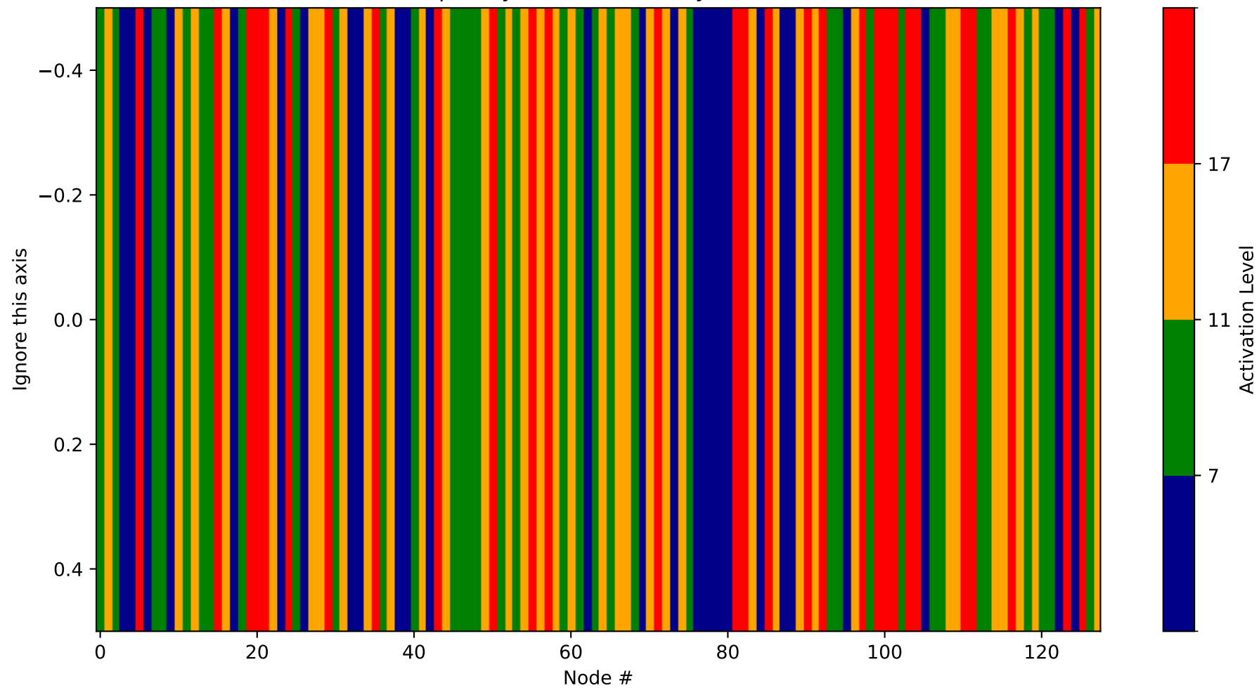
Heatmap - Layer 21 (Probability 3072-3200)
