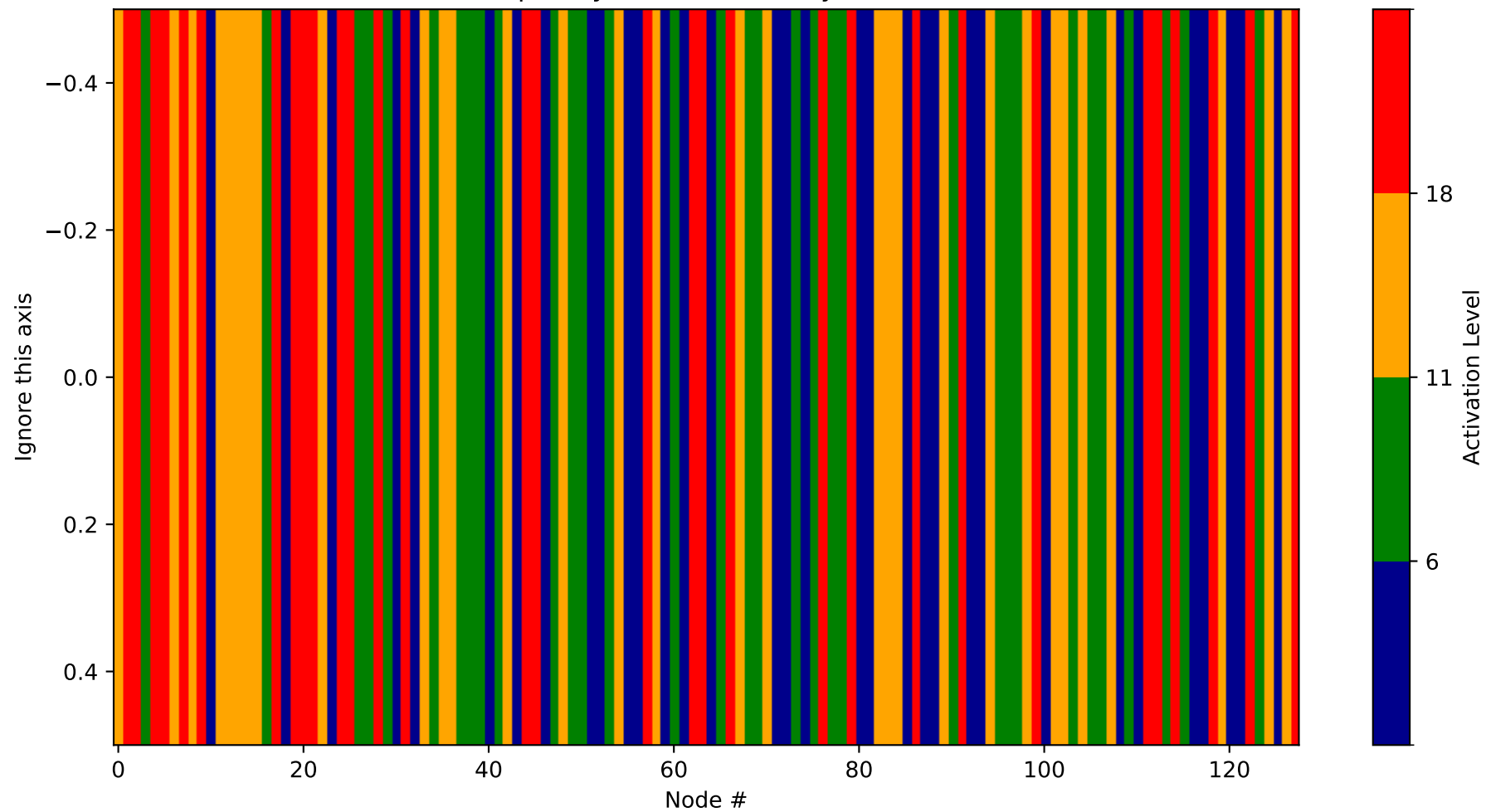
Heatmap - Layer 12 (Probability 3584-3712)
