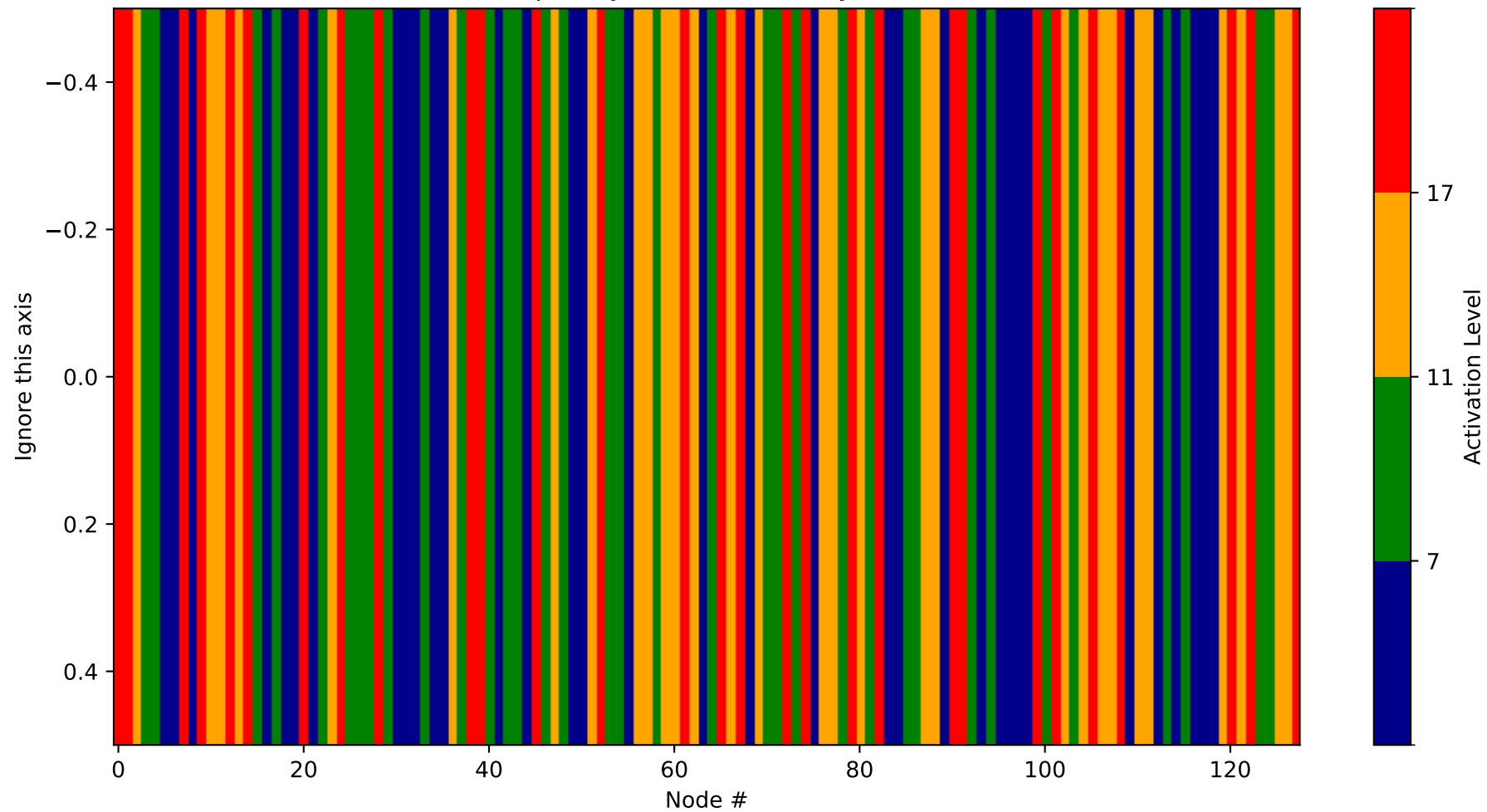
Heatmap - Layer 21 (Probability 768-896)
