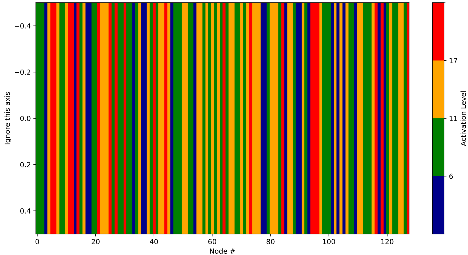
Heatmap - Layer 30 (Probability 1152-1280)
