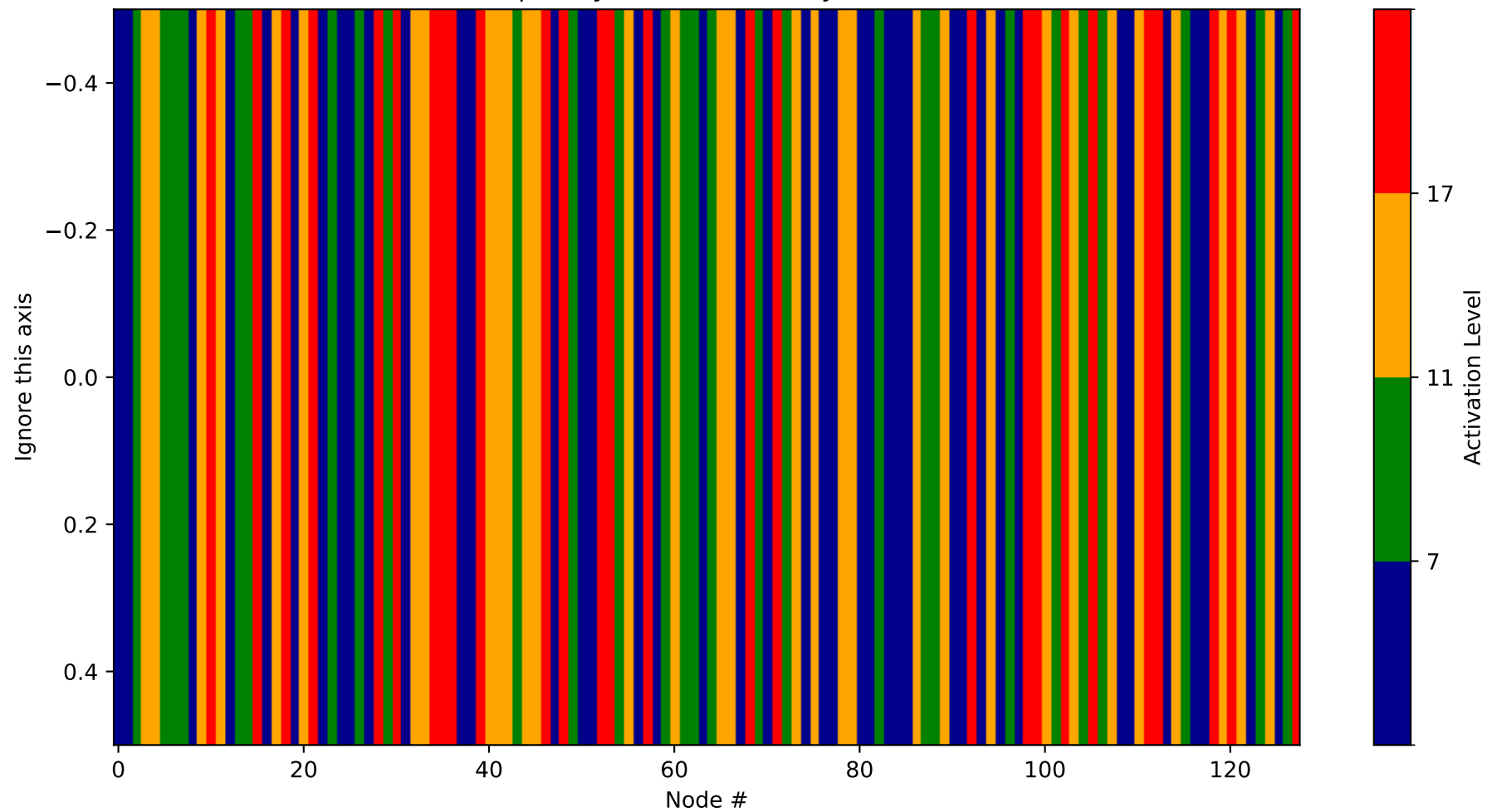
Heatmap - Layer 23 (Probability 2048-2176)
