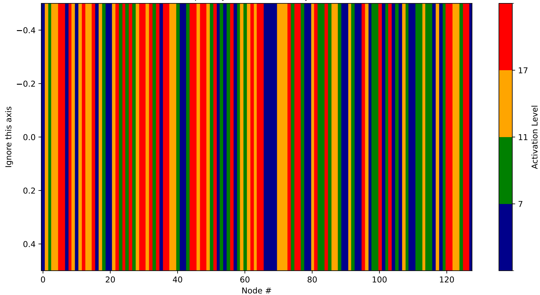
Heatmap - Layer 25 (Probability 128-256)
