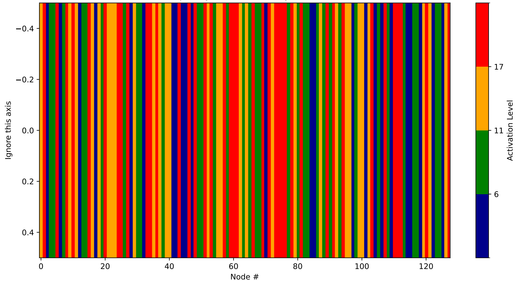
Heatmap - Layer 10 (Probability 2048-2176)
