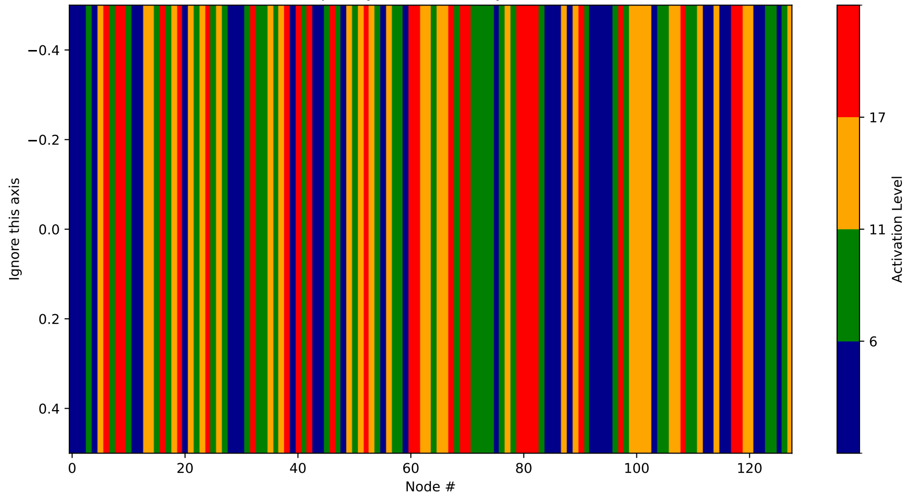
Heatmap - Layer 8 (Probability 1280-1408)
