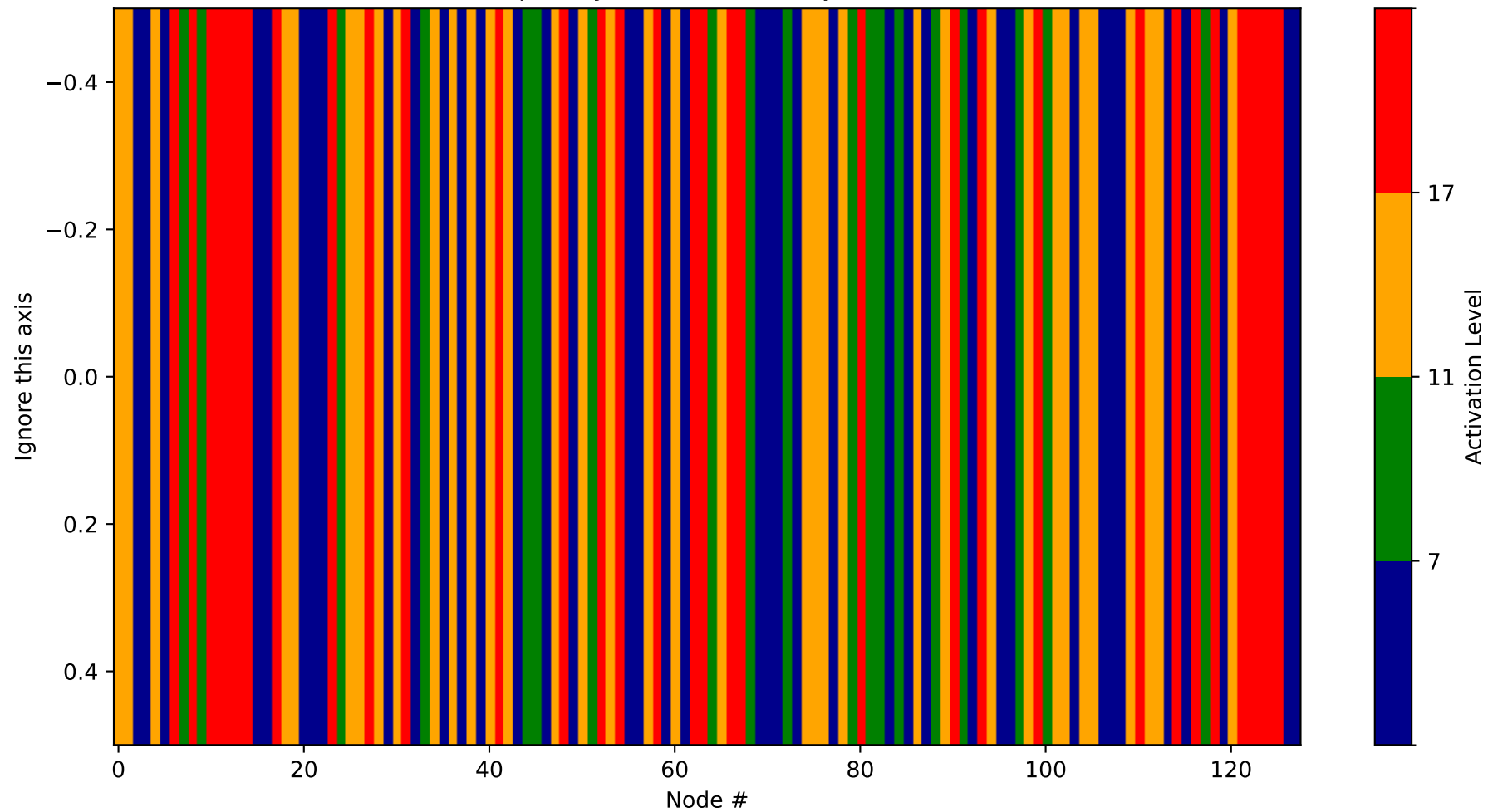
Heatmap - Layer 22 (Probability 1664-1792)
