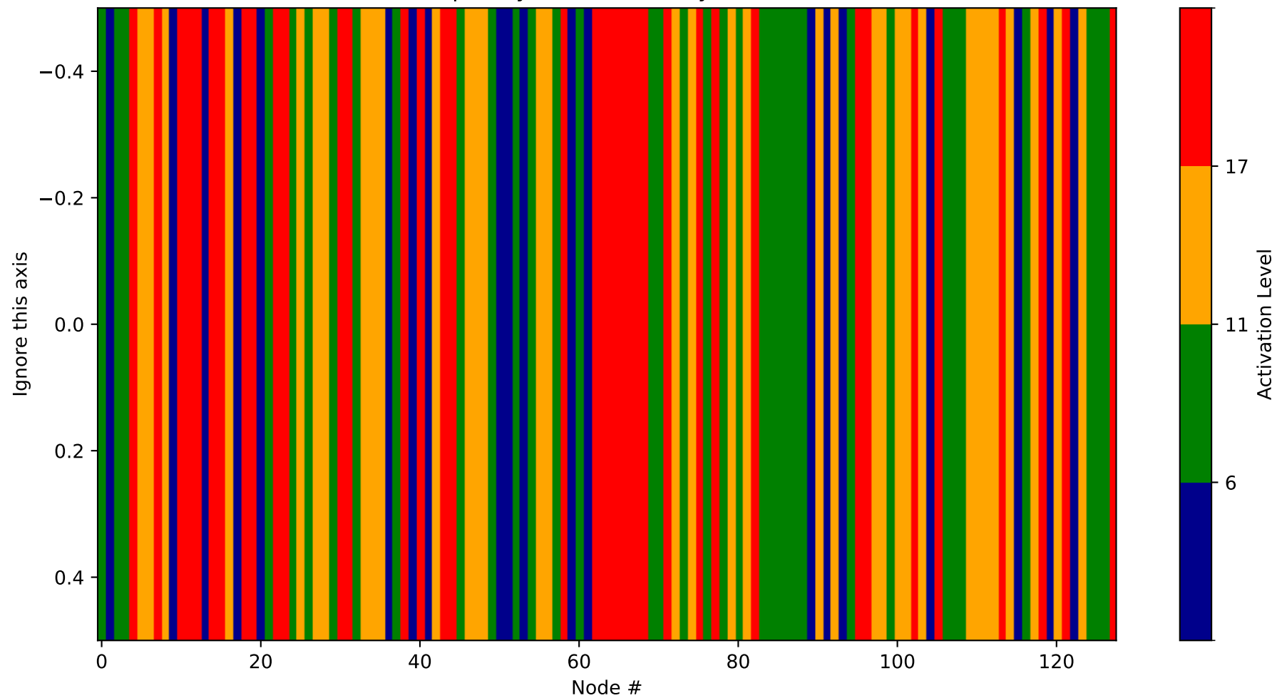
Heatmap - Layer 9 (Probability 1408-1536)
