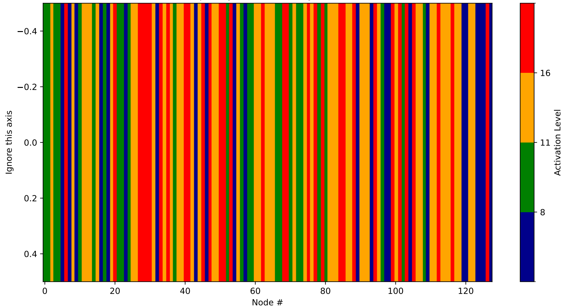
Heatmap - Layer 2 (Probability 3840-3968)
