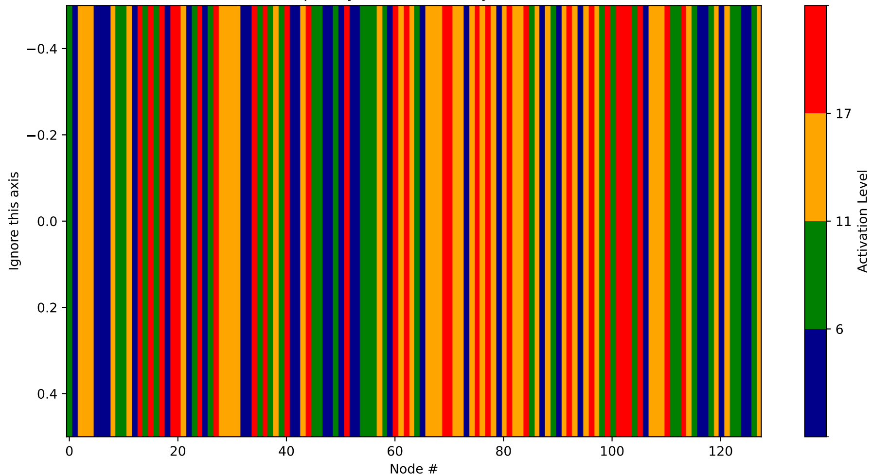
Heatmap - Layer 13 (Probability 3840-3968)
