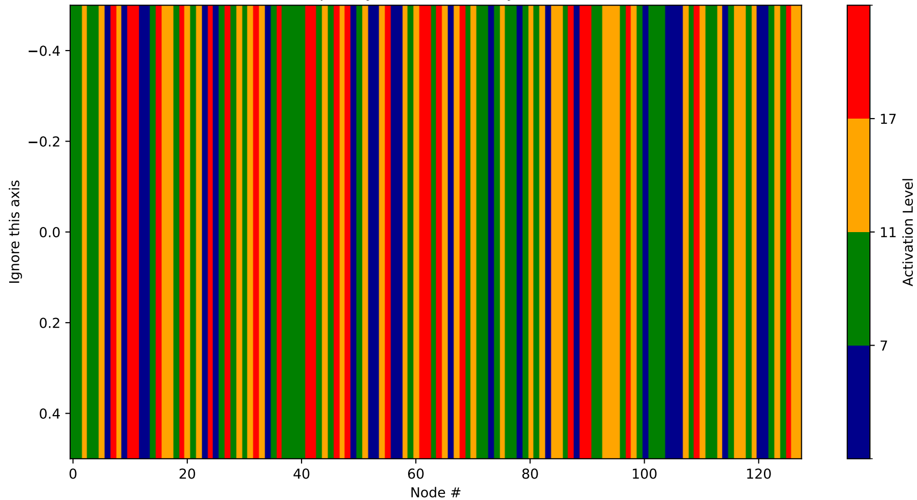
Heatmap - Layer 26 (Probability 3200-3328)
