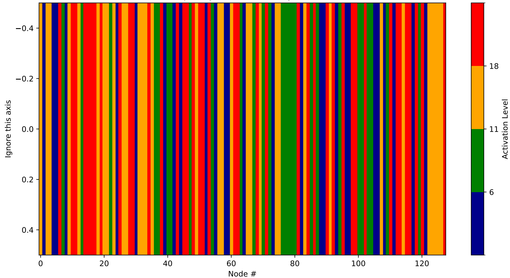
Heatmap - Layer 12 (Probability 512-640)
