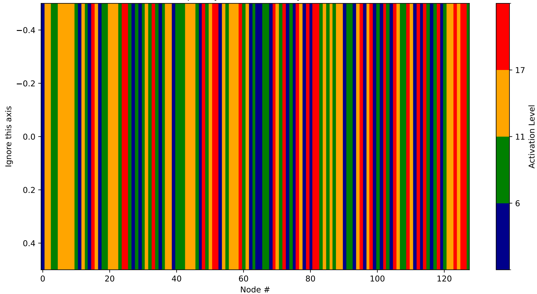
Heatmap - Layer 30 (Probability 2944-3072)
