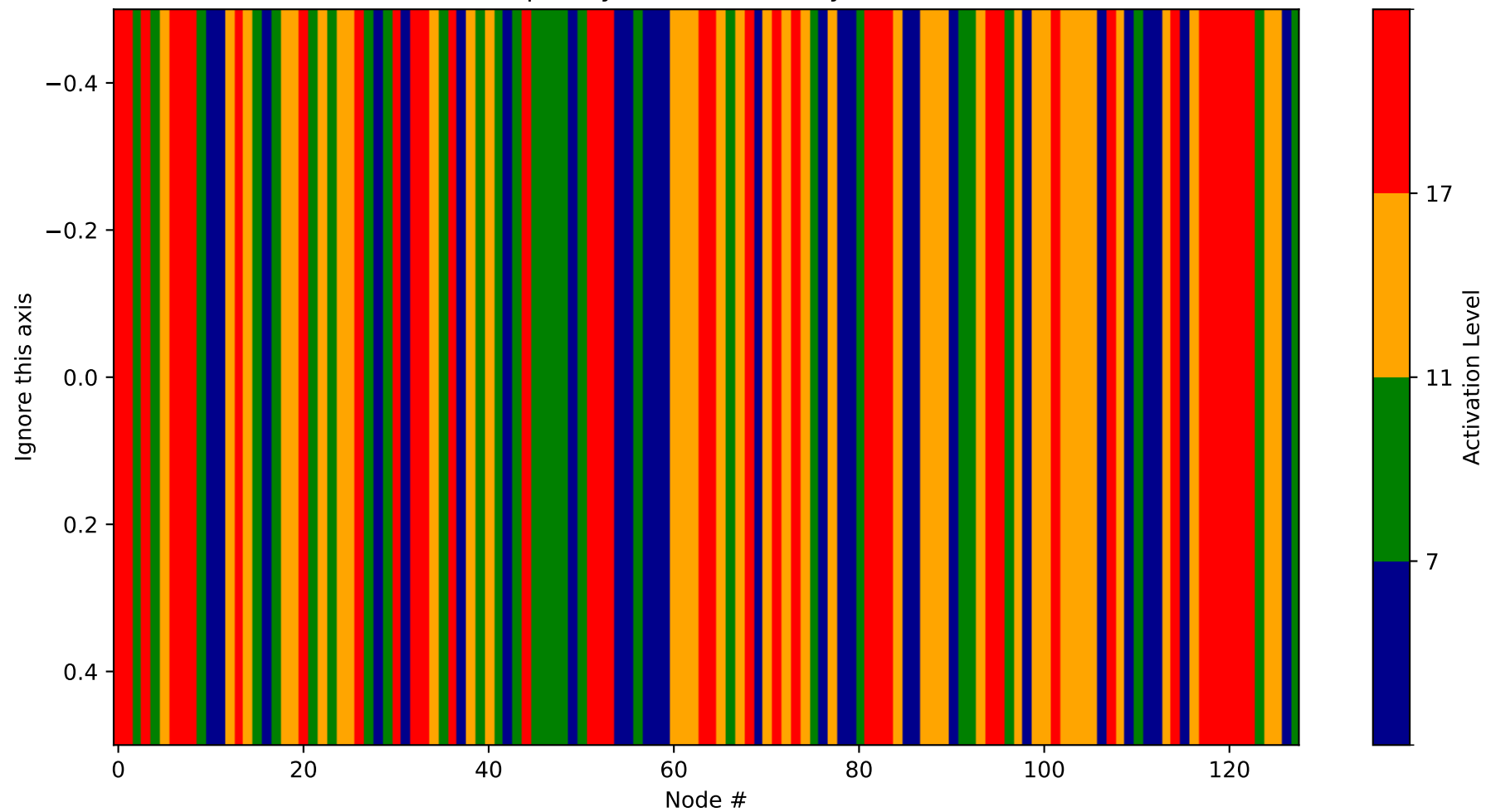
Heatmap - Layer 27 (Probability 896-1024)
