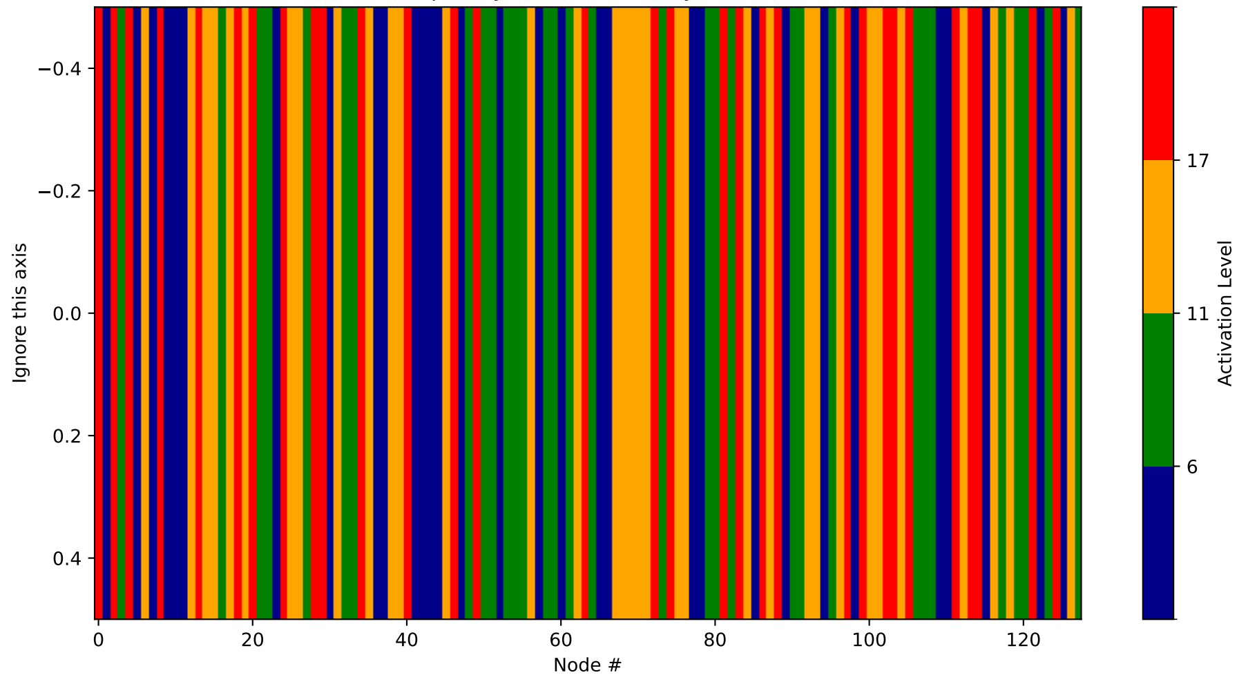
Heatmap - Layer 29 (Probability 3840-3968)
