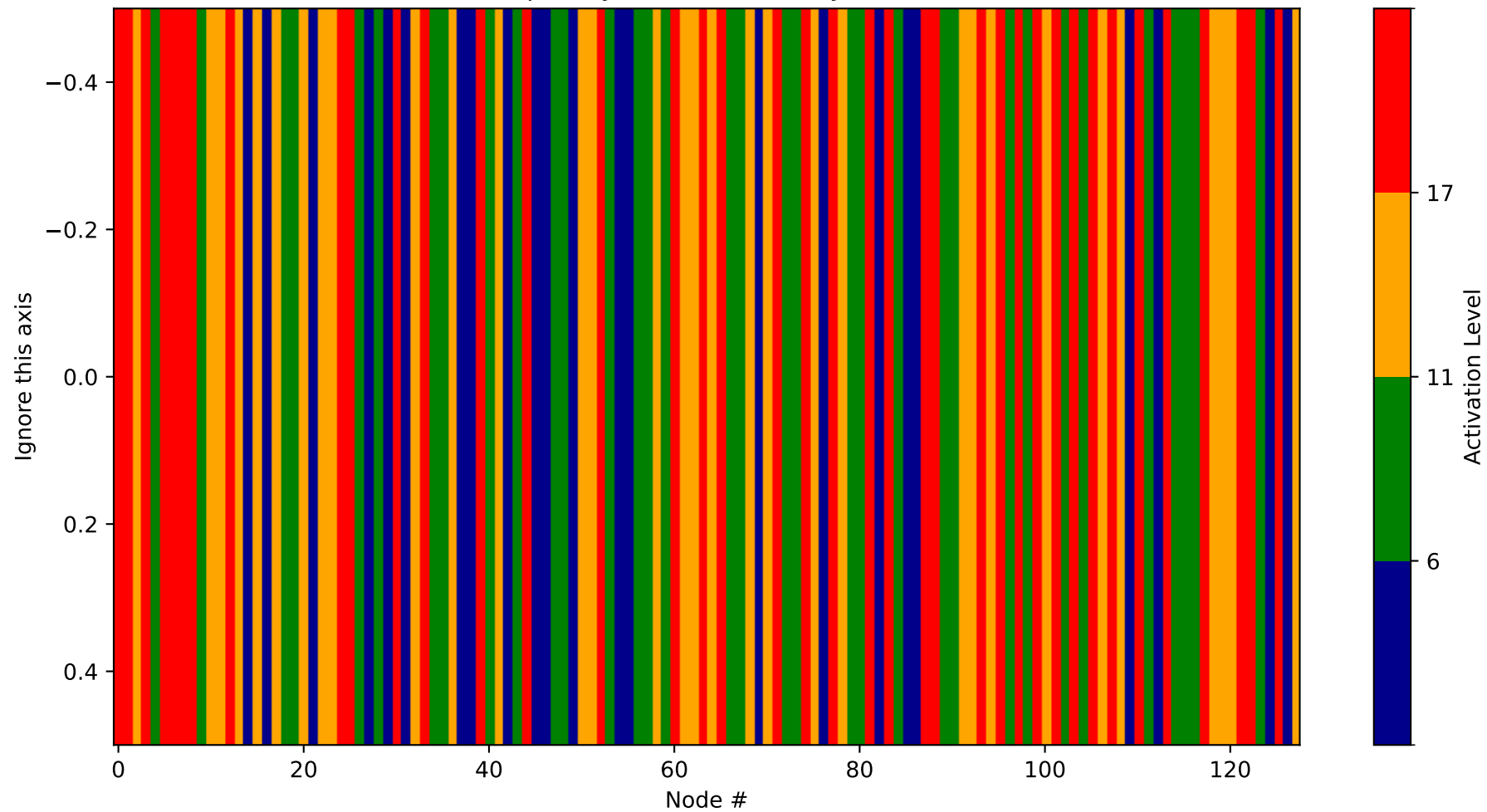
Heatmap - Layer 20 (Probability 896-1024)
