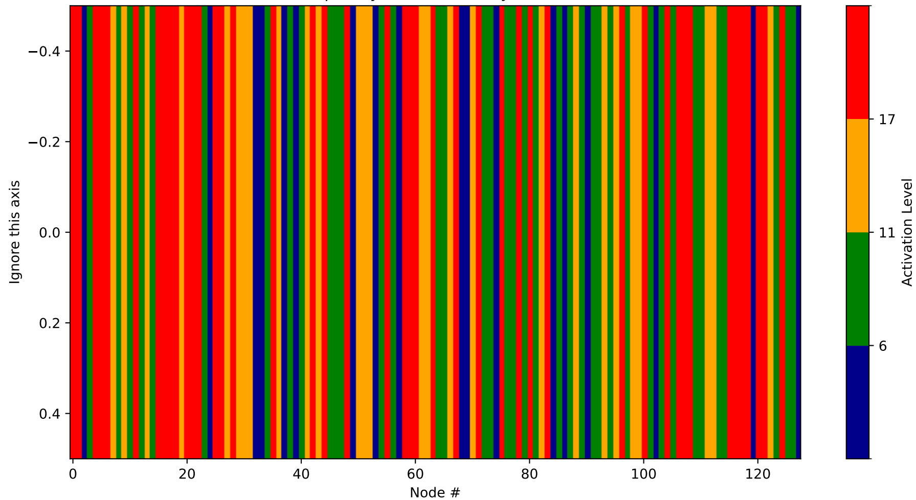
Heatmap - Layer 7 (Probability 2560-2688)
