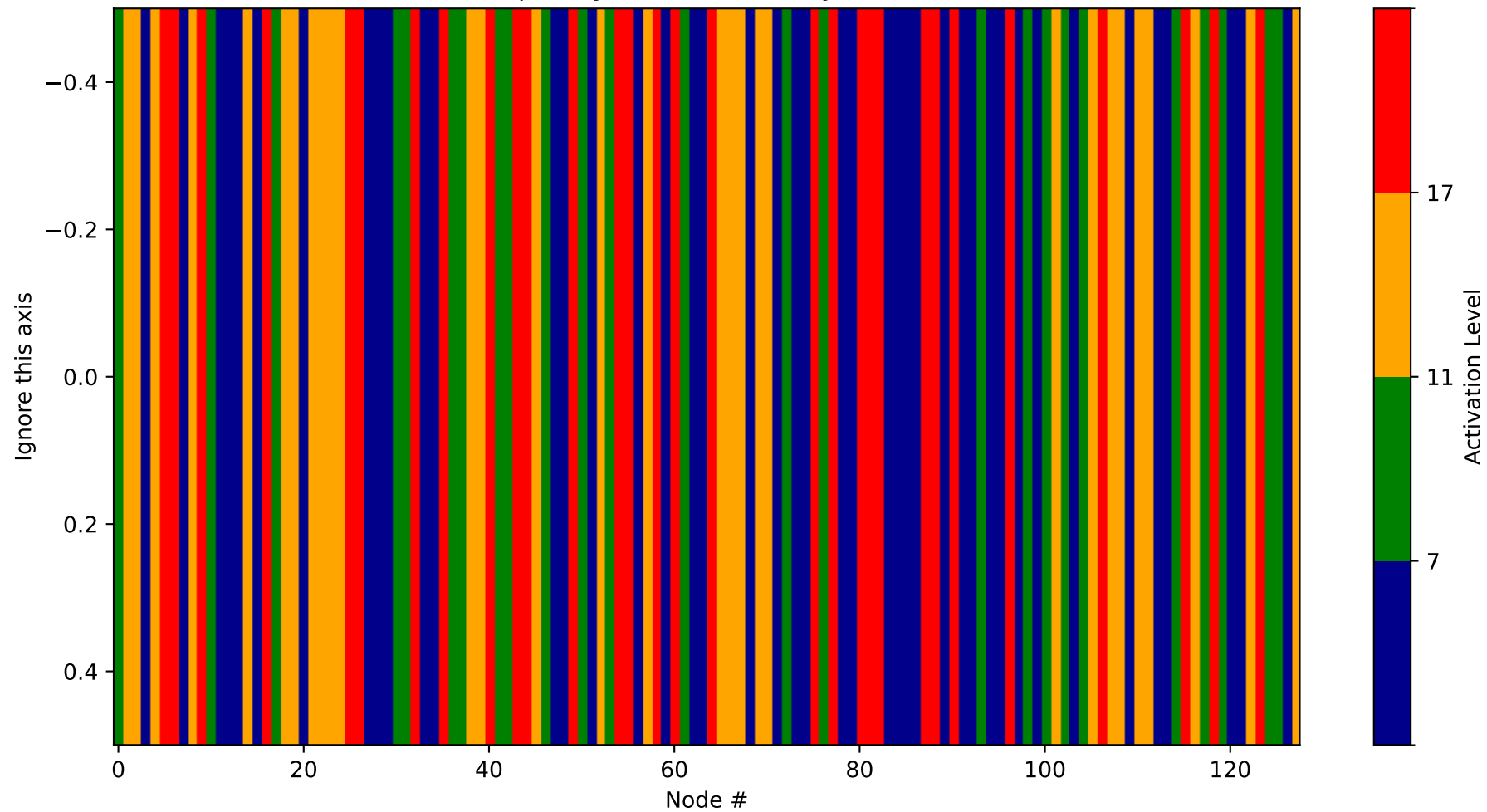
Heatmap - Layer 22 (Probability 1280-1408)
