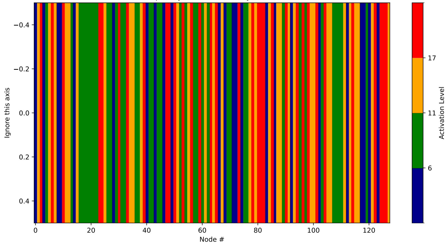
Heatmap - Layer 30 (Probability 3712-3840)
