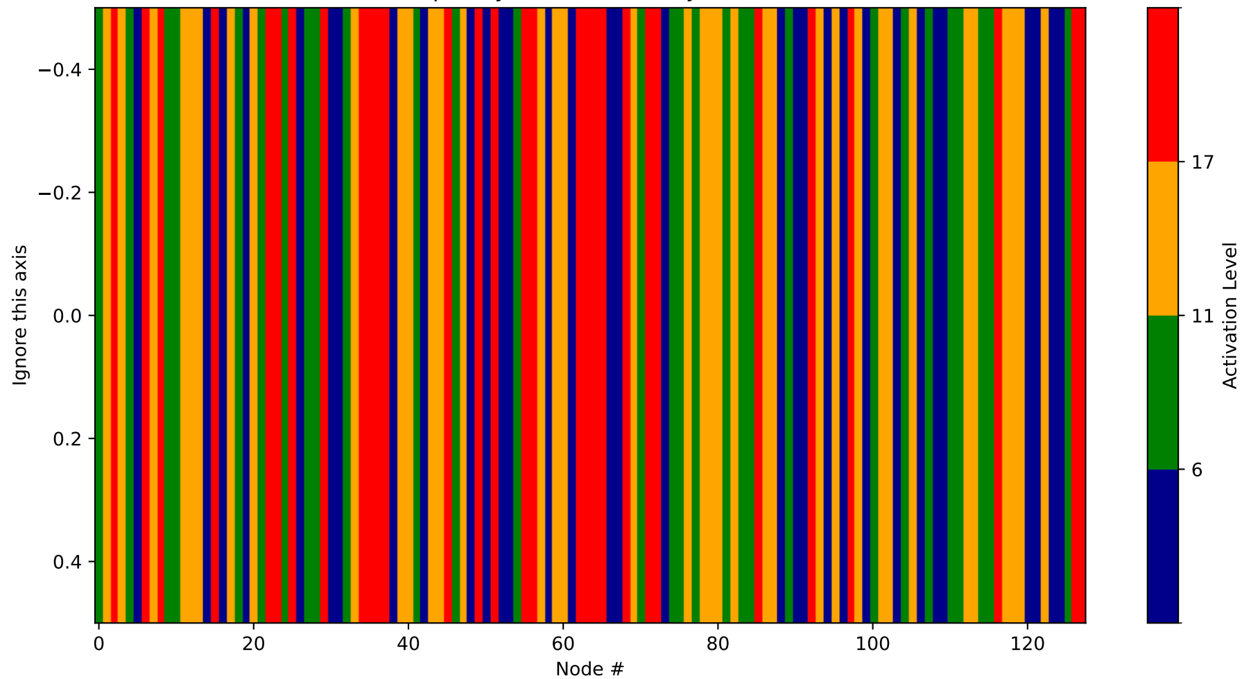
Heatmap - Layer 20 (Probability 2816-2944)
