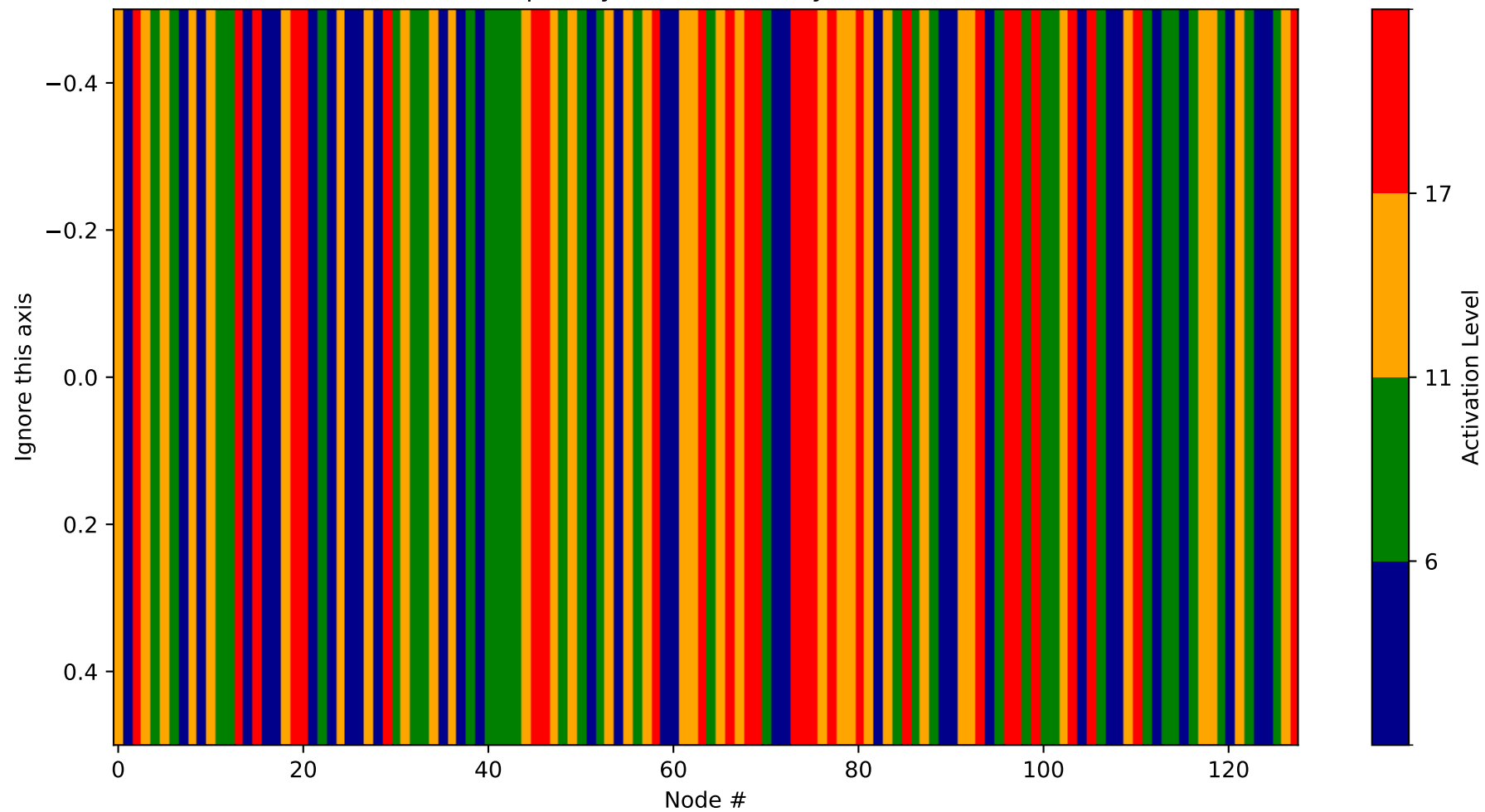
Heatmap - Layer 9 (Probability 3840-3968)
