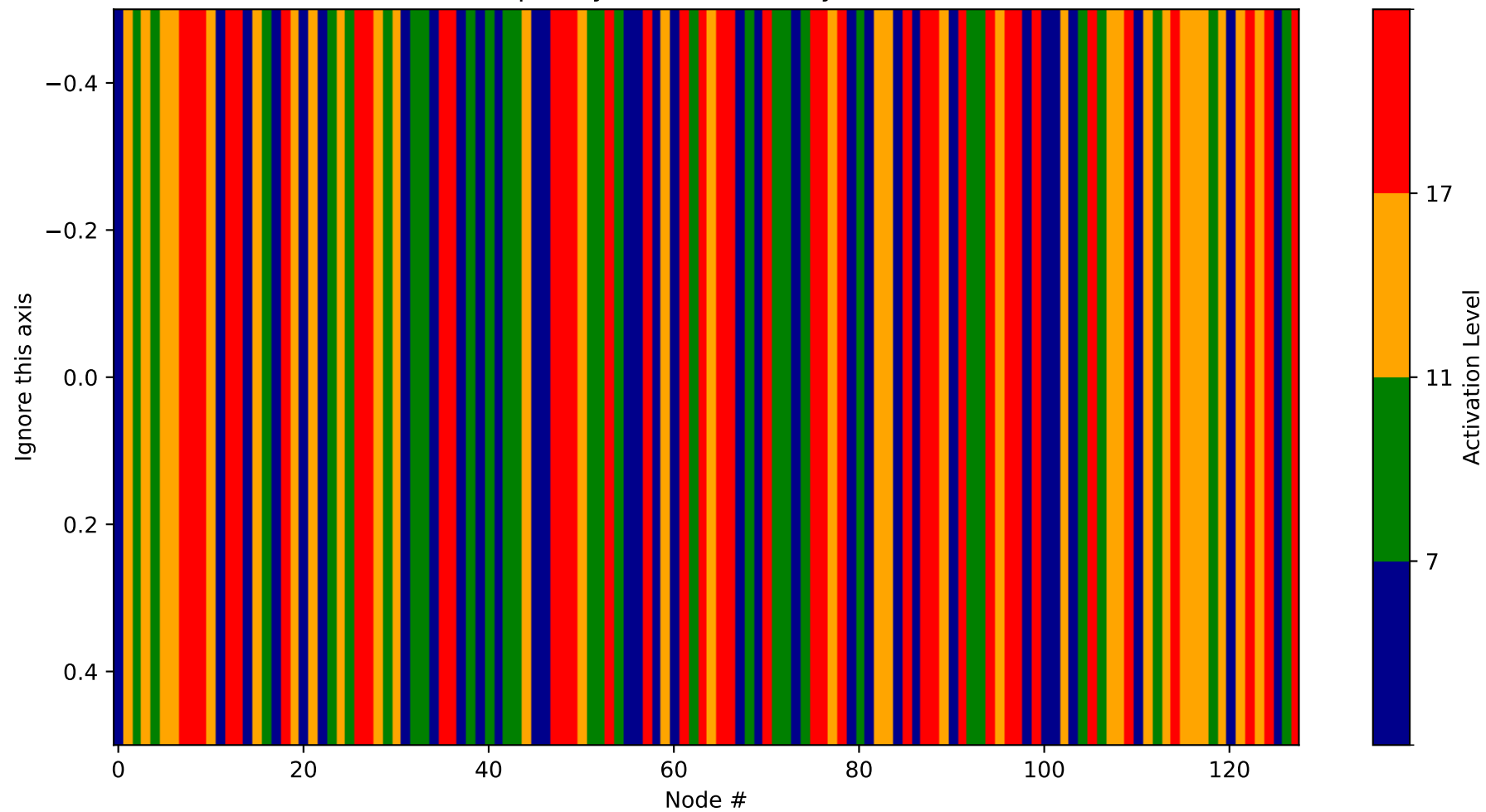
Heatmap - Layer 26 (Probability 3968-4096)
