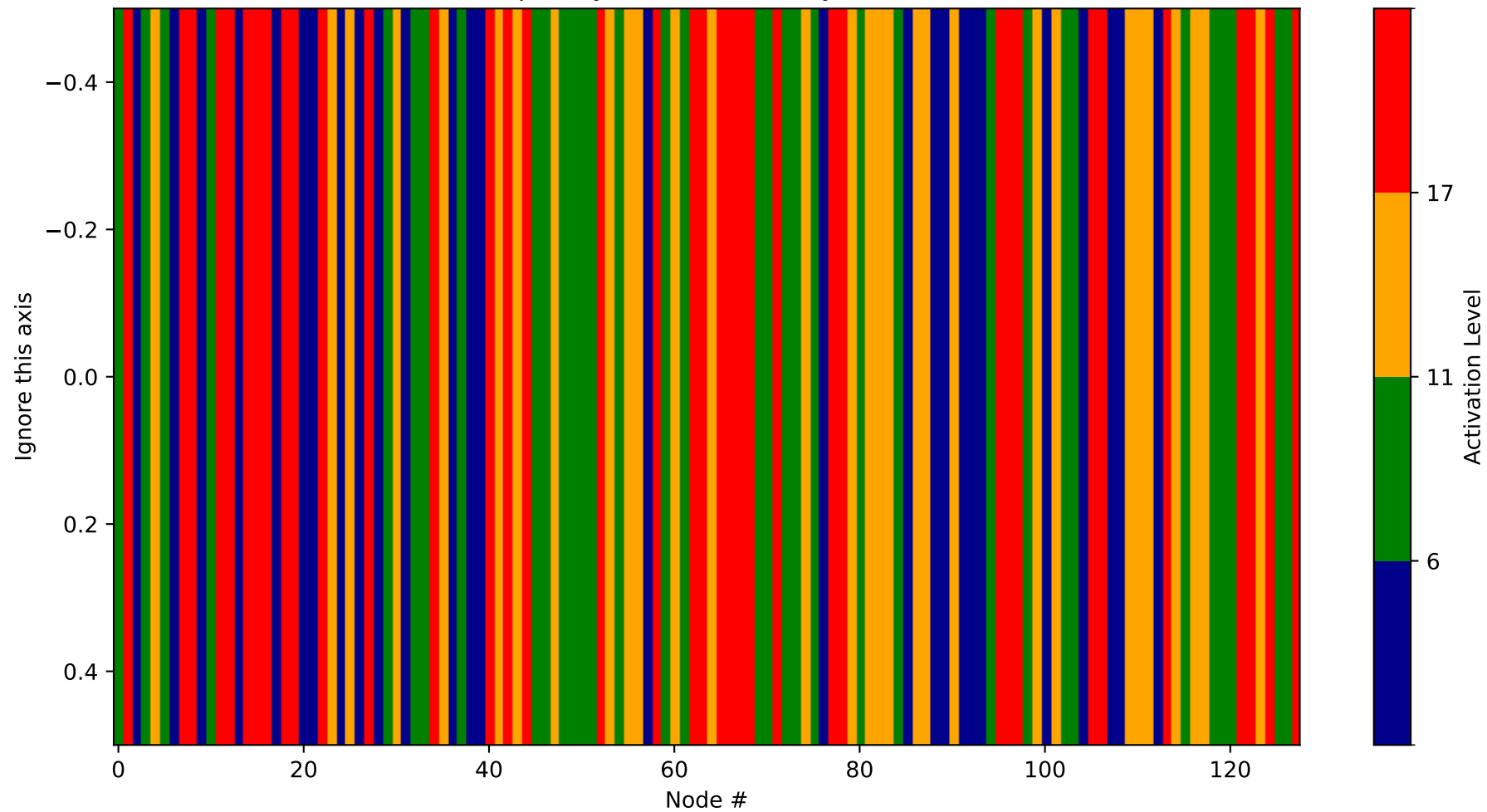
Heatmap - Layer 11 (Probability 1408-1536)
