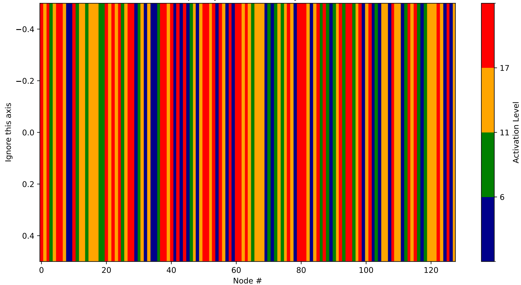
Heatmap - Layer 16 (Probability 384-512)
