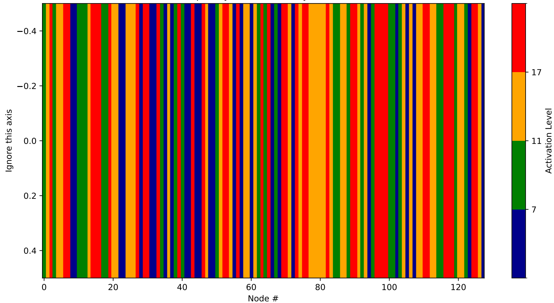
Heatmap - Layer 5 (Probability 3712-3840)
