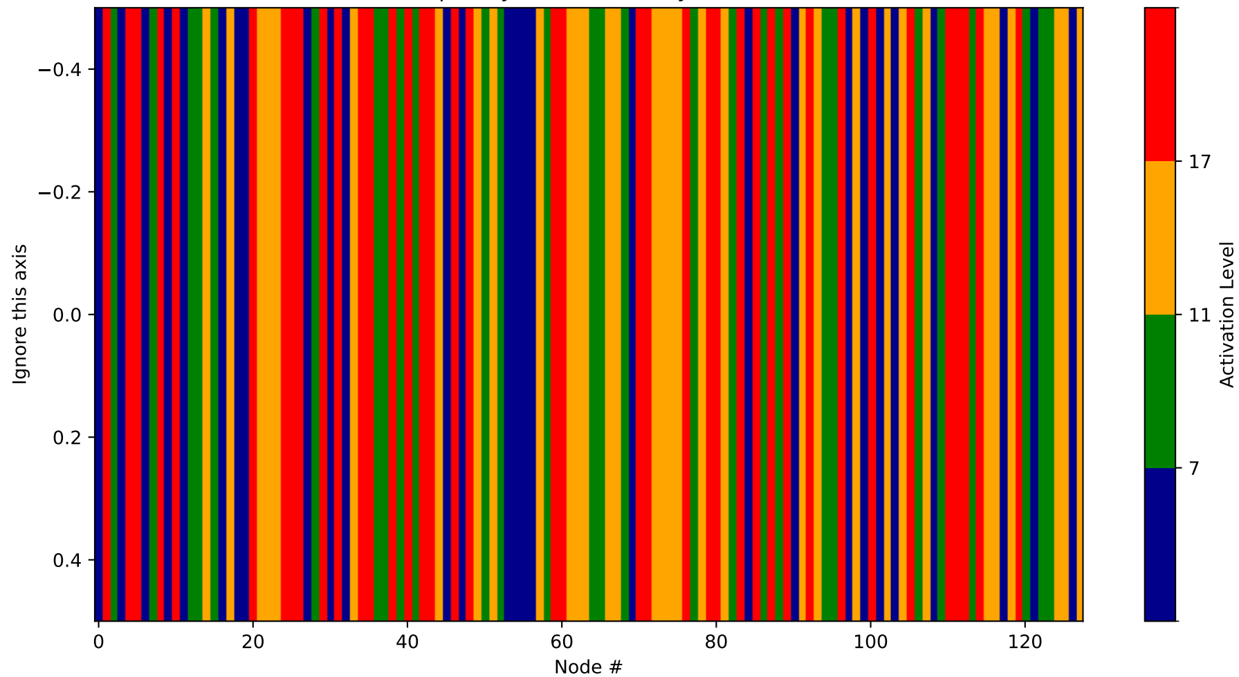
Heatmap - Layer 5 (Probability 2048-2176)
