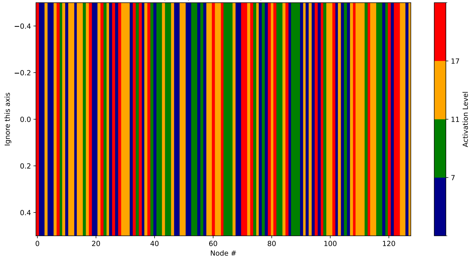
Heatmap - Layer 27 (Probability 2560-2688)
