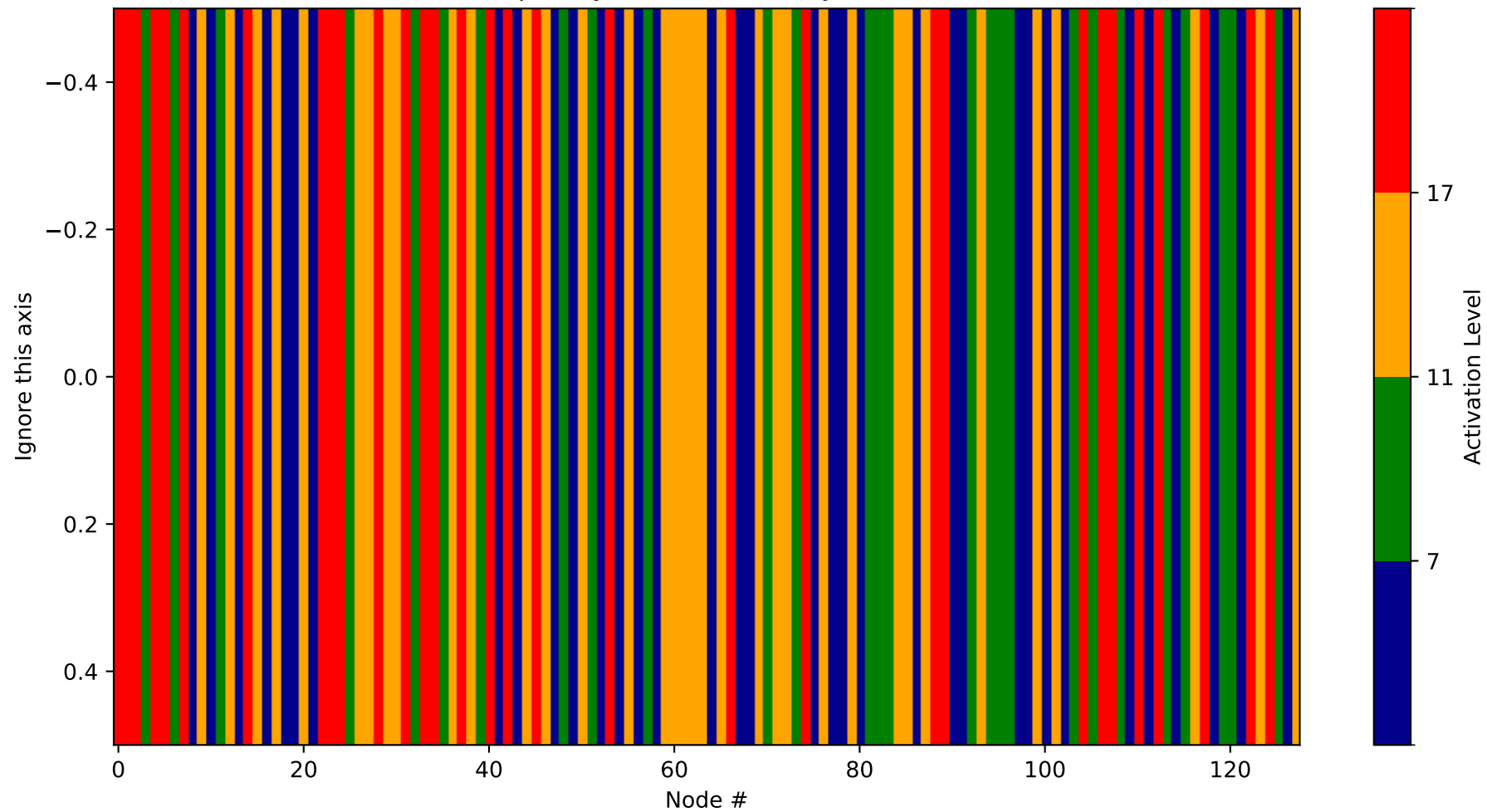
Heatmap - Layer 27 (Probability 1792-1920)
