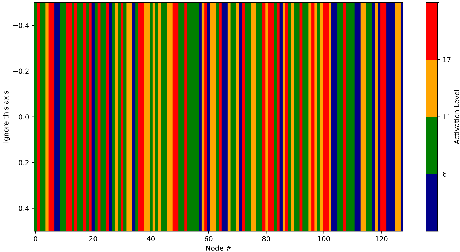
Heatmap - Layer 7 (Probability 128-256)
