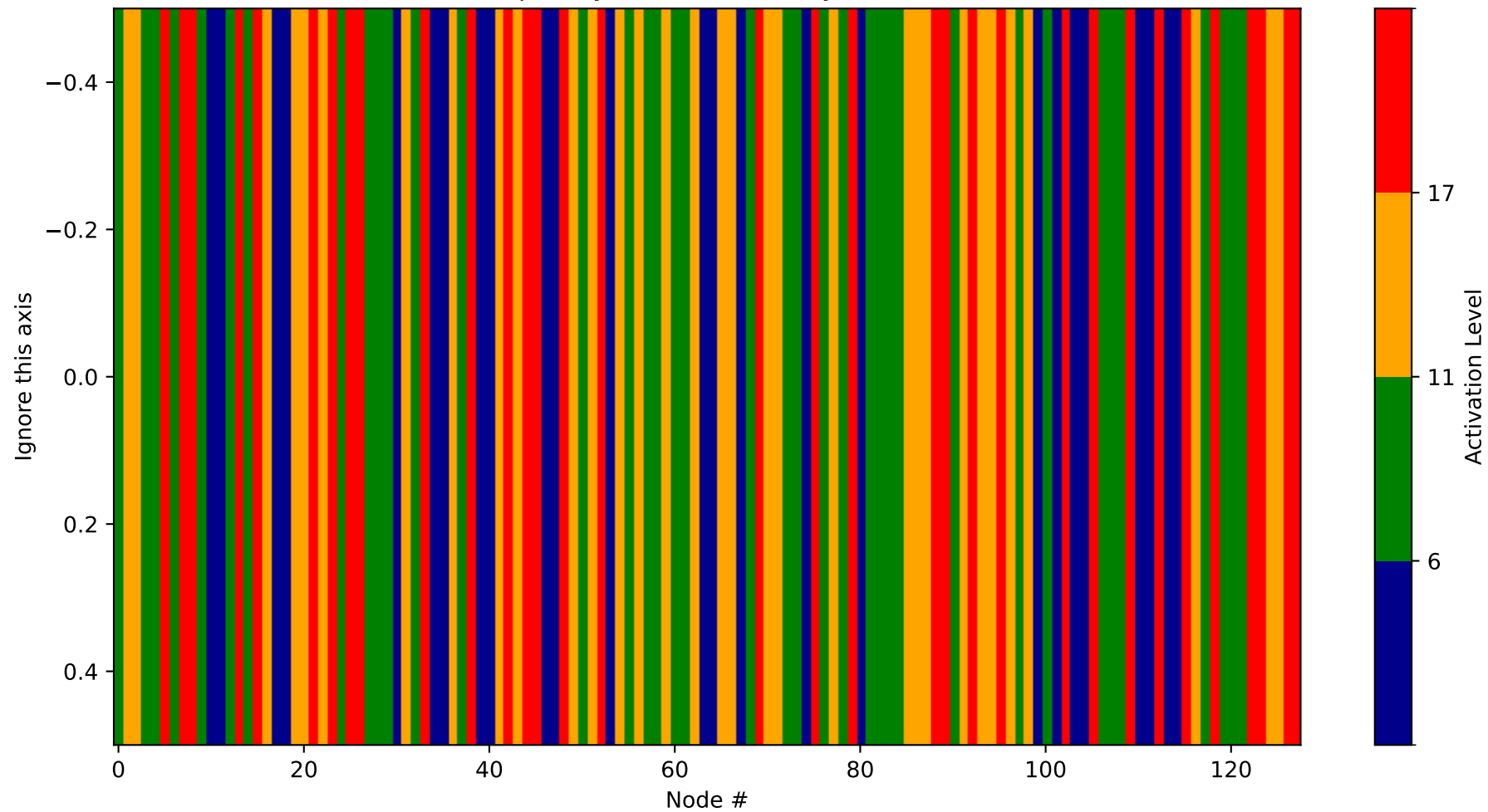
Heatmap - Layer 18 (Probability 2944-3072)
