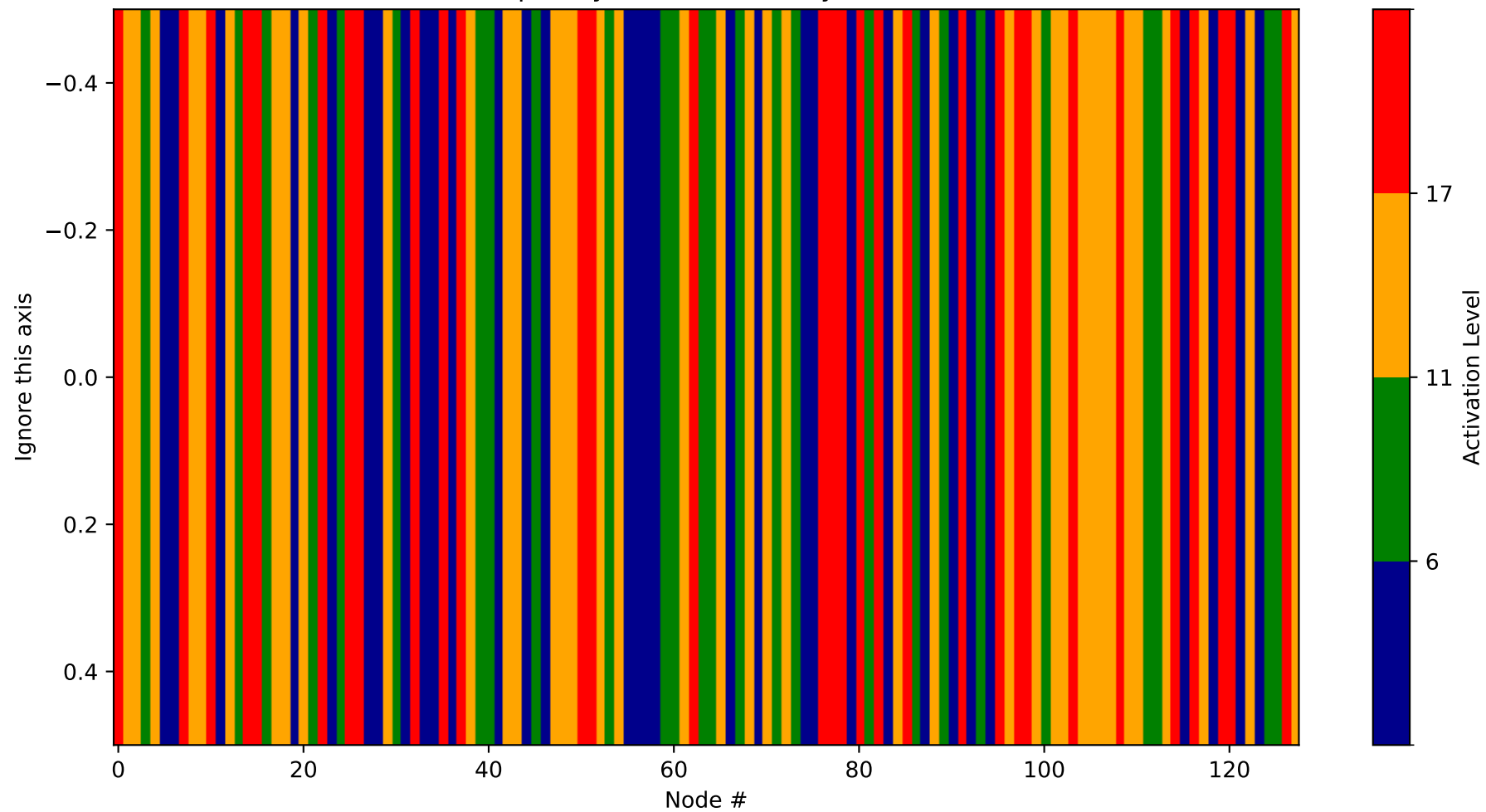
Heatmap - Layer 11 (Probability 1024-1152)
