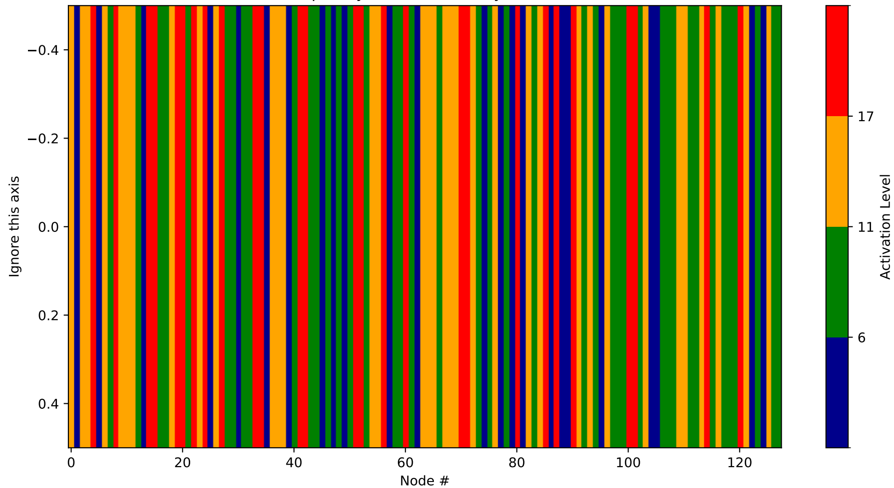
Heatmap - Layer 18 (Probability 1920-2048)
