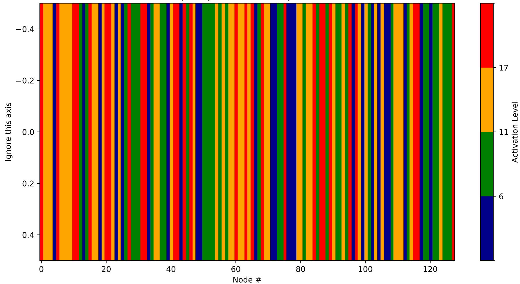
Heatmap - Layer 30 (Probability 3200-3328)
