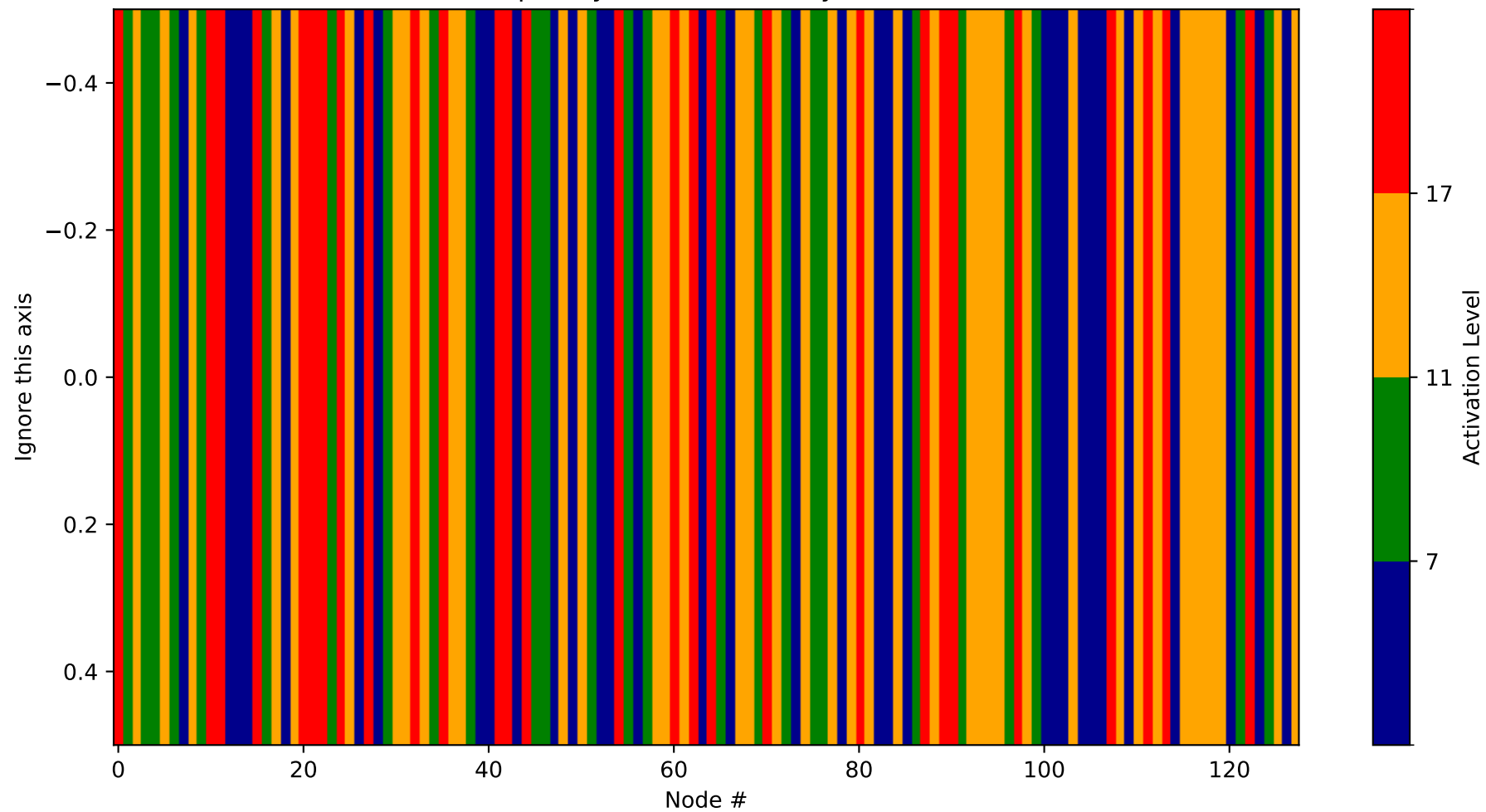
Heatmap - Layer 21 (Probability 3200-3328)
