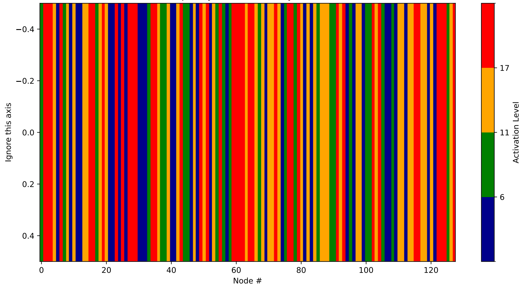
Heatmap - Layer 10 (Probability 2816-2944)
