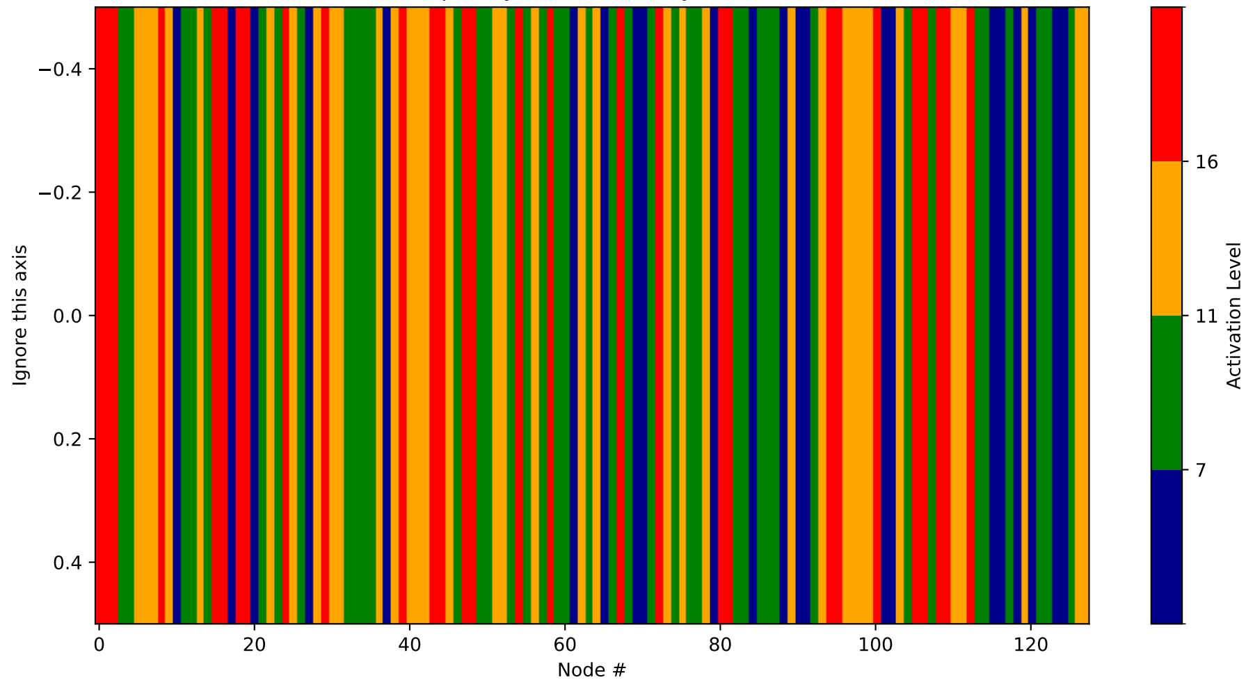
Heatmap - Layer 4 (Probability 1152-1280)
