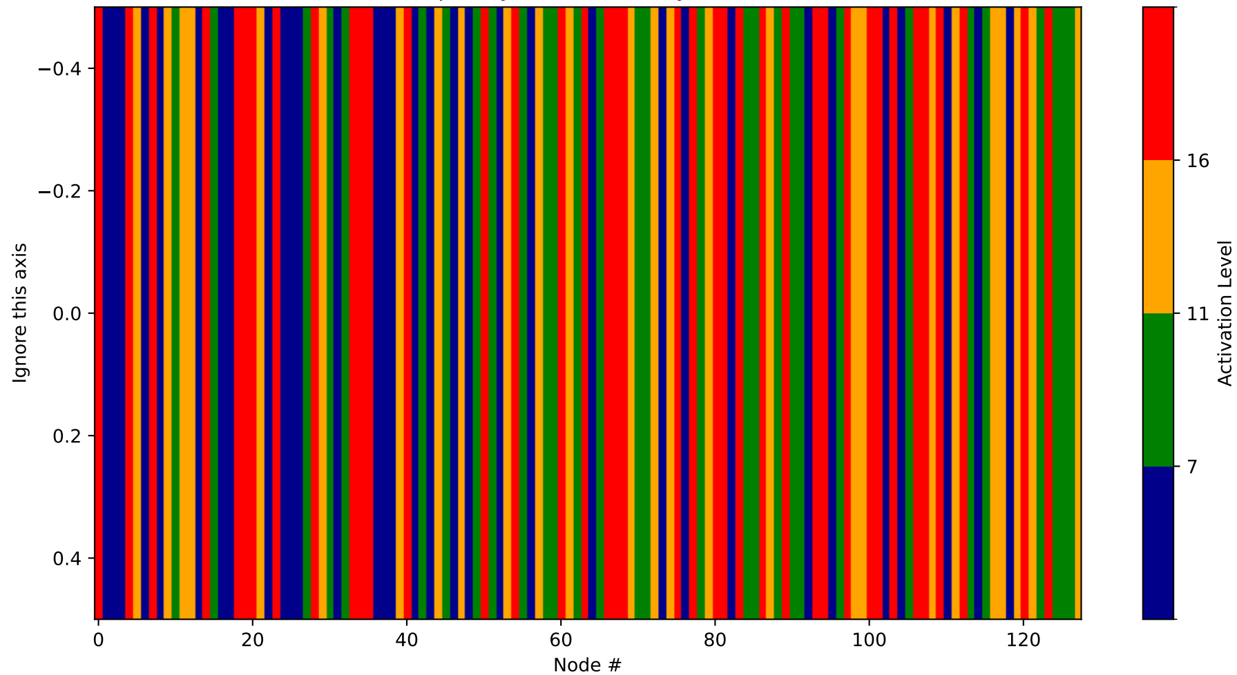
Heatmap - Layer 4 (Probability 1792-1920)
