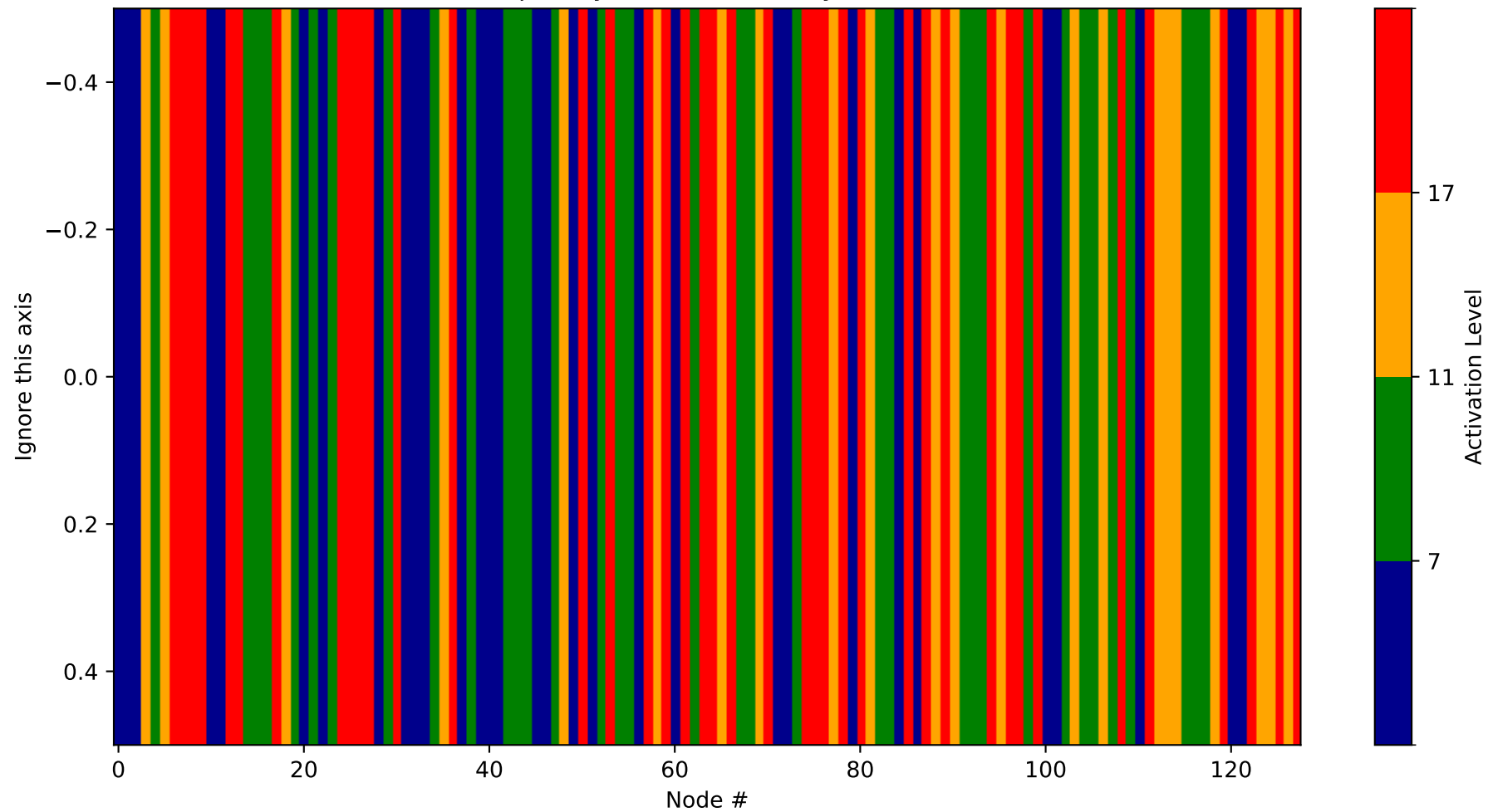
Heatmap - Layer 21 (Probability 3968-4096)
