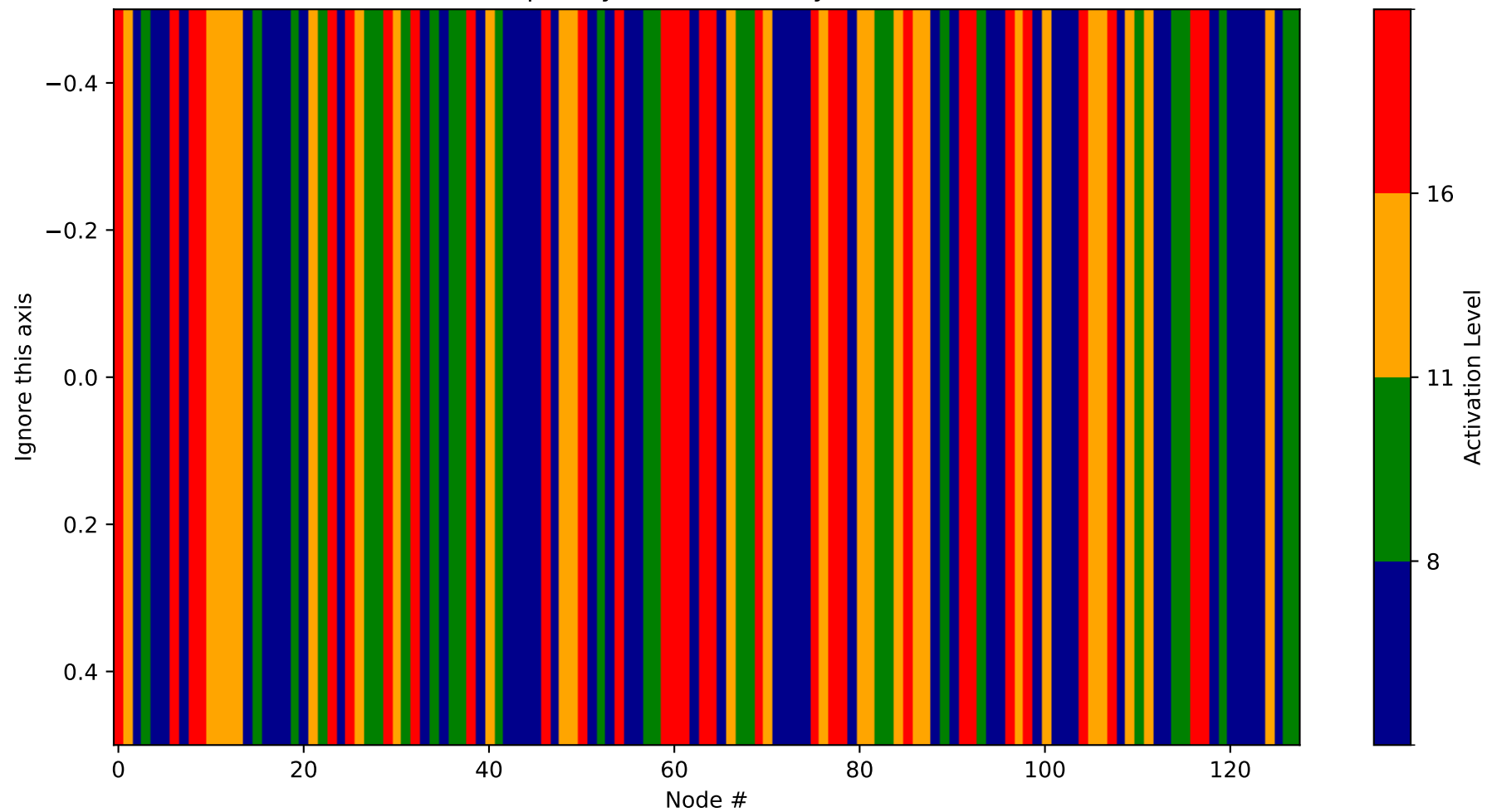
Heatmap - Layer 3 (Probability 3456-3584)
