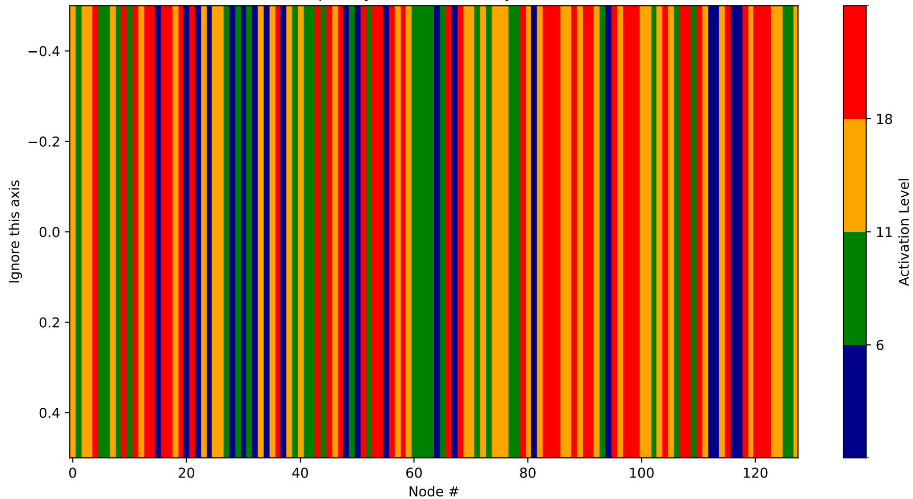
Heatmap - Layer 32 (Probability 1536-1664)
