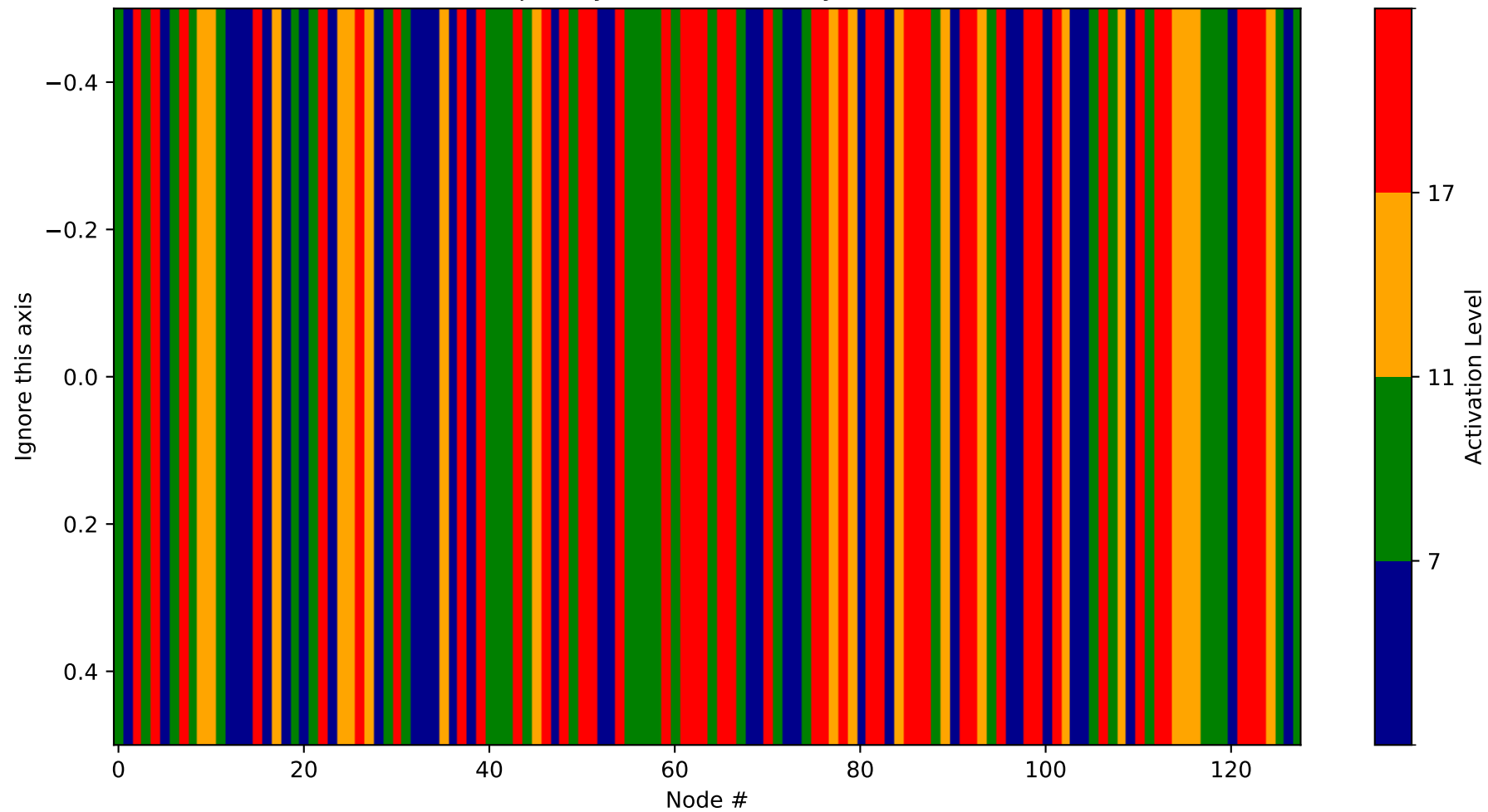
Heatmap - Layer 22 (Probability 2688-2816)
