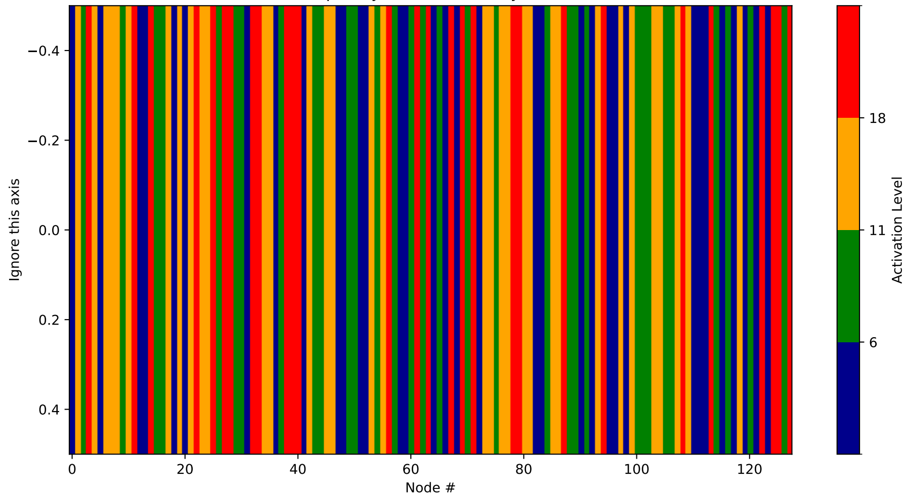
Heatmap - Layer 32 (Probability 768-896)
