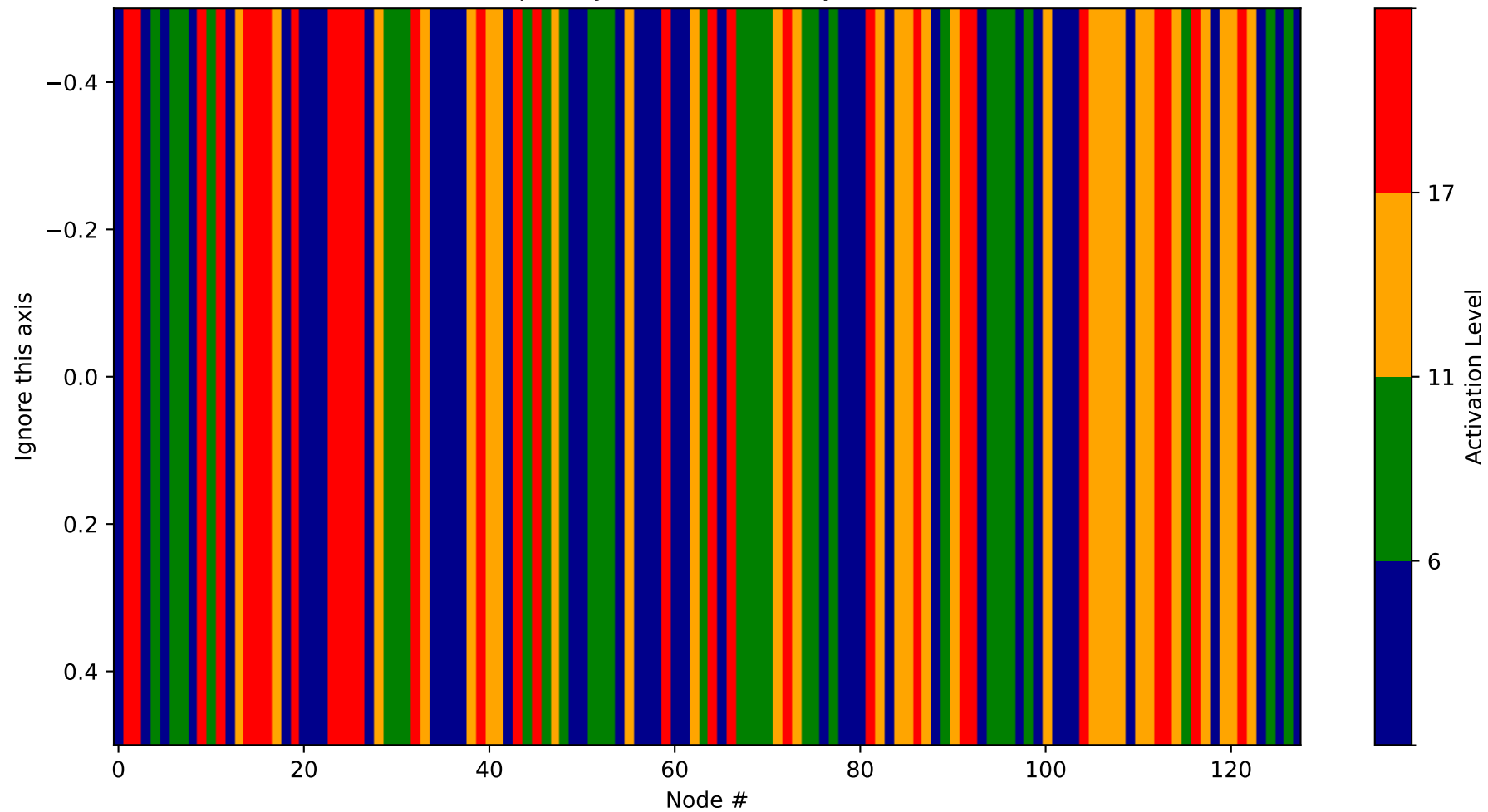
Heatmap - Layer 11 (Probability 1152-1280)
