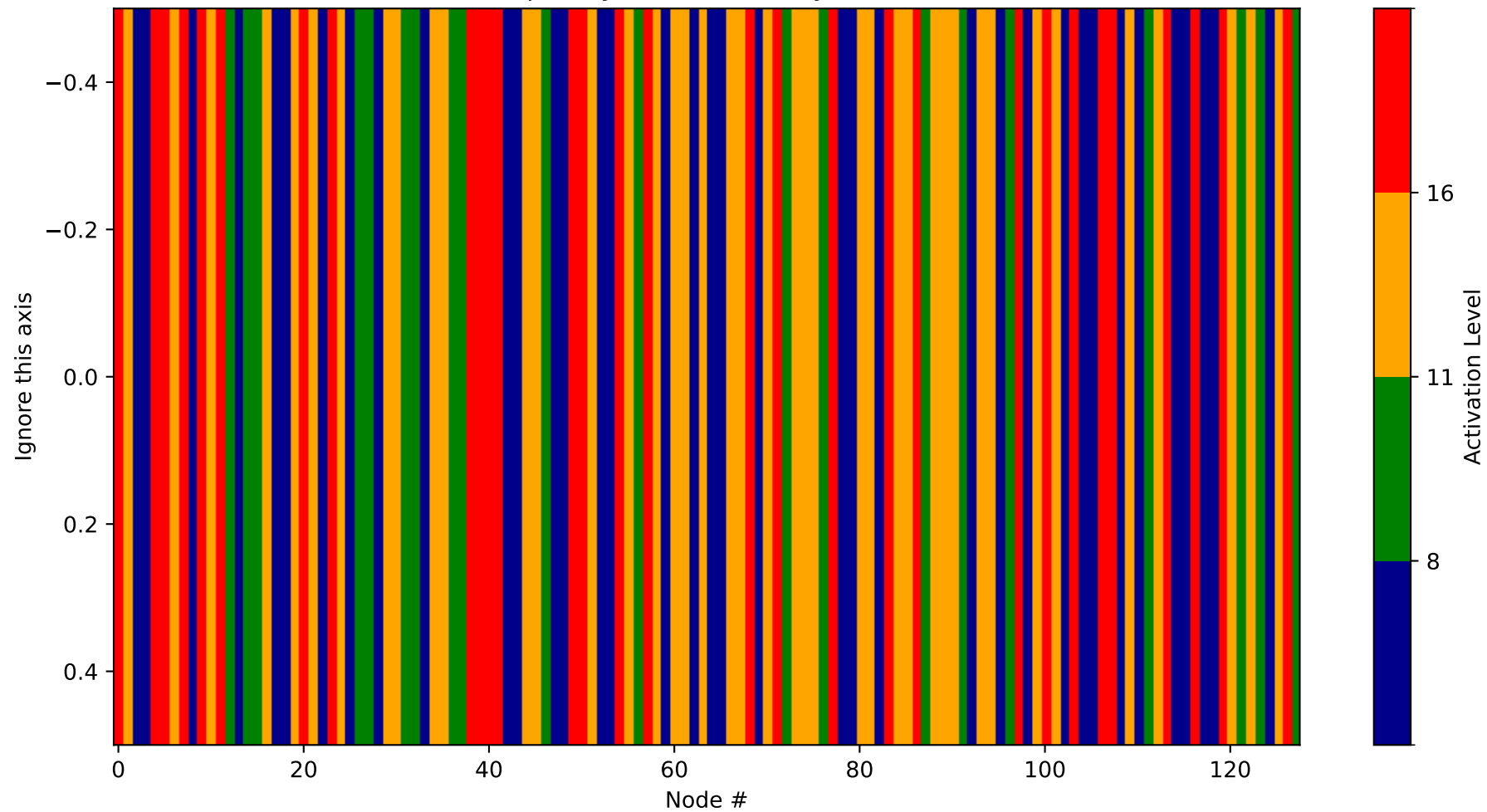
Heatmap - Layer 3 (Probability 1792-1920)
