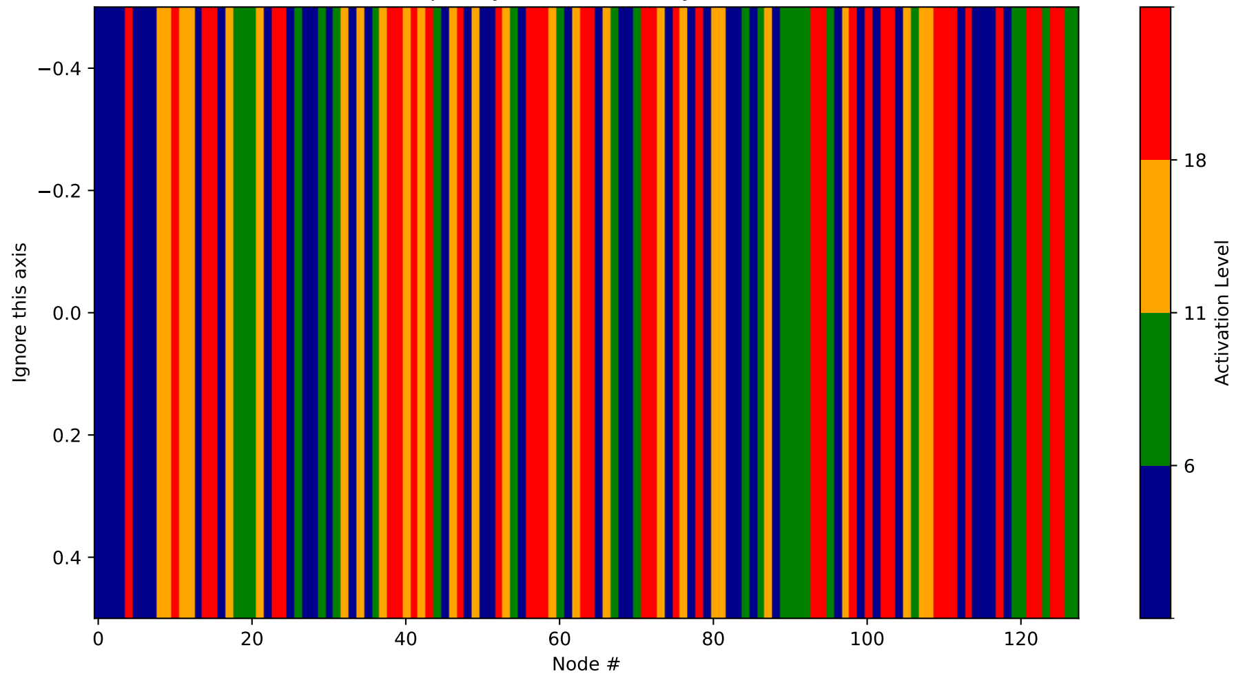
Heatmap - Layer 32 (Probability 2304-2432)
