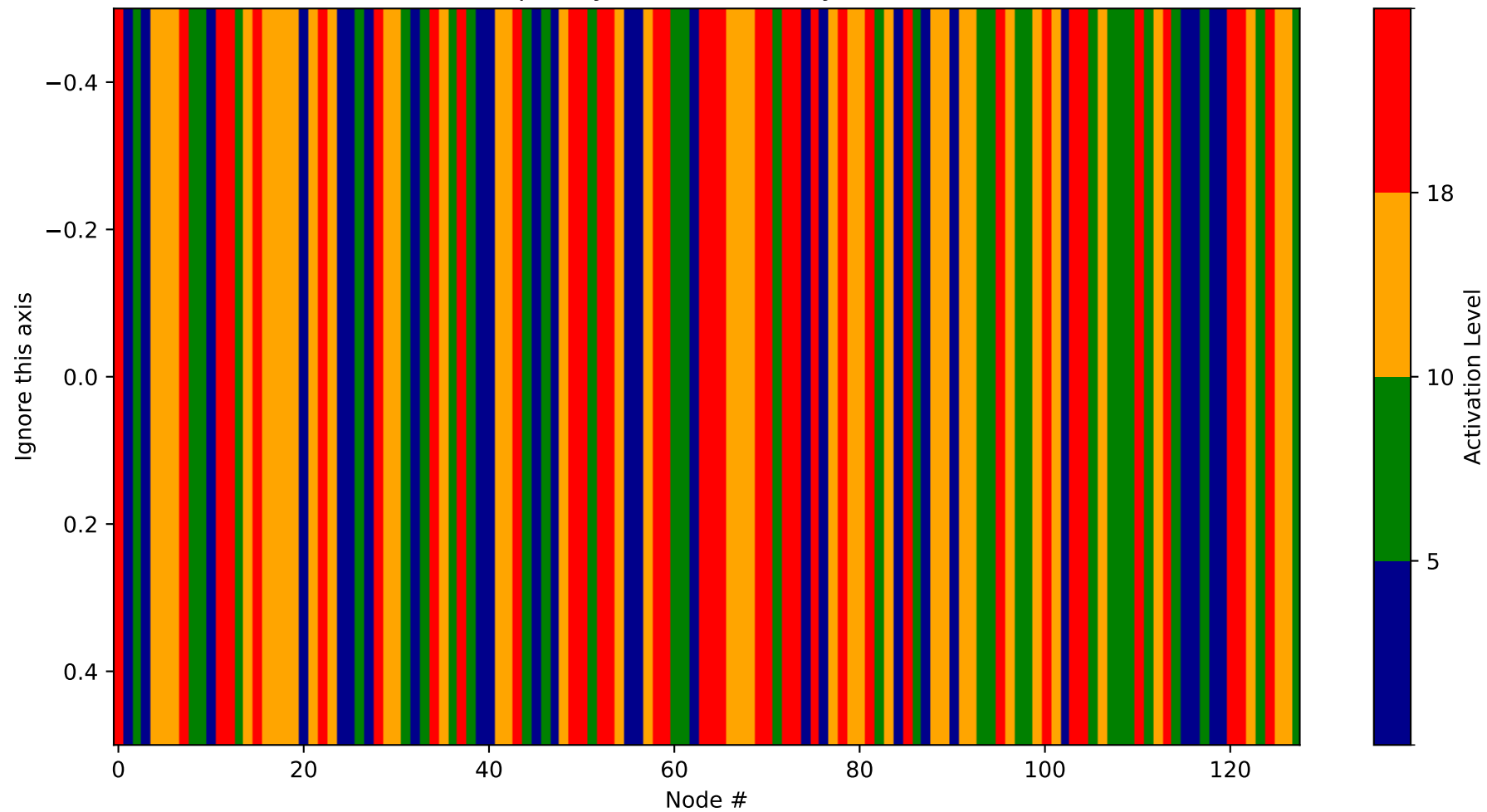
Heatmap - Layer 31 (Probability 2560-2688)
