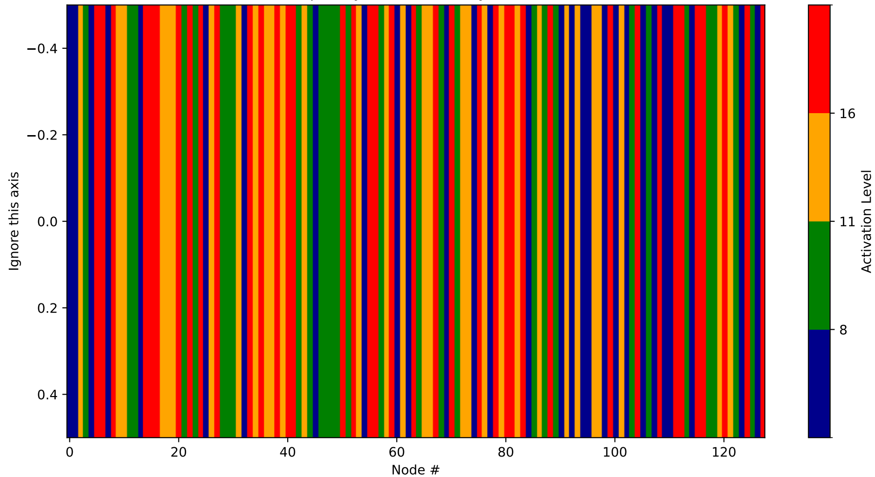
Heatmap - Layer 2 (Probability 3072-3200)
