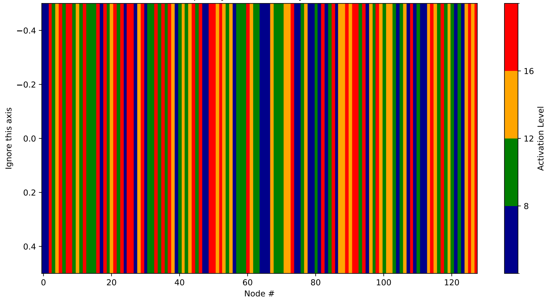
Heatmap - Layer 0 (Probability 2176-2304)
