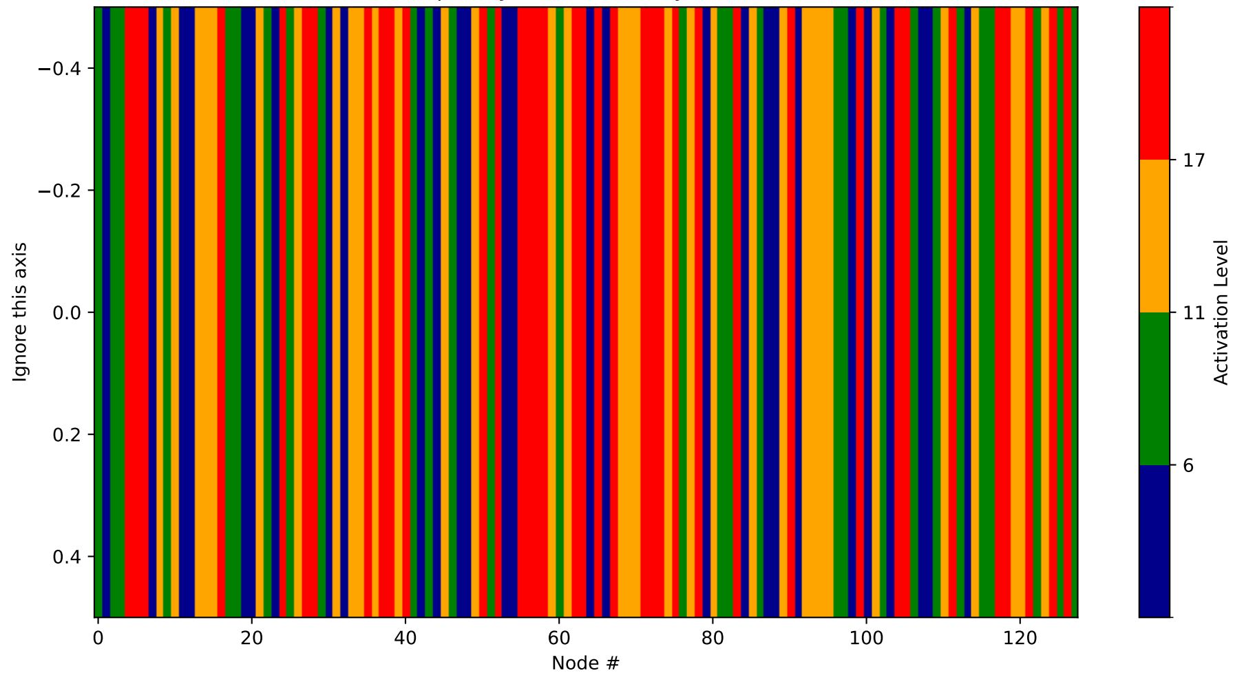
Heatmap - Layer 7 (Probability 3072-3200)
