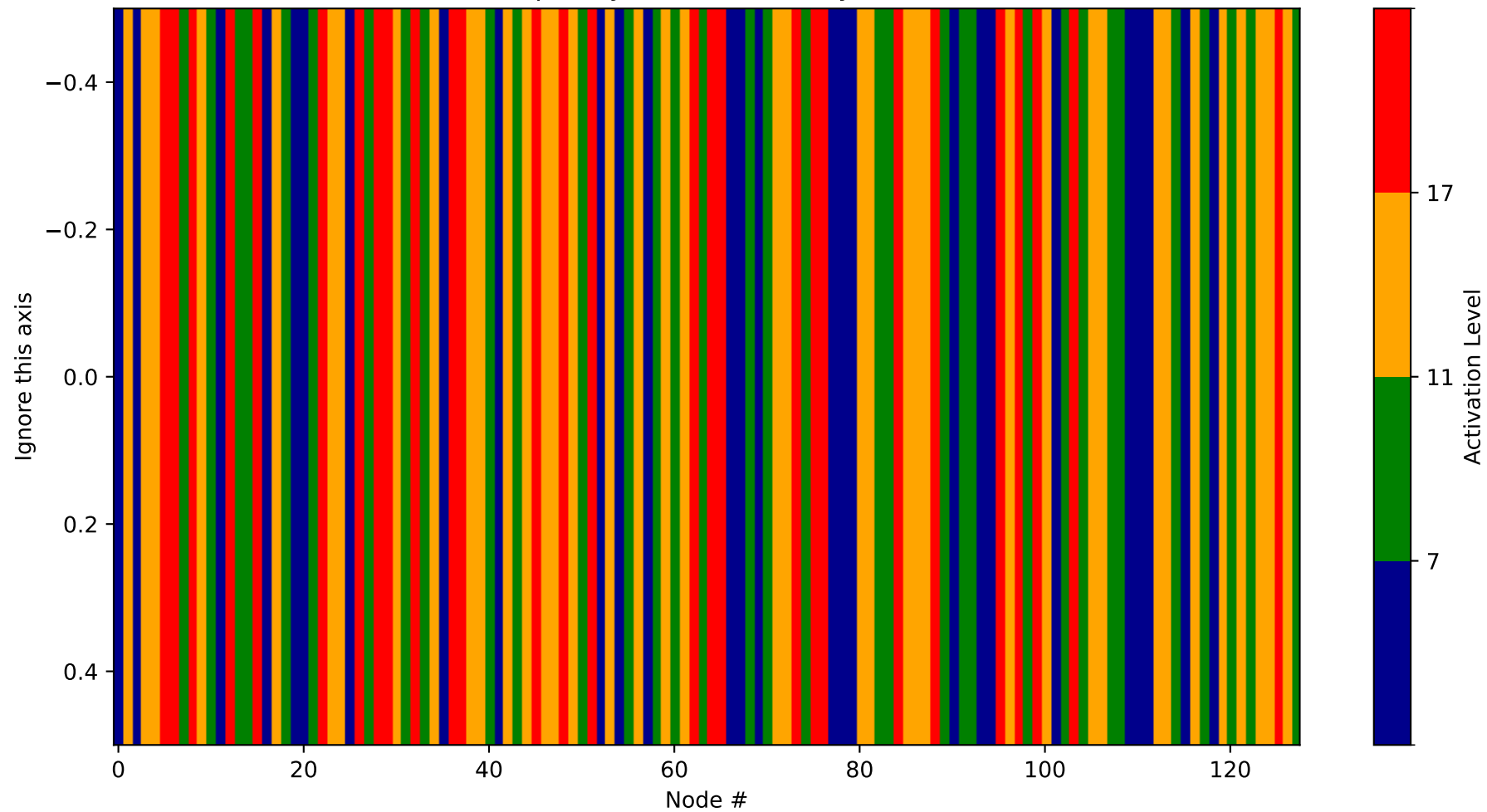
Heatmap - Layer 27 (Probability 128-256)
