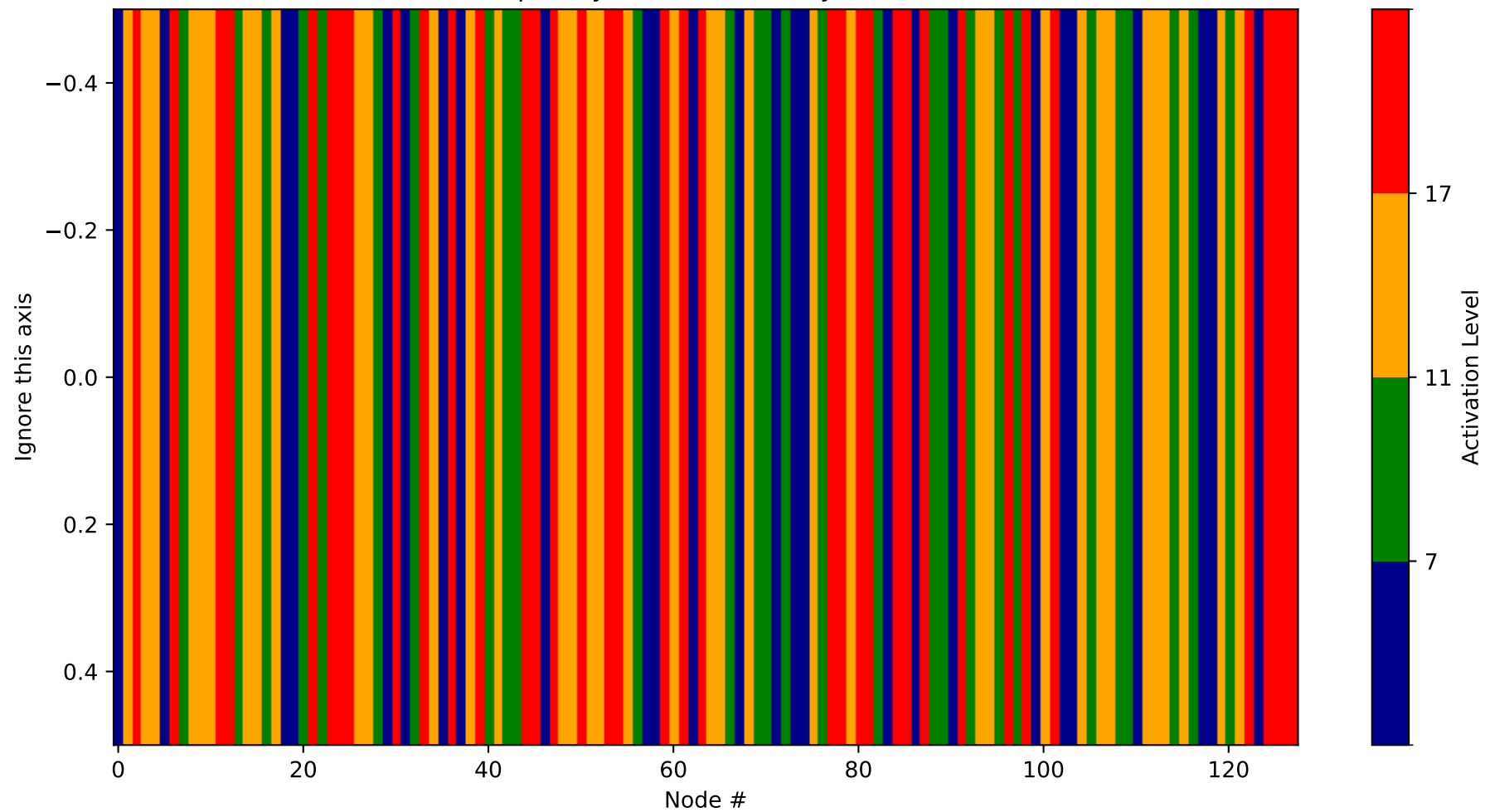
Heatmap - Layer 27 (Probability 3712-3840)
