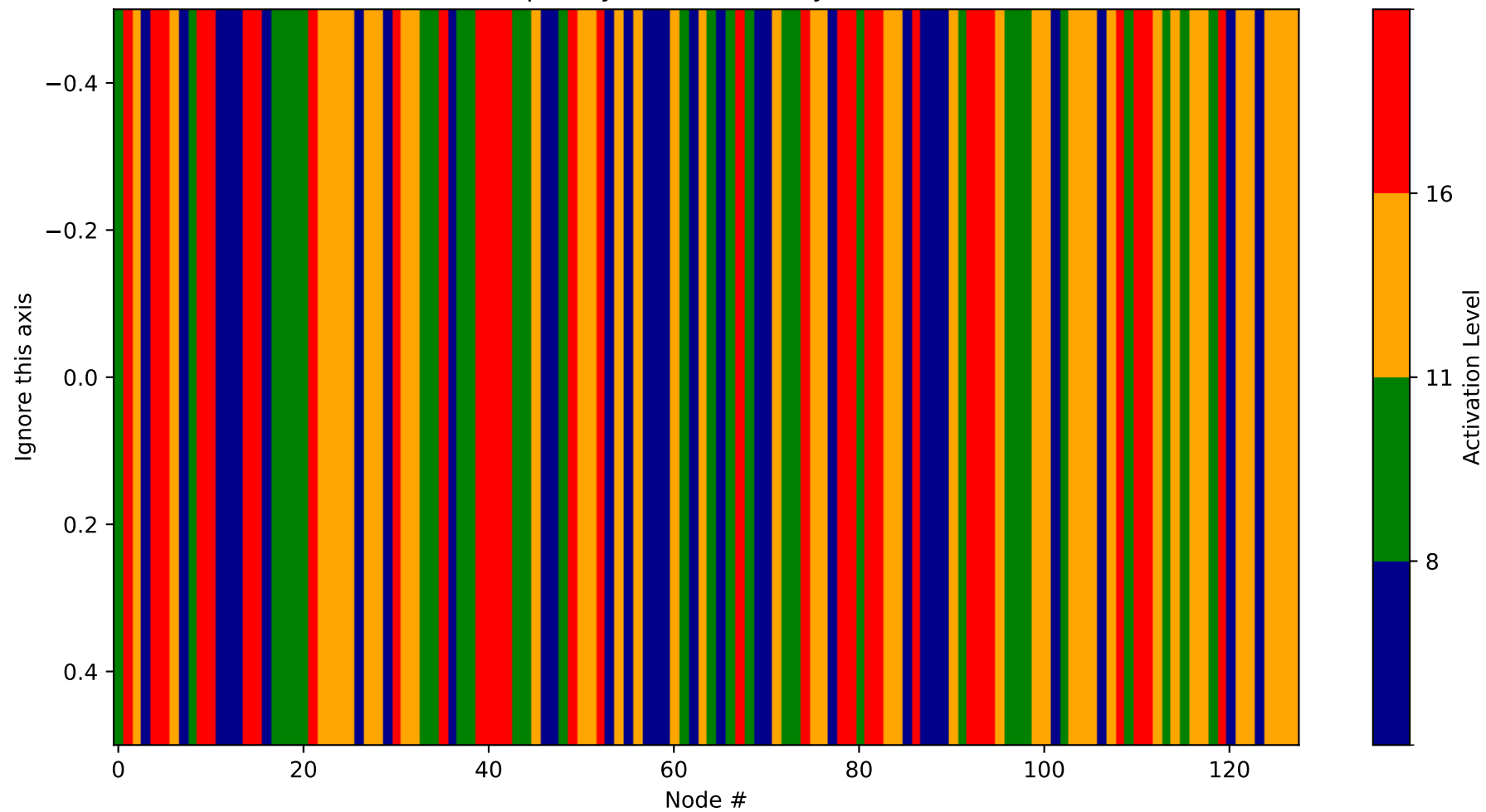
Heatmap - Layer 2 (Probability 2048-2176)
