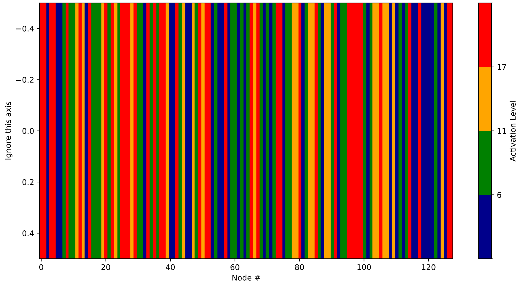
Heatmap - Layer 17 (Probability 1024-1152)
