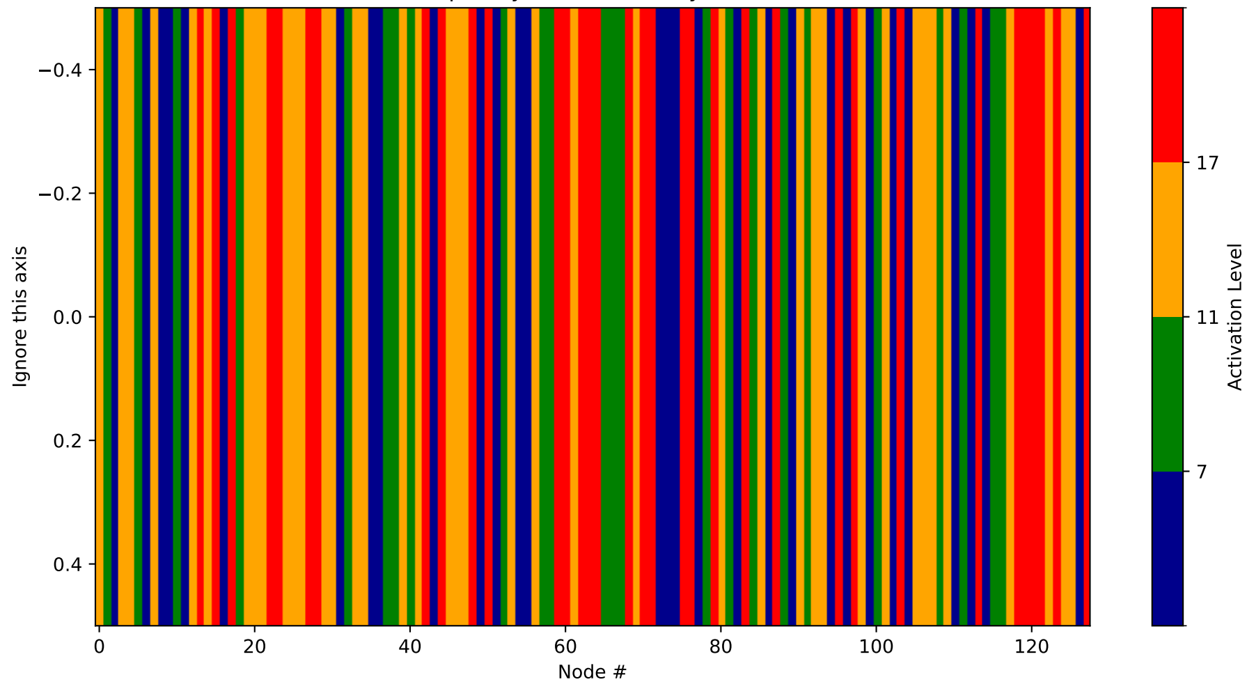
Heatmap - Layer 5 (Probability 896-1024)
