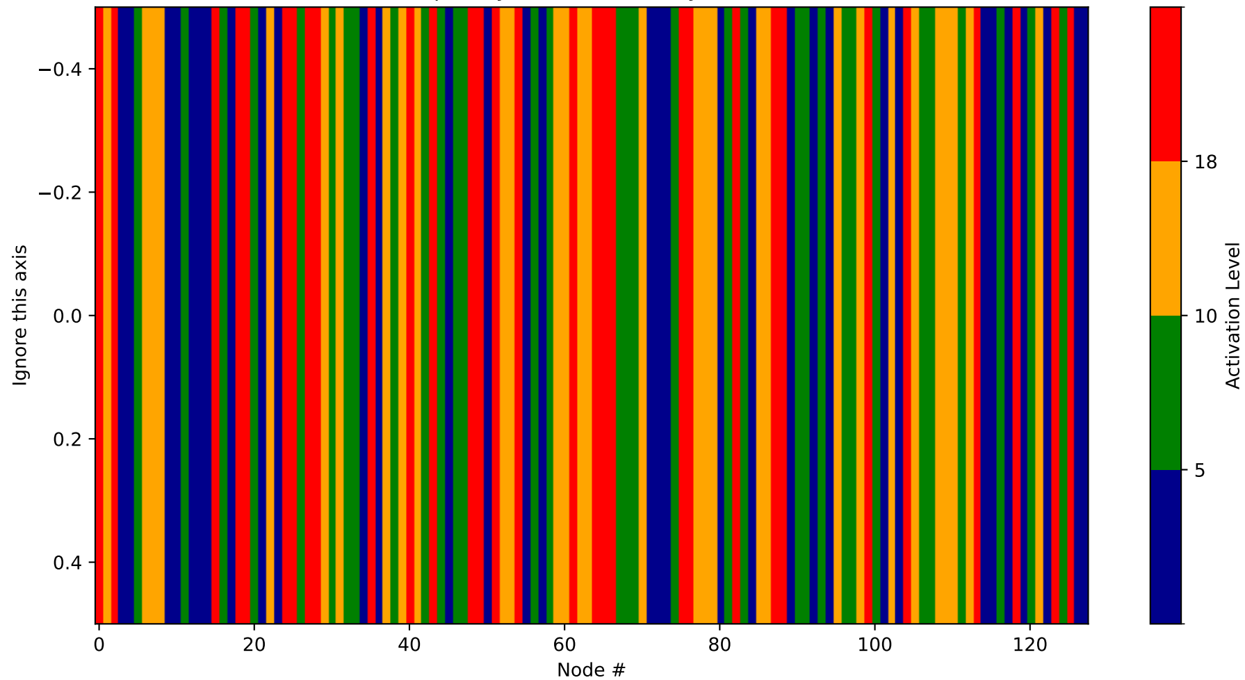
Heatmap - Layer 31 (Probability 2688-2816)
