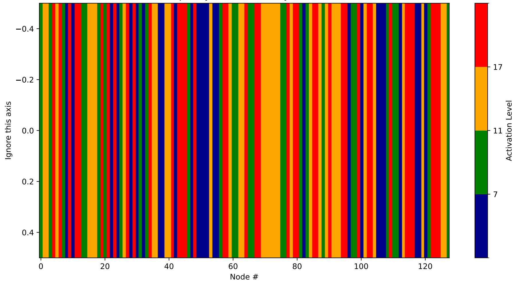
Heatmap - Layer 23 (Probability 1536-1664)
