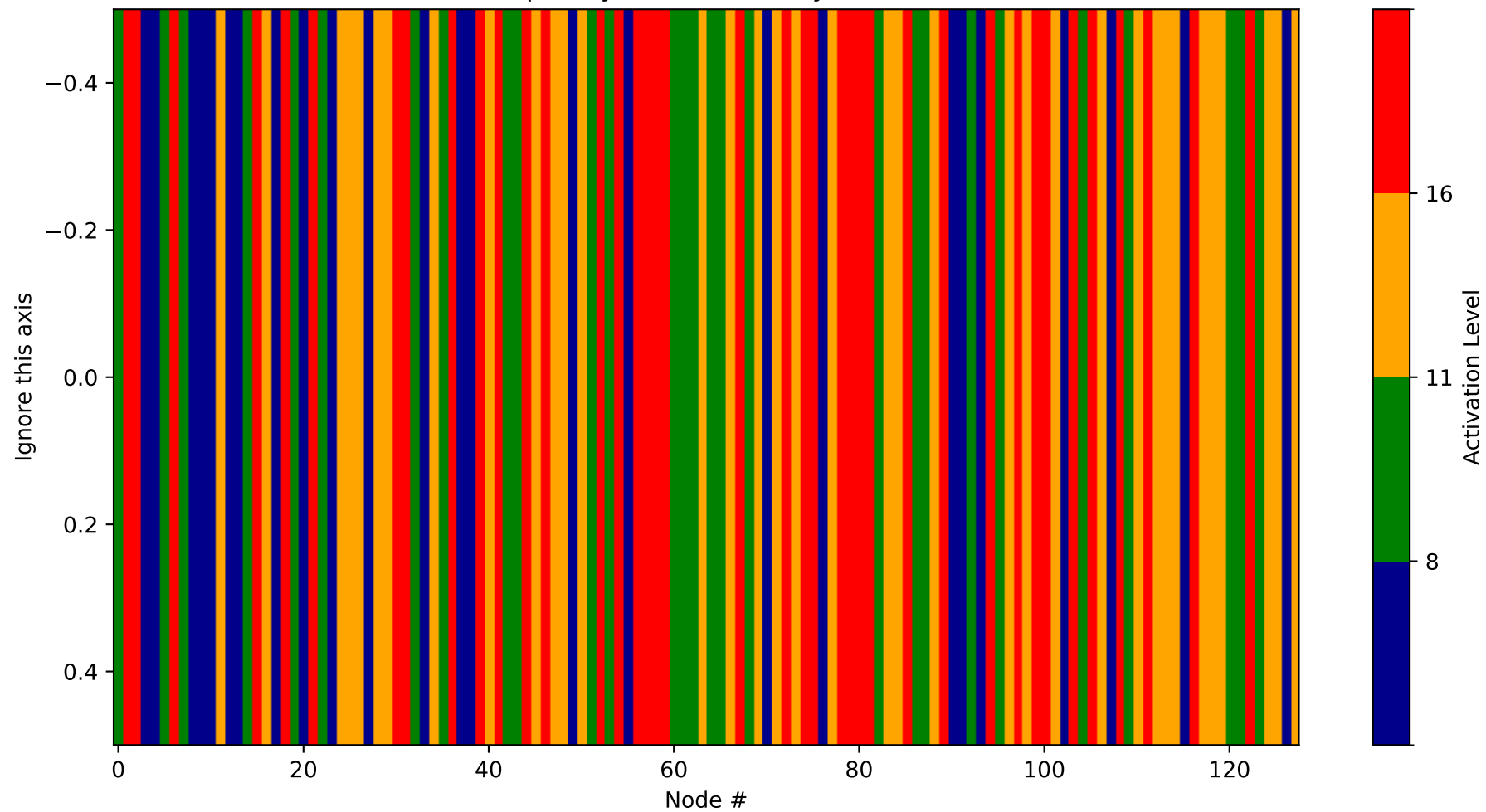
Heatmap - Layer 2 (Probability 1152-1280)
