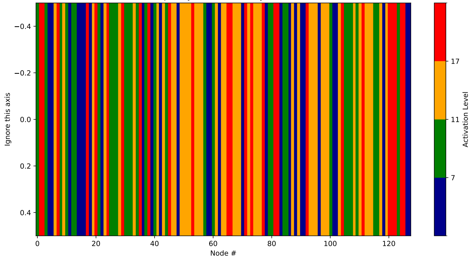
Heatmap - Layer 25 (Probability 2432-2560)
