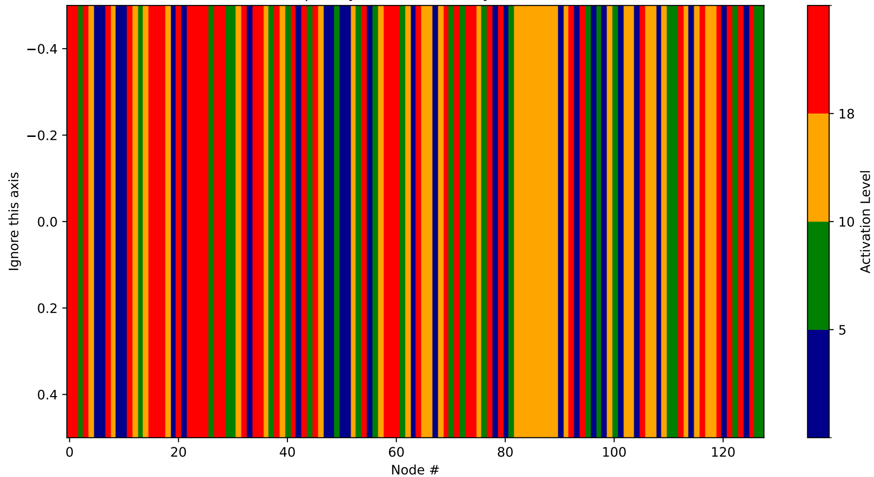
Heatmap - Layer 31 (Probability 1408-1536)
