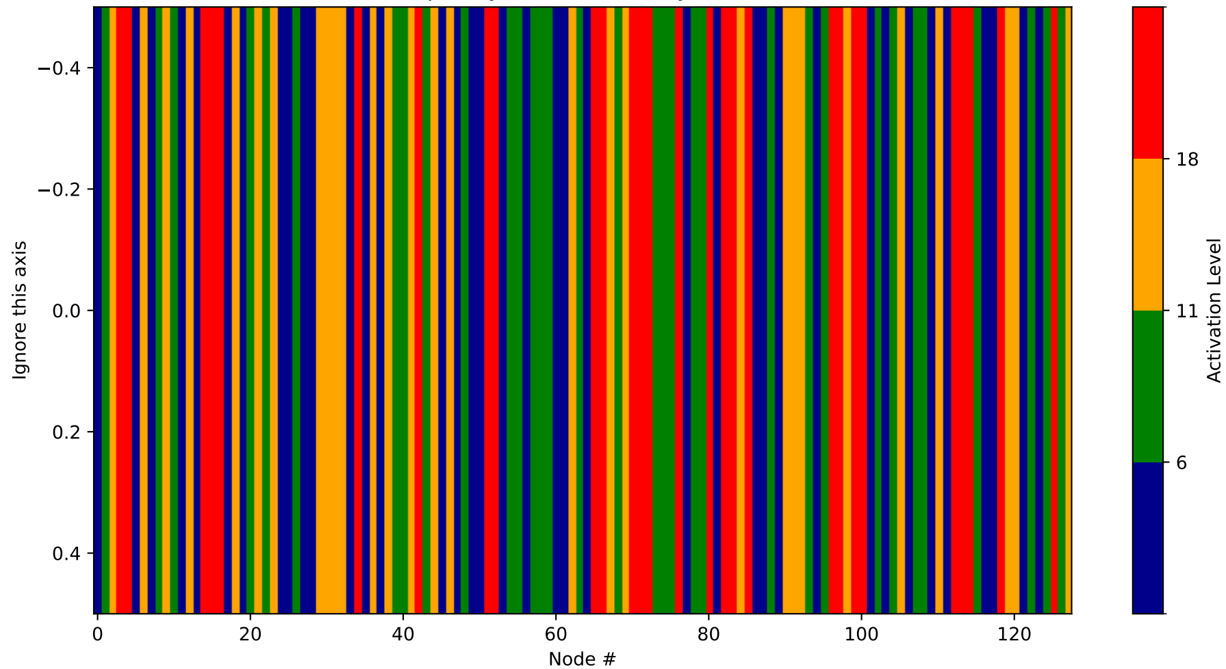
Heatmap - Layer 14 (Probability 1920-2048)
