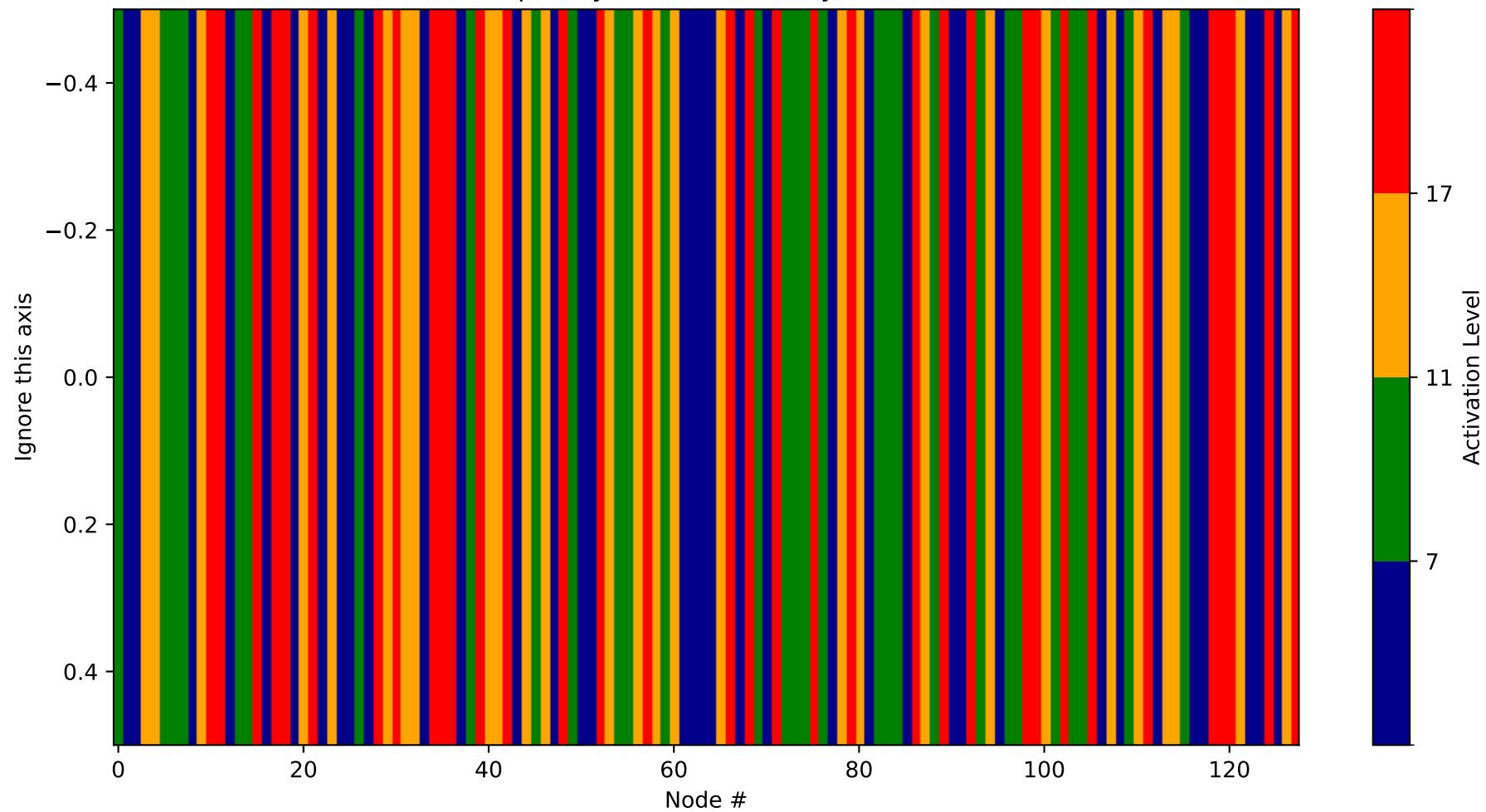
Heatmap - Layer 25 (Probability 2048-2176)
