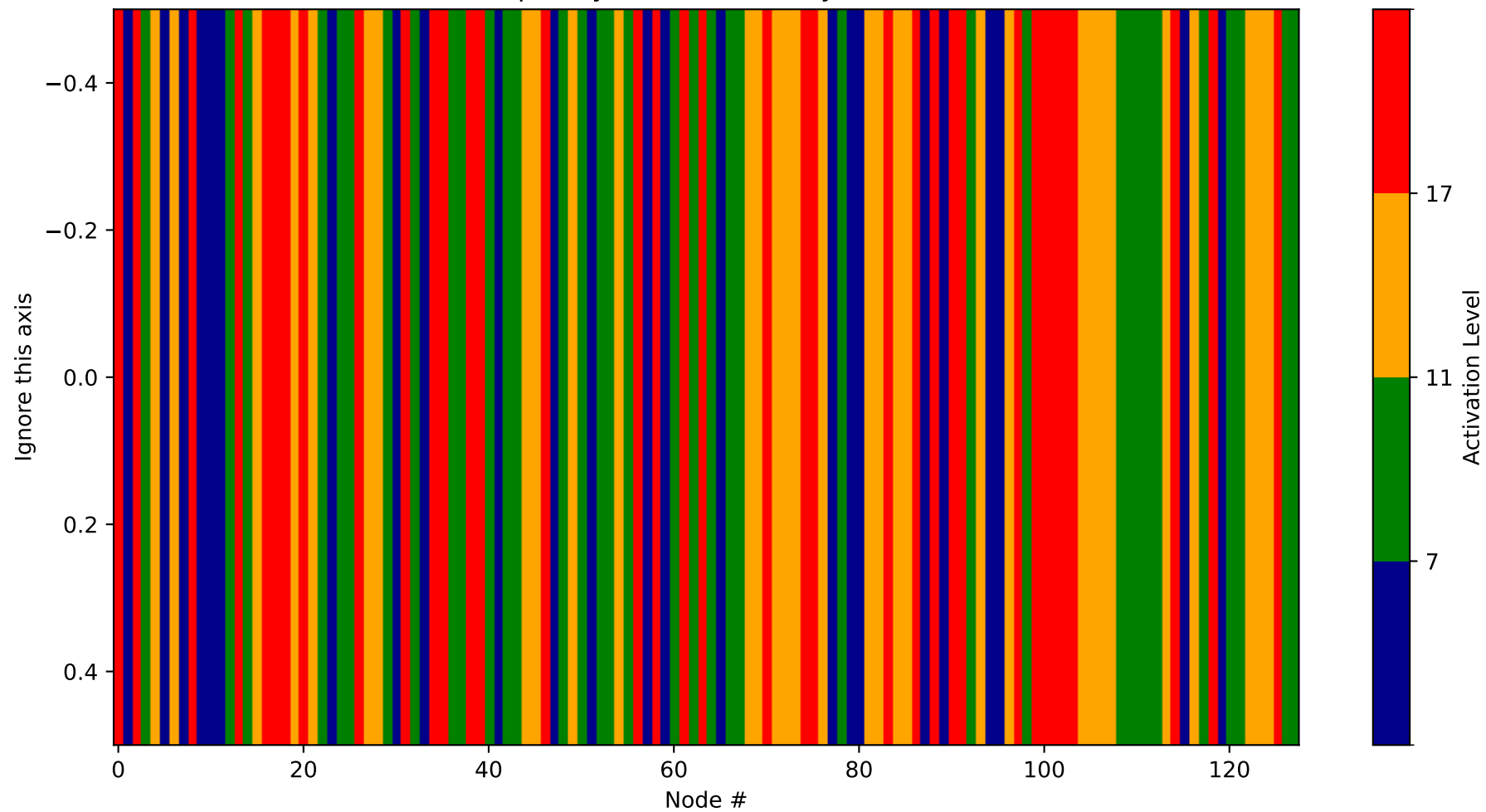
Heatmap - Layer 26 (Probability 3840-3968)
