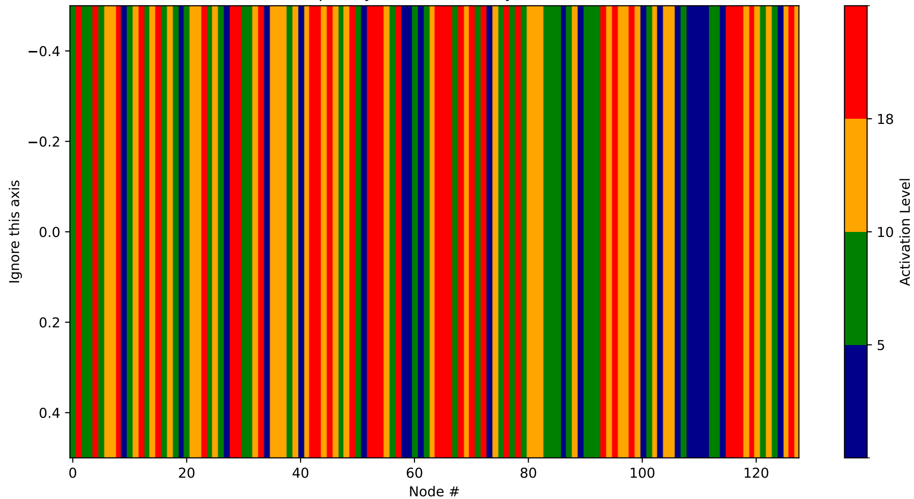
Heatmap - Layer 31 (Probability 2816-2944)
