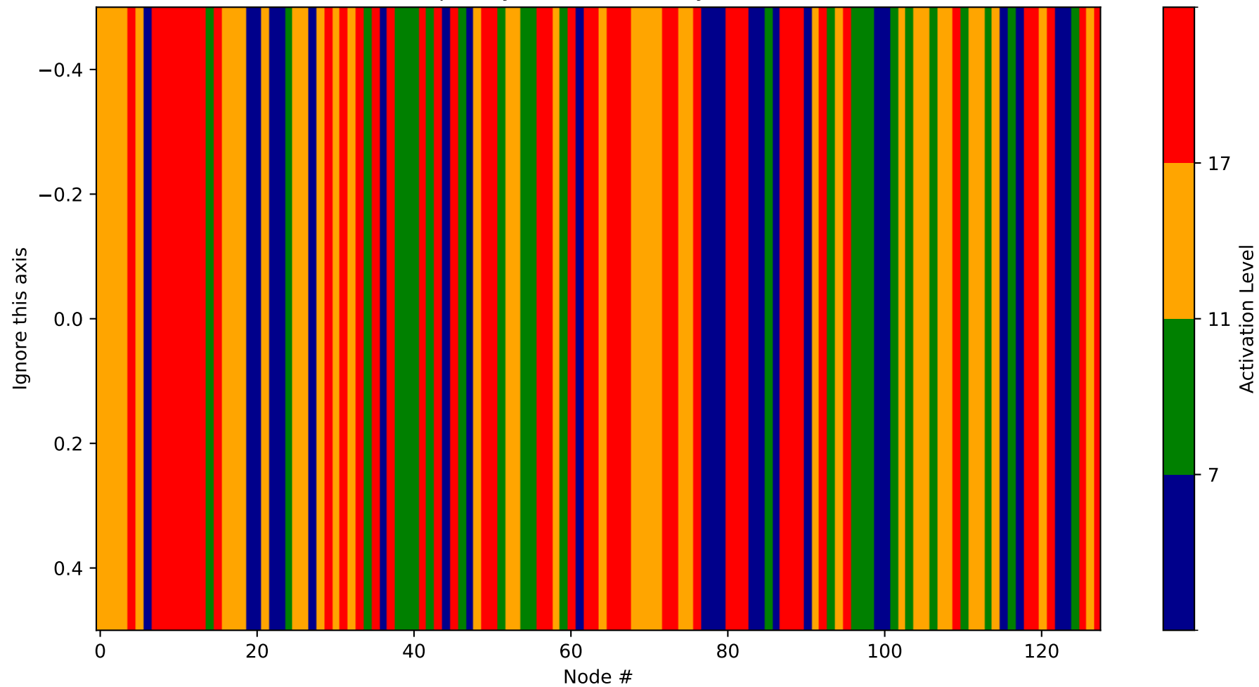
Heatmap - Layer 26 (Probability 2176-2304)
