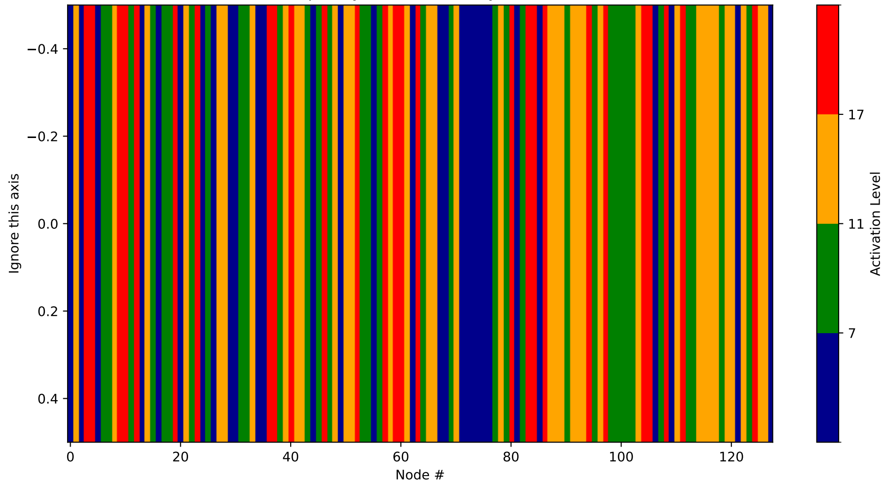
Heatmap - Layer 25 (Probability 3456-3584)
