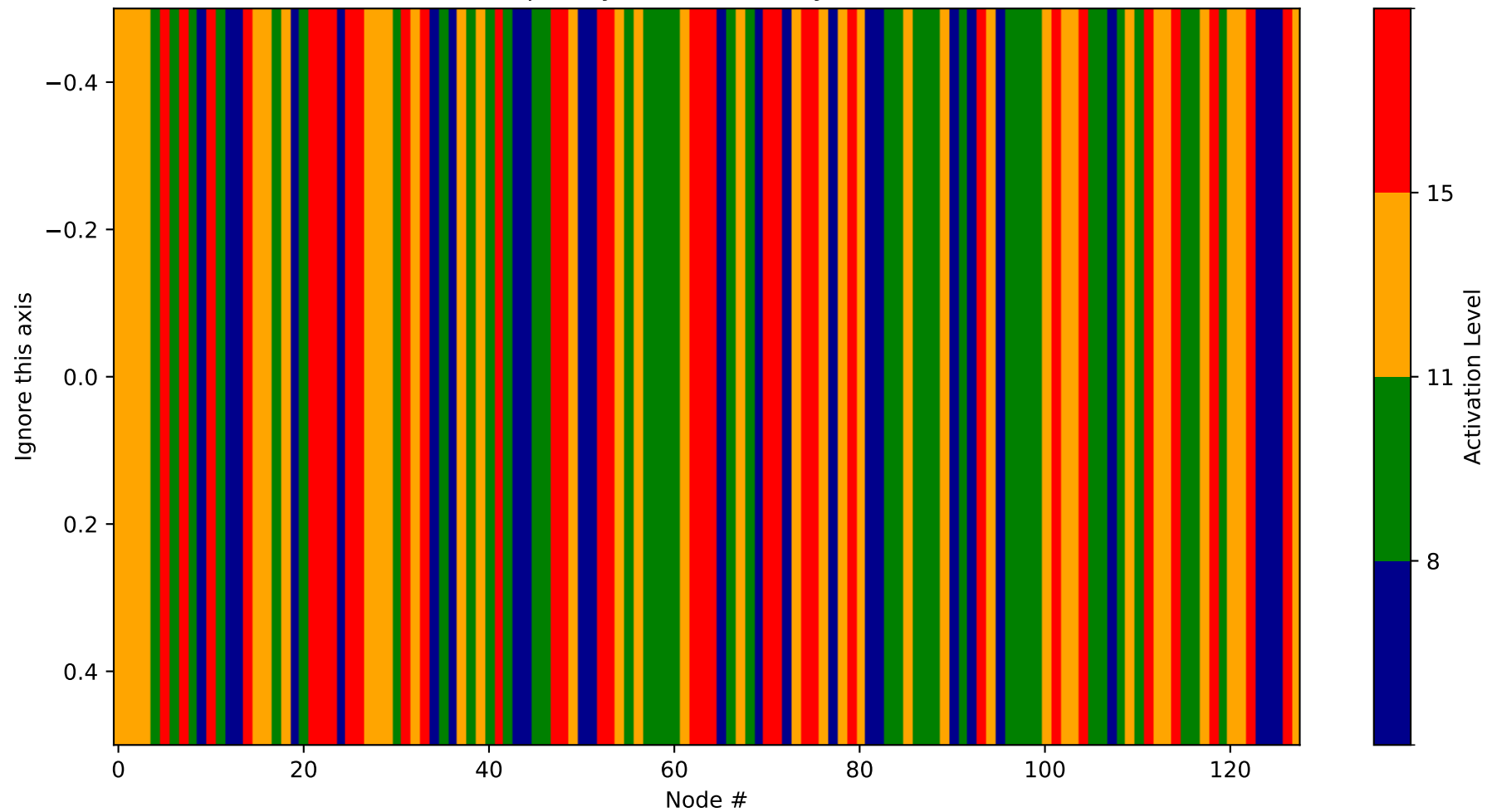
Heatmap - Layer 1 (Probability 2944-3072)
