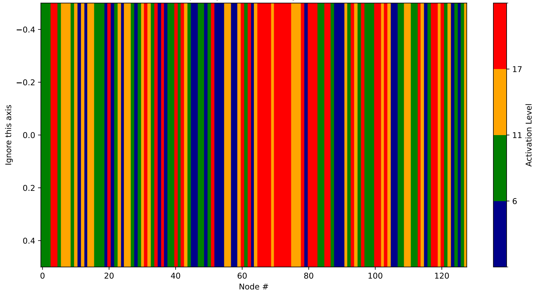
Heatmap - Layer 7 (Probability 1920-2048)
