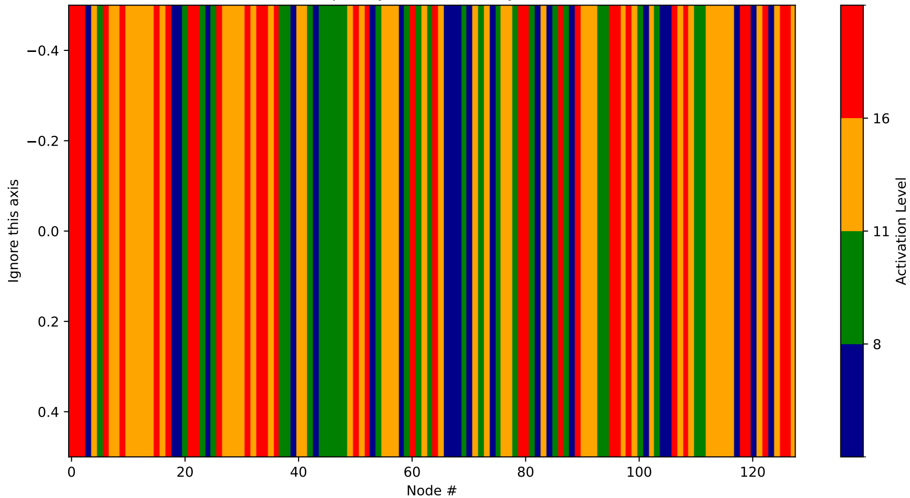
Heatmap - Layer 2 (Probability 384-512)
