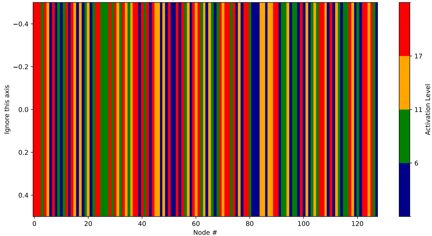
Heatmap - Layer 29 (Probability 1792-1920)
