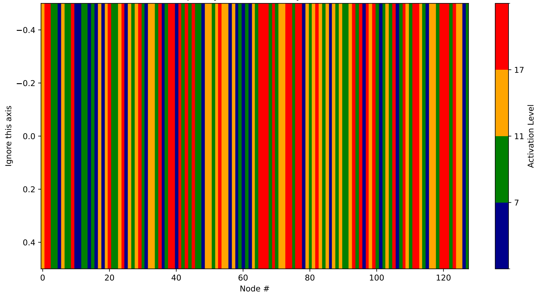
Heatmap - Layer 22 (Probability 2432-2560)
