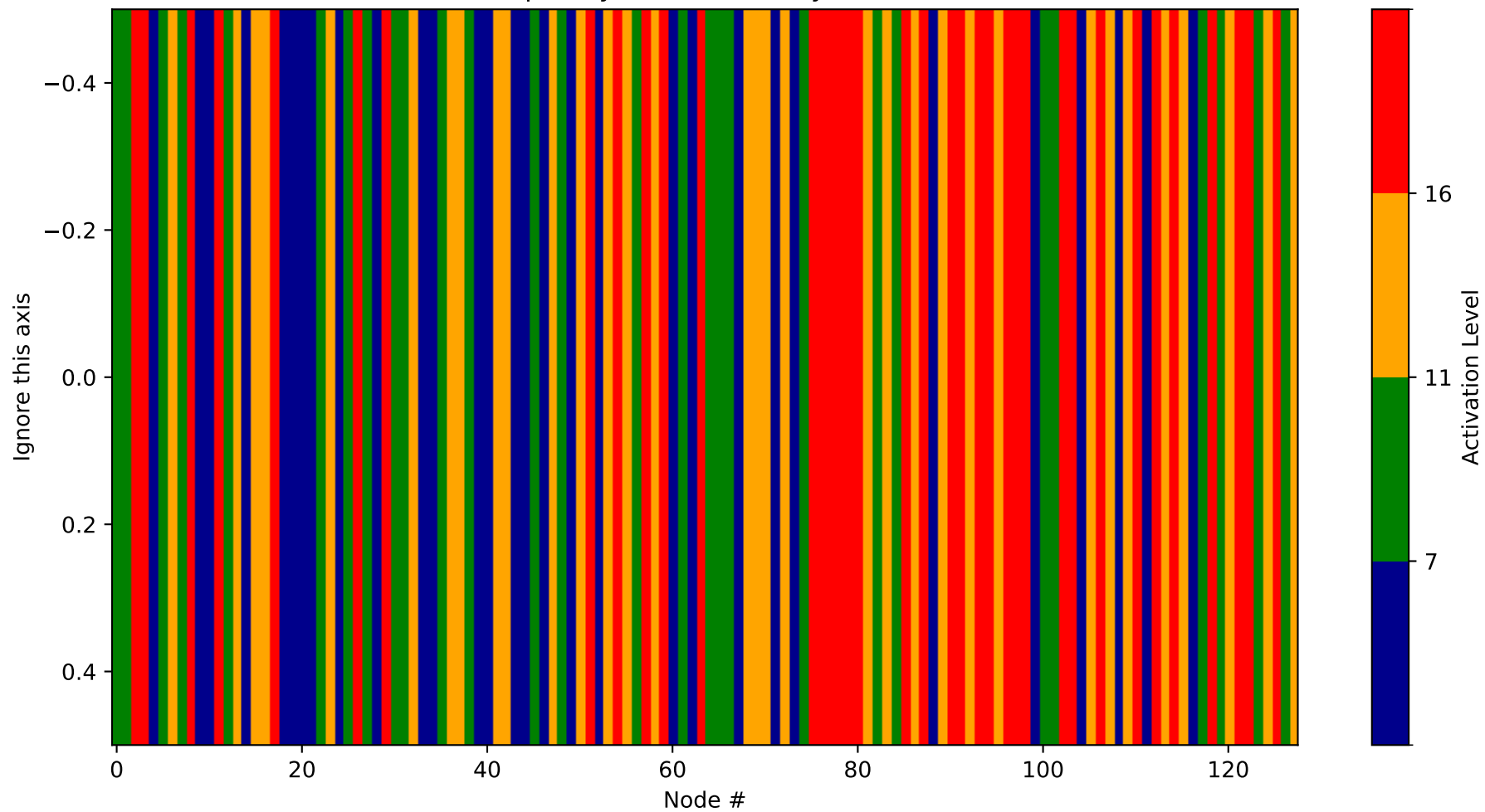
Heatmap - Layer 4 (Probability 3968-4096)
