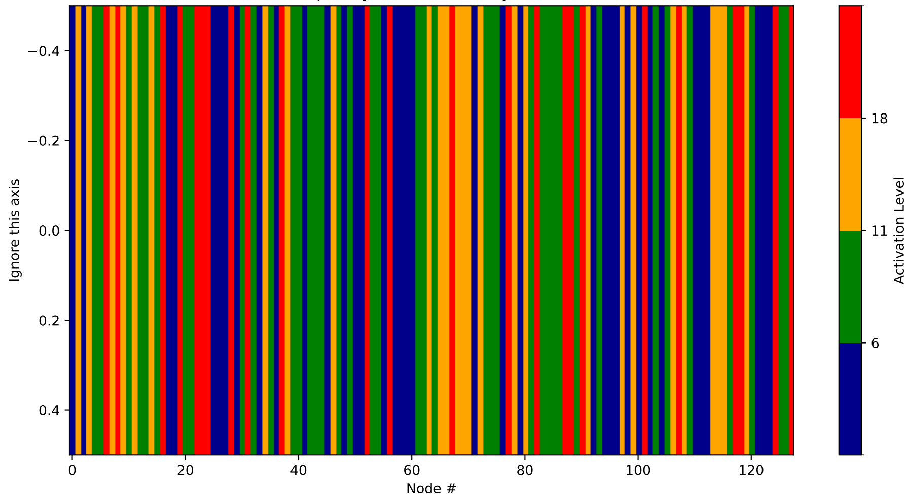
Heatmap - Layer 14 (Probability 1280-1408)
