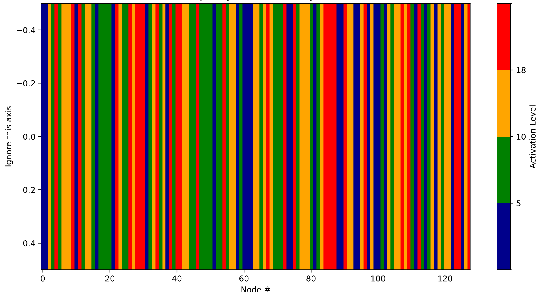
Heatmap - Layer 31 (Probability 0-128)
