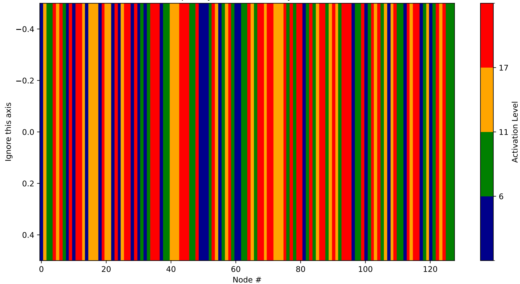
Heatmap - Layer 20 (Probability 1536-1664)
