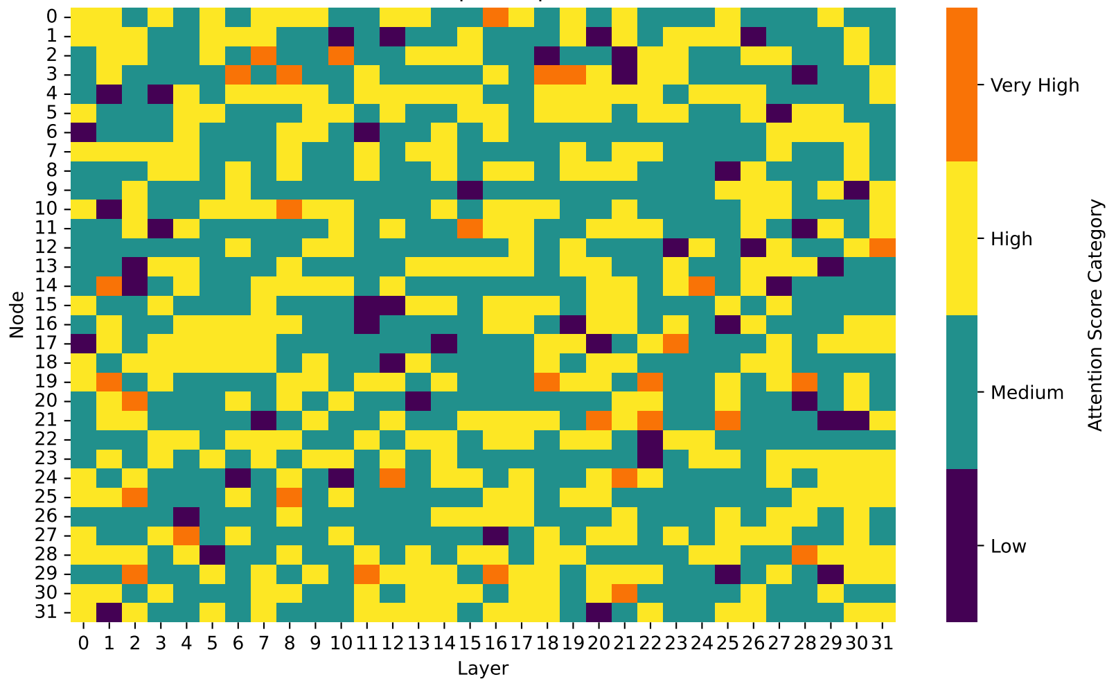
Heatmap for input 9
