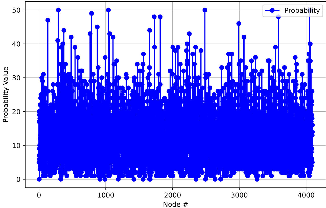
Probability Statistics Across Inputs - Layer 28
