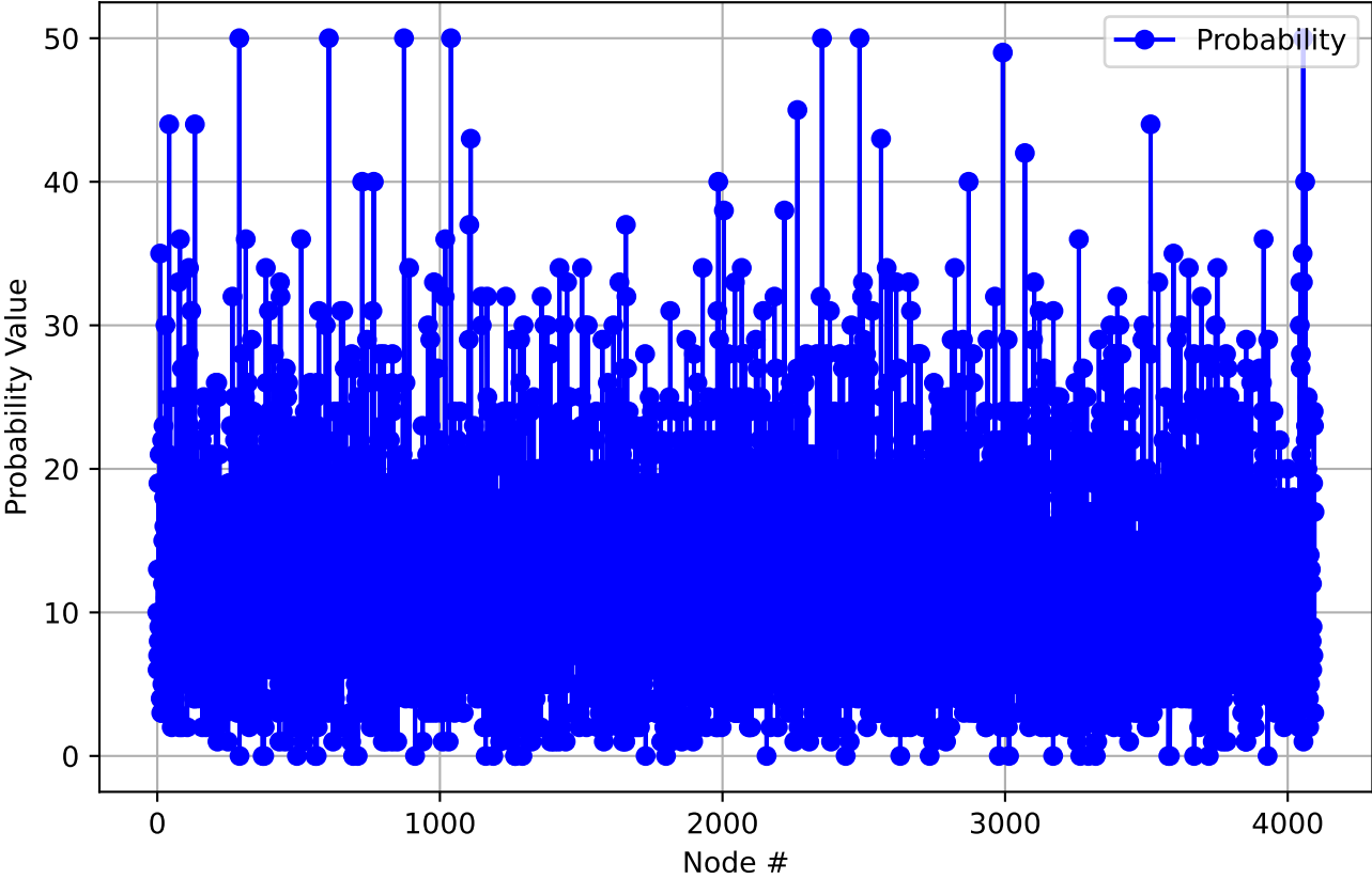
Probability Statistics Across Inputs - Layer 5
