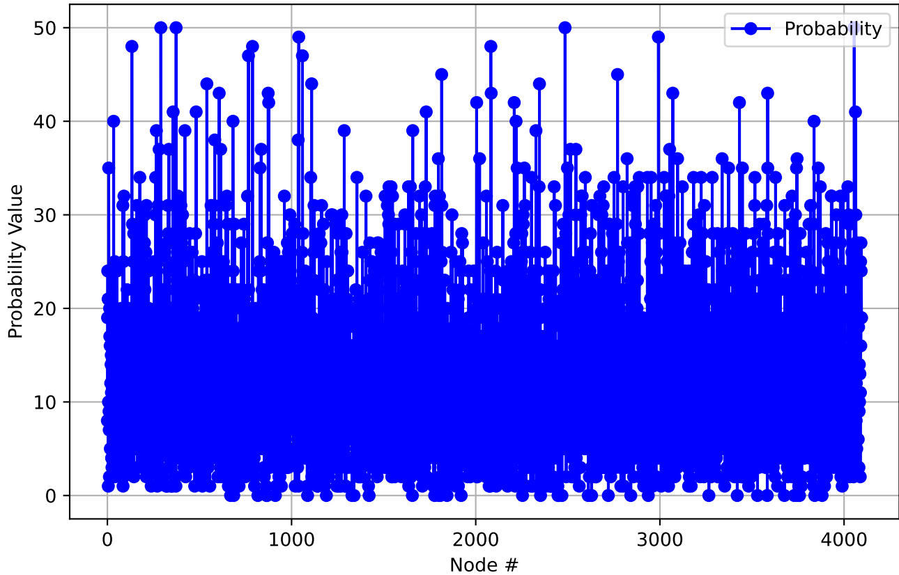
Probability Statistics Across Inputs - Layer 19
