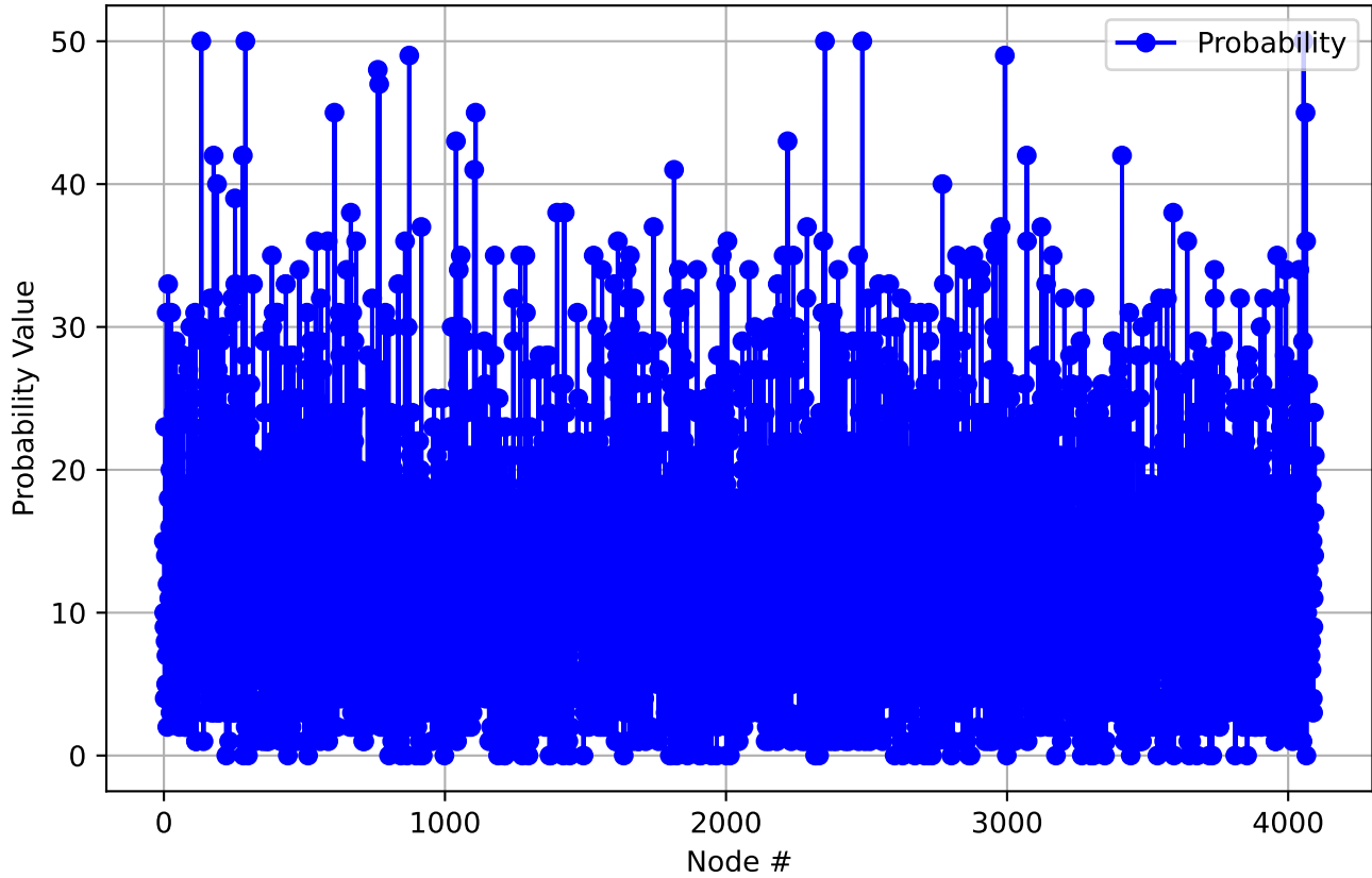
Probability Statistics Across Inputs - Layer 11
