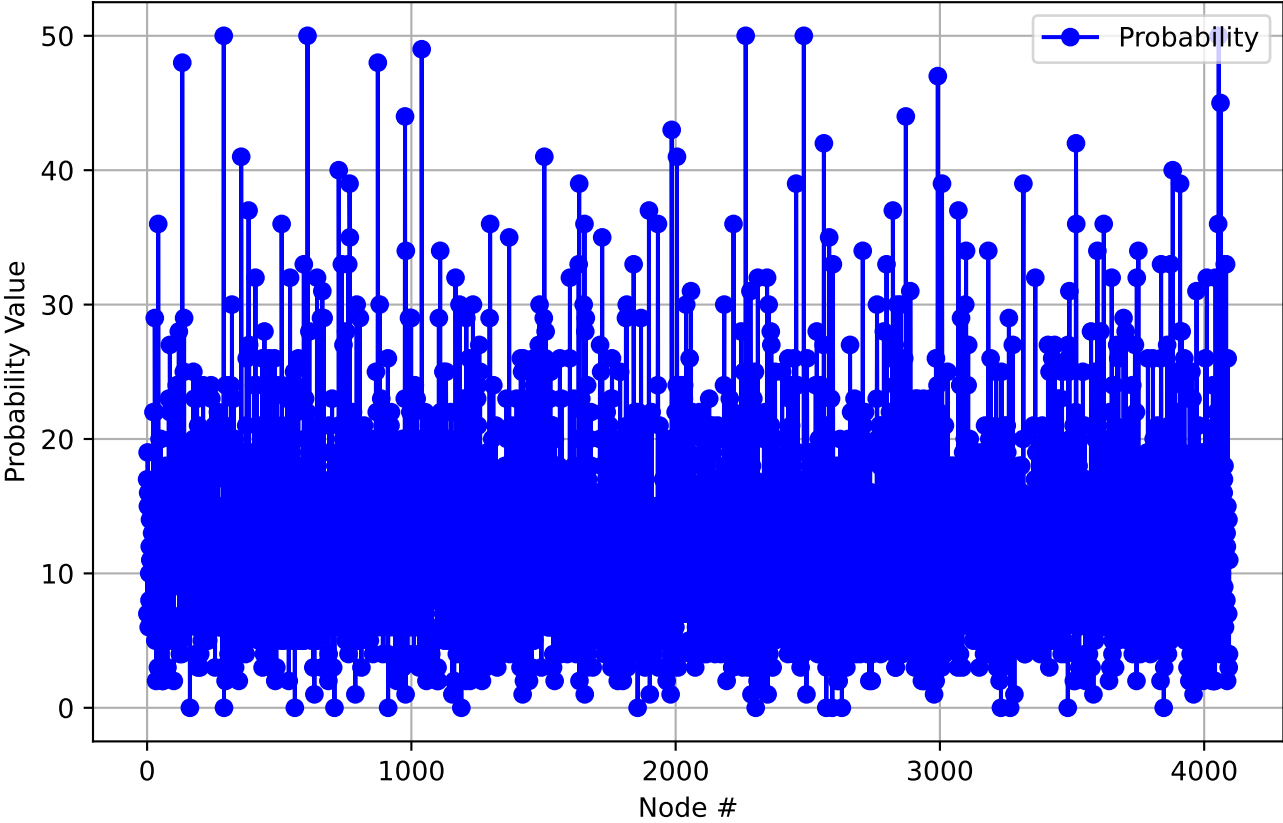
Probability Statistics Across Inputs - Layer 2
