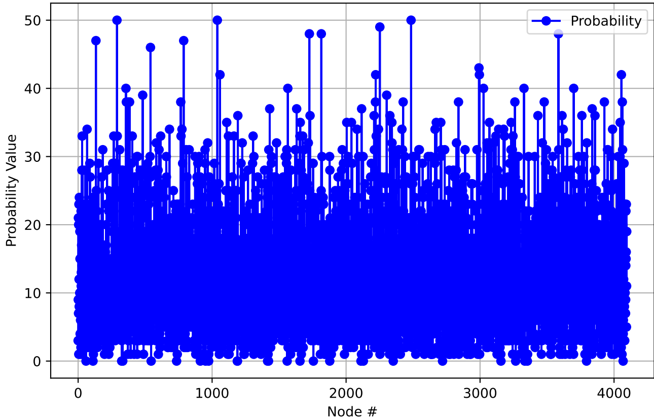
Probability Statistics Across Inputs - Layer 30
