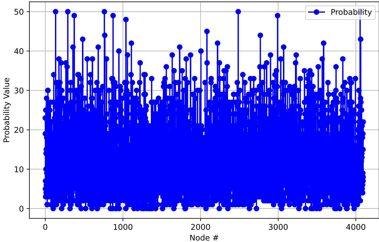
Probability Statistics Across Inputs - Layer 16
