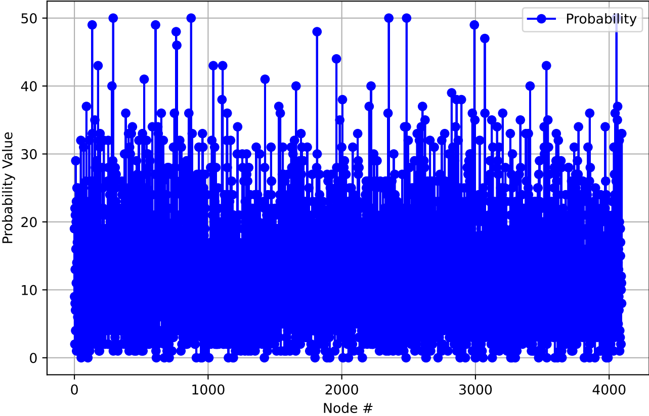
Probability Statistics Across Inputs - Layer 9
