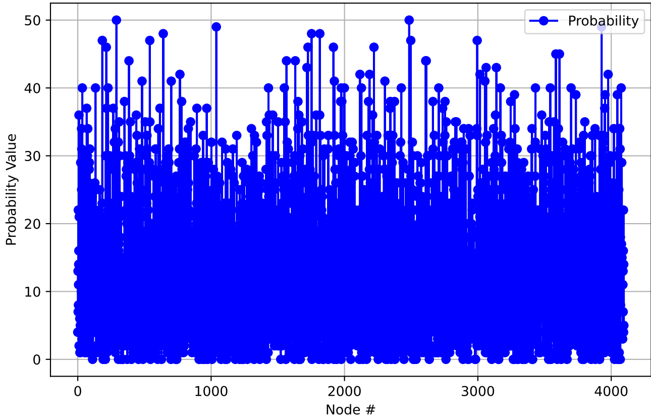
Probability Statistics Across Inputs - Layer 31
