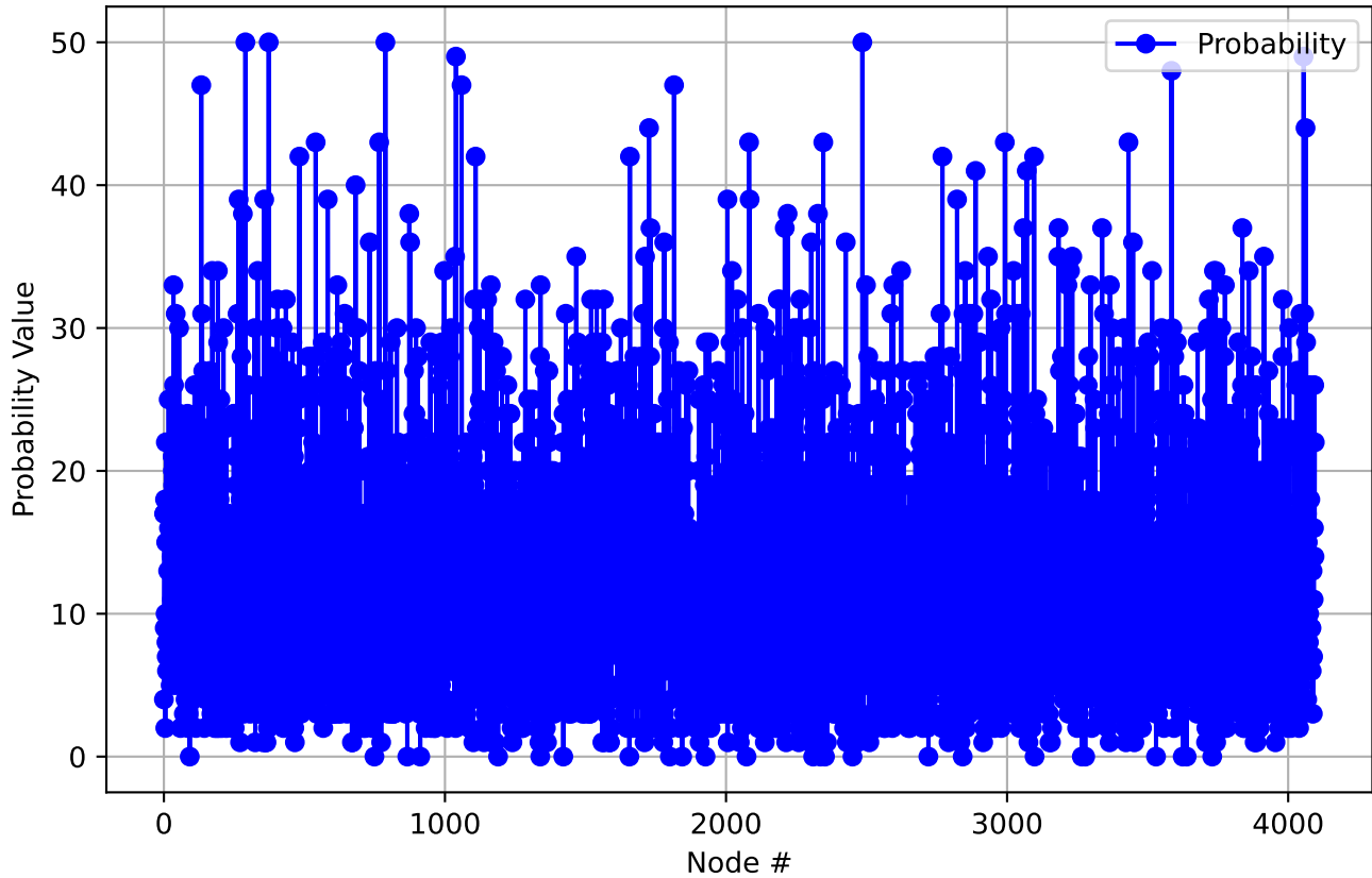
Probability Statistics Across Inputs - Layer 22
