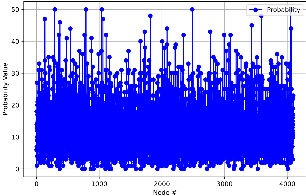
Probability Statistics Across Inputs - Layer 24
