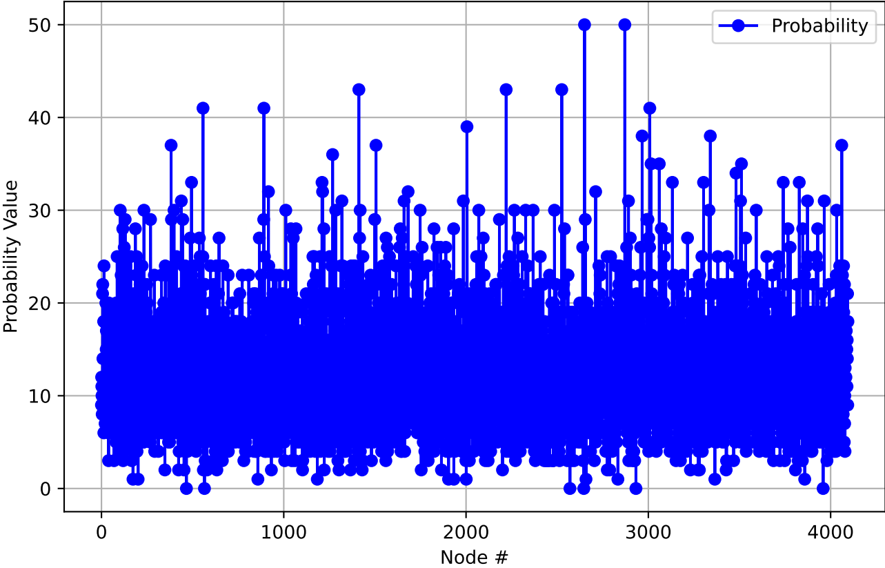
Probability Statistics Across Inputs - Layer 0
