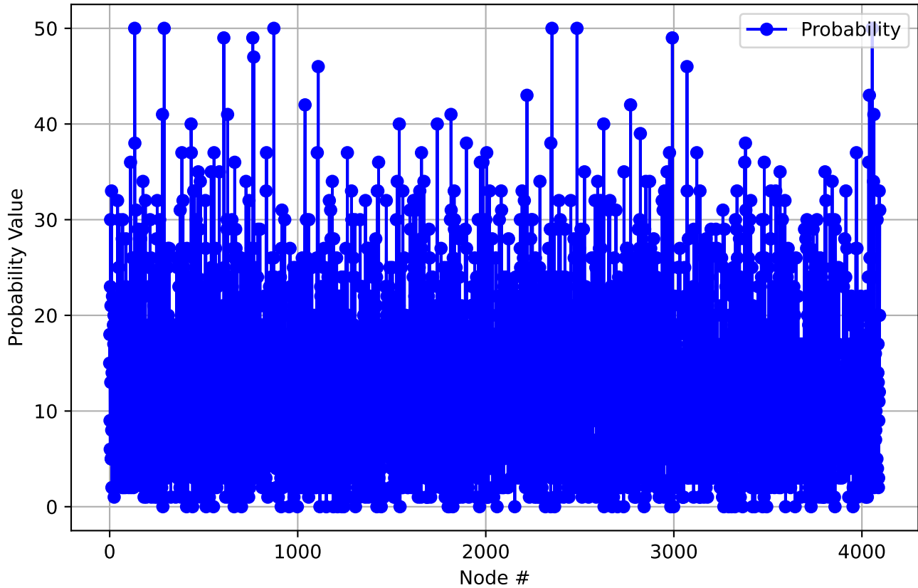
Probability Statistics Across Inputs - Layer 10
