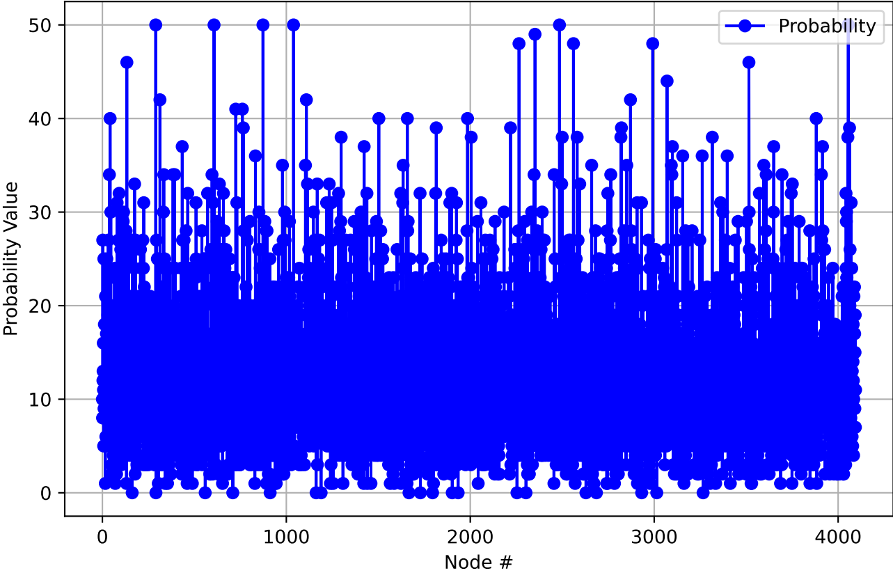
Probability Statistics Across Inputs - Layer 4
