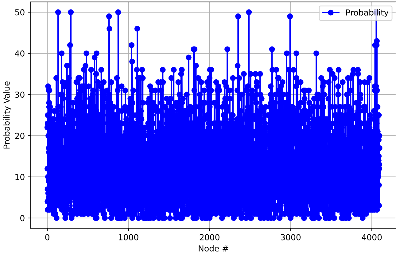
Probability Statistics Across Inputs - Layer 12
