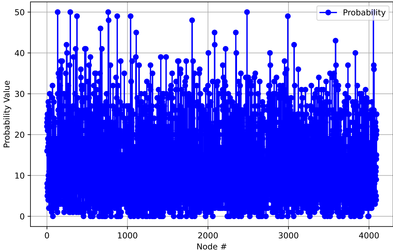
Probability Statistics Across Inputs - Layer 14
