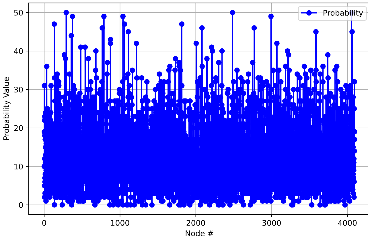
Probability Statistics Across Inputs - Layer 20
