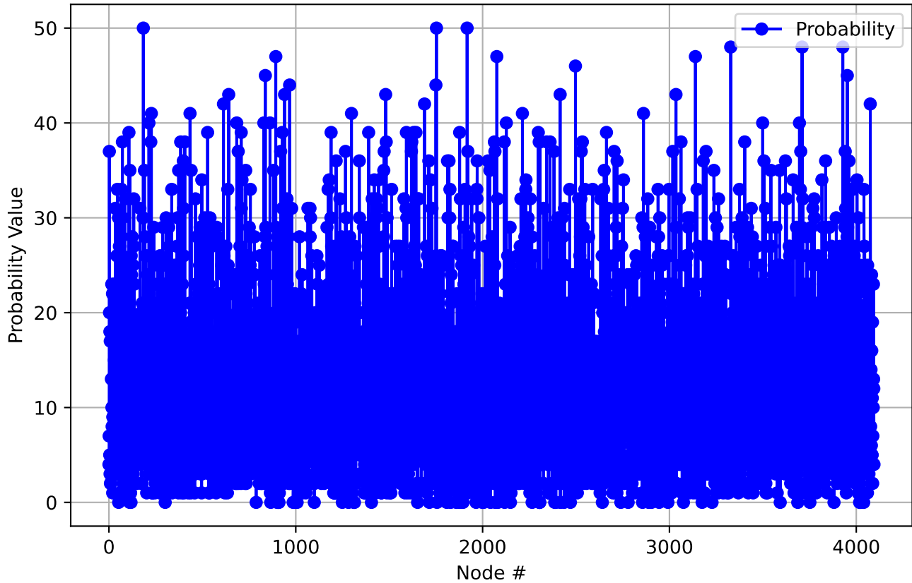
Probability Statistics Across Inputs - Layer 32
