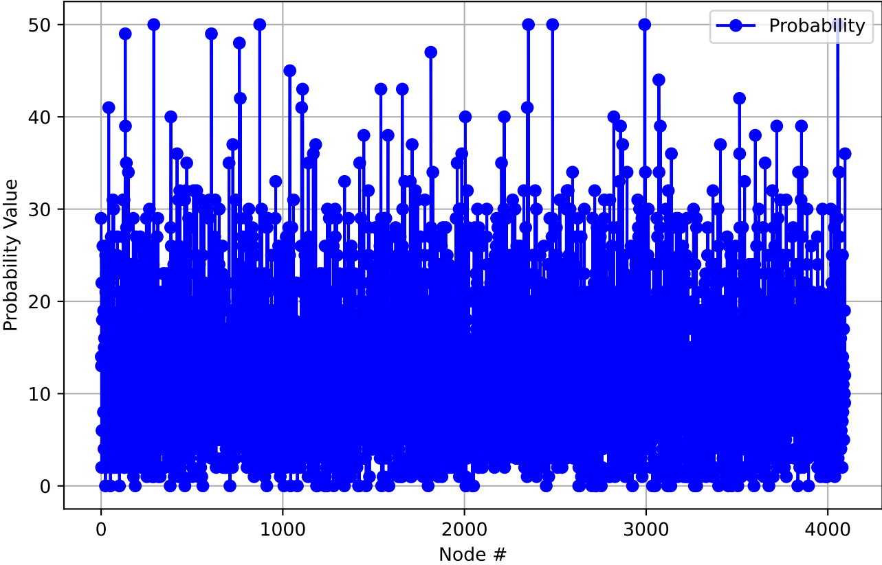
Probability Statistics Across Inputs - Layer 8
