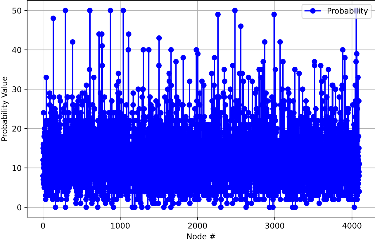
Probability Statistics Across Inputs - Layer 3
