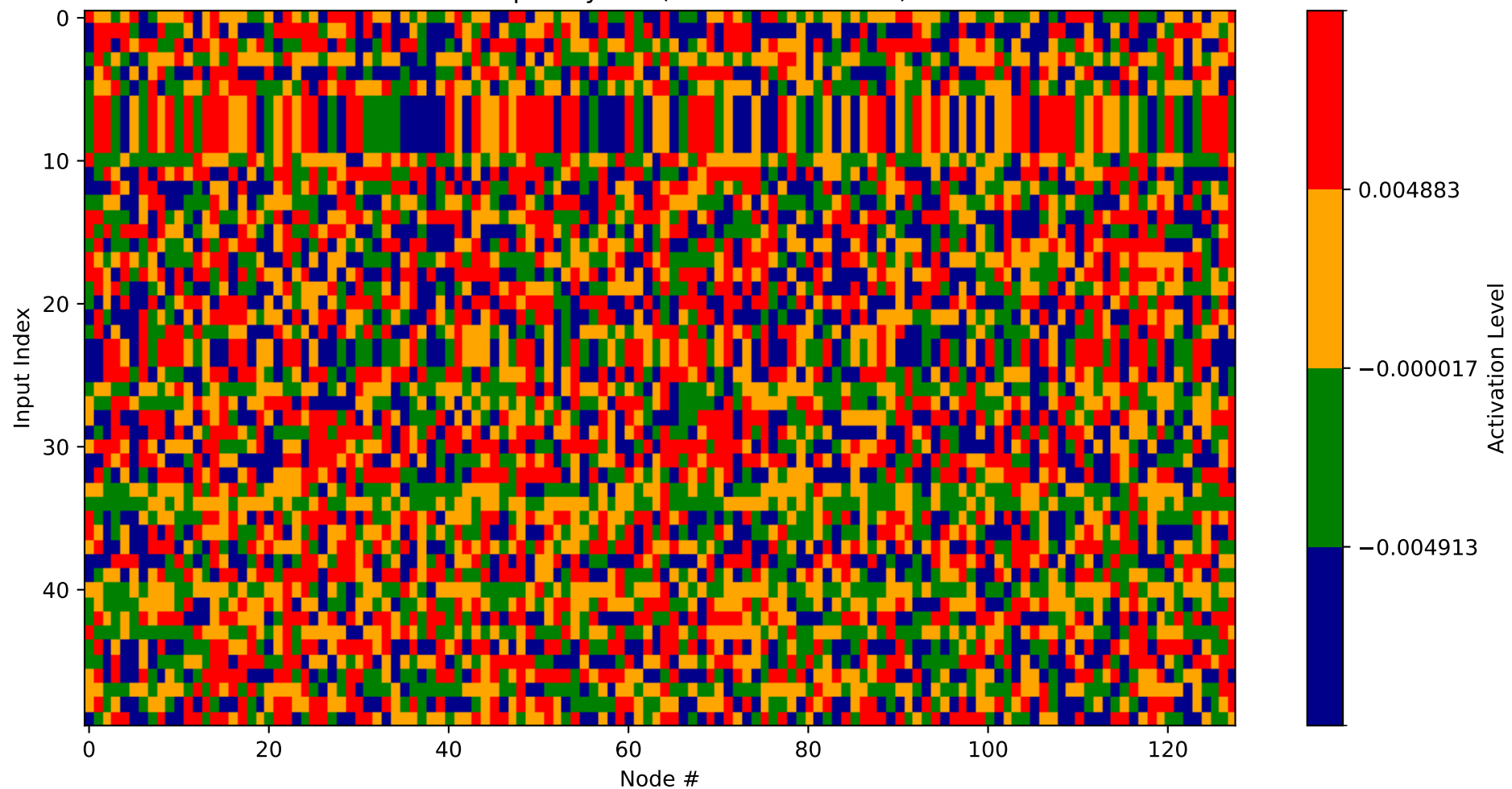
Heatmap - Layer 0 (Nodes 2944-3072)
