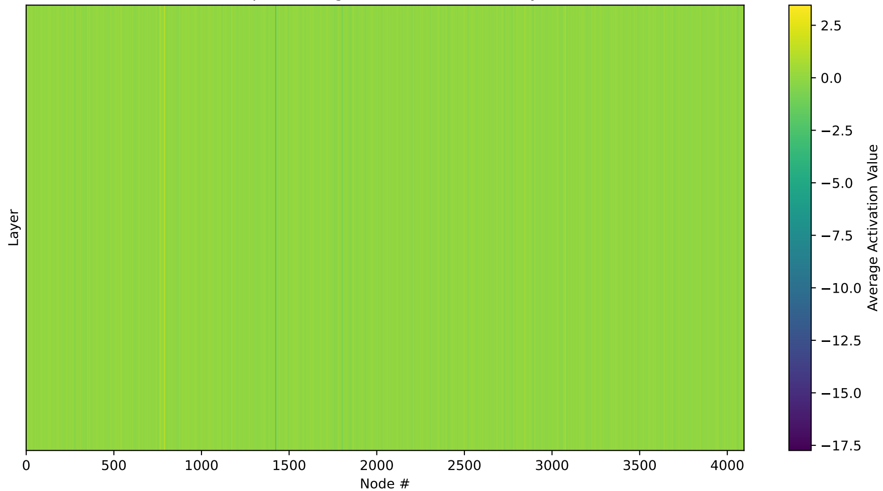
Heatmap of Average Node Activations - Layer 28
