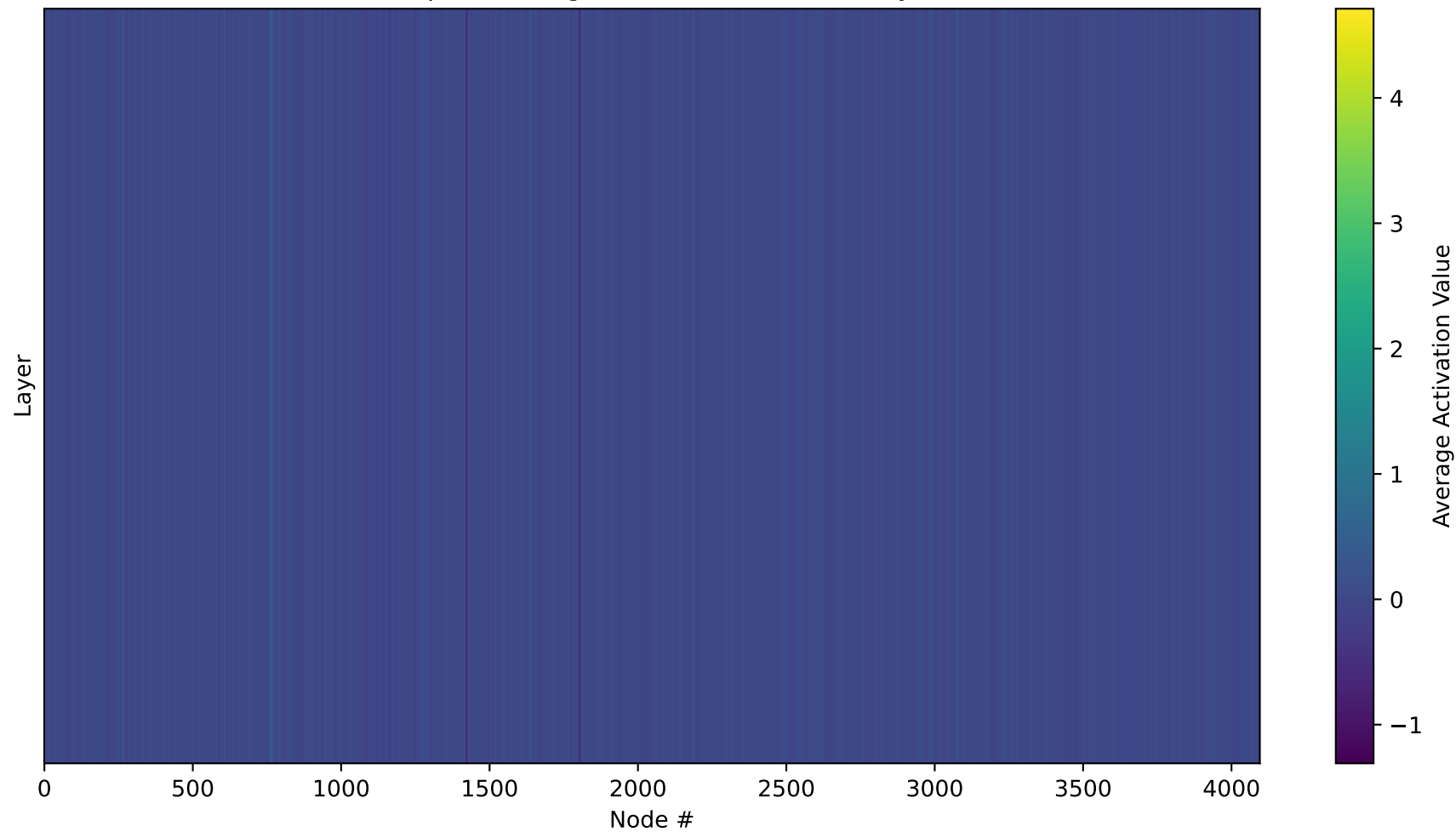
Heatmap of Average Node Activations - Layer 16
