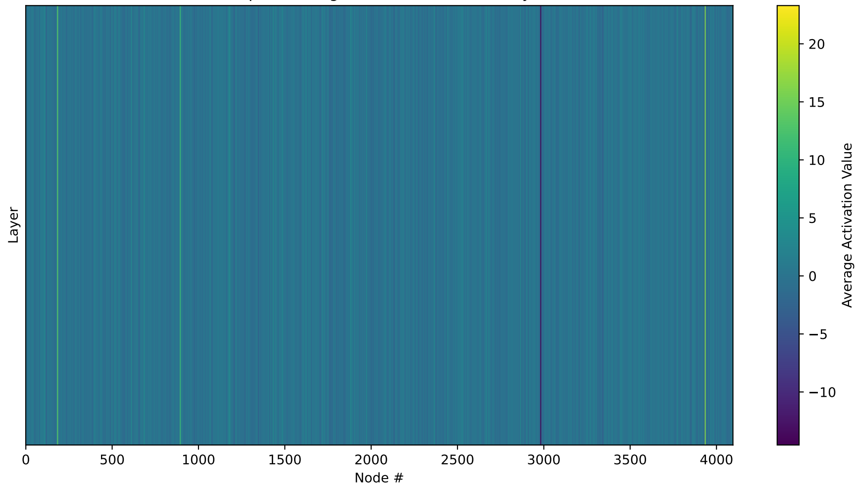
Heatmap of Average Node Activations - Layer 32
