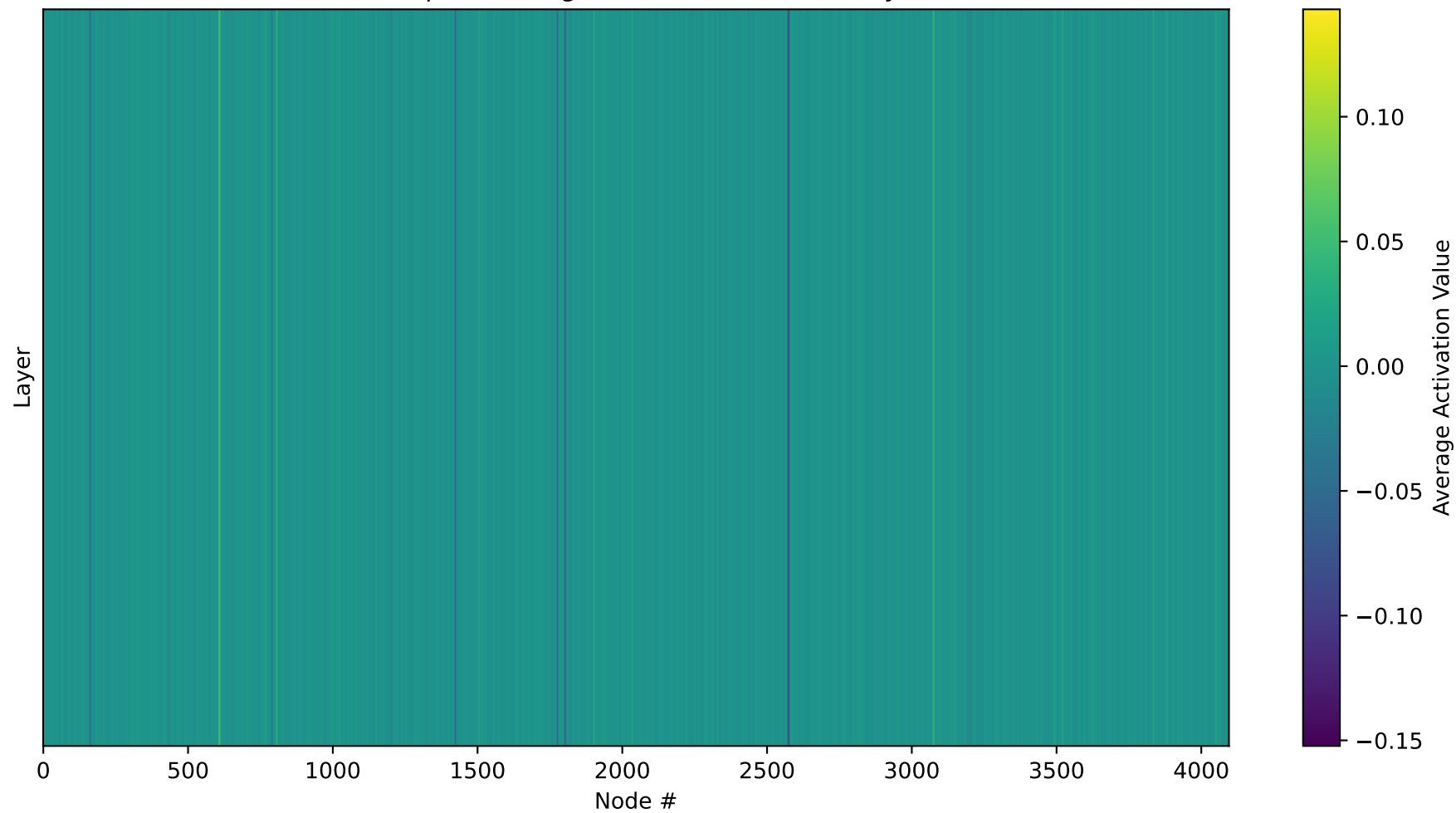
Heatmap of Average Node Activations - Layer 1
