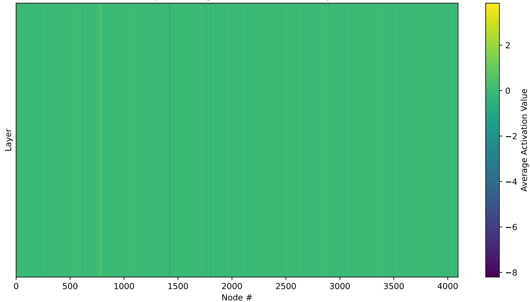
Heatmap of Average Node Activations - Layer 23
