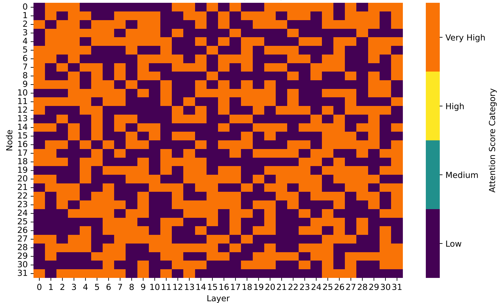
Heatmap of probability for logical
