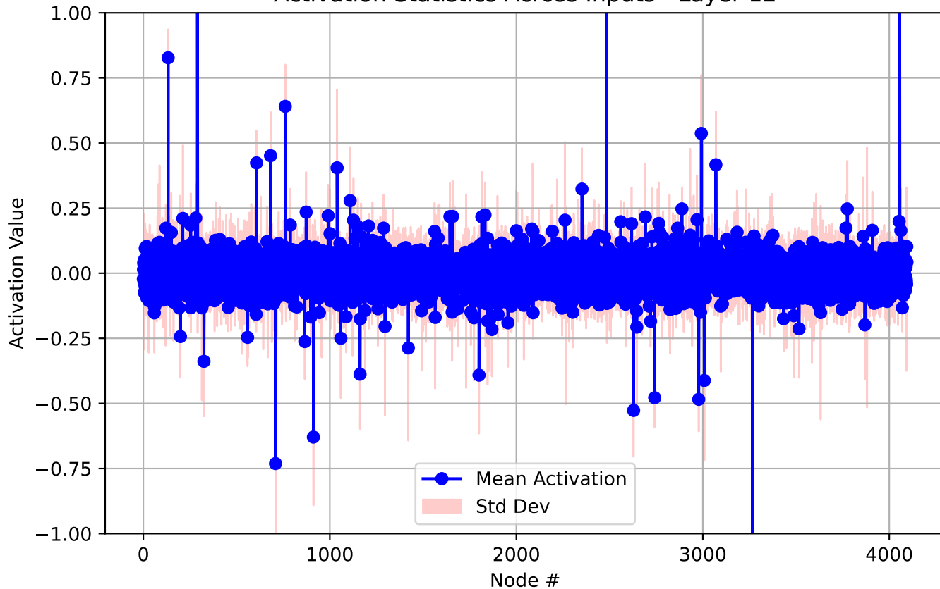
Activation Statistics Across Inputs - Layer 12
