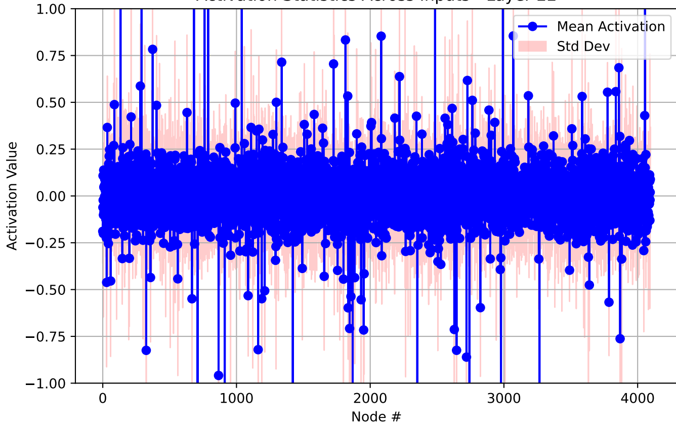
Activation Statistics Across Inputs - Layer 22
