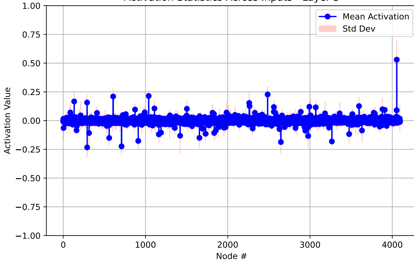
Activation Statistics Across Inputs - Layer 3
