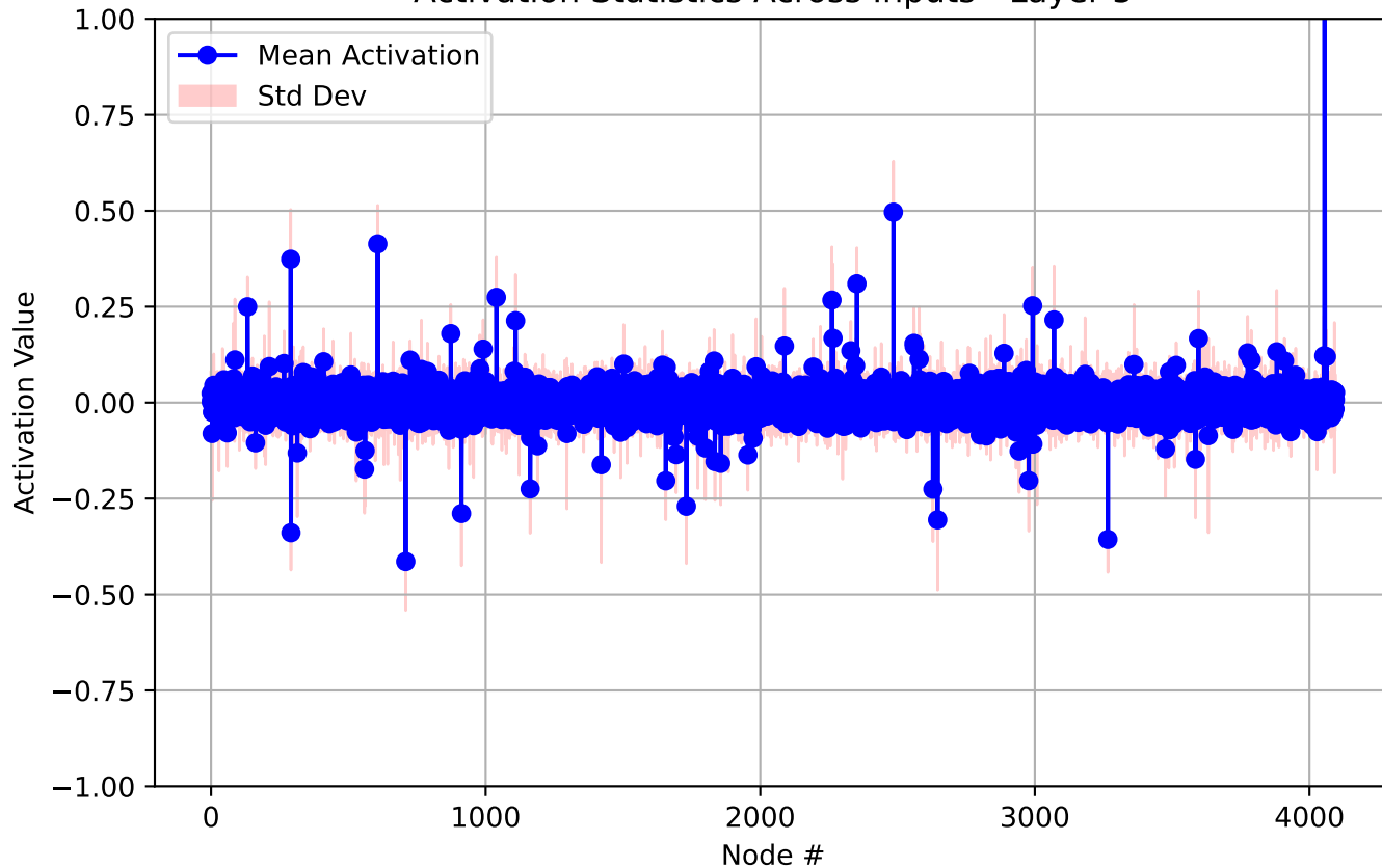
Activation Statistics Across Inputs - Layer 5
