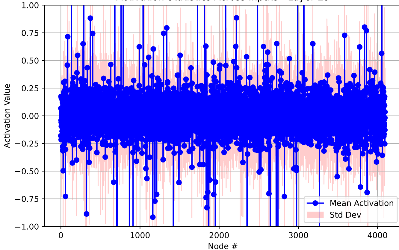
Activation Statistics Across Inputs - Layer 25
