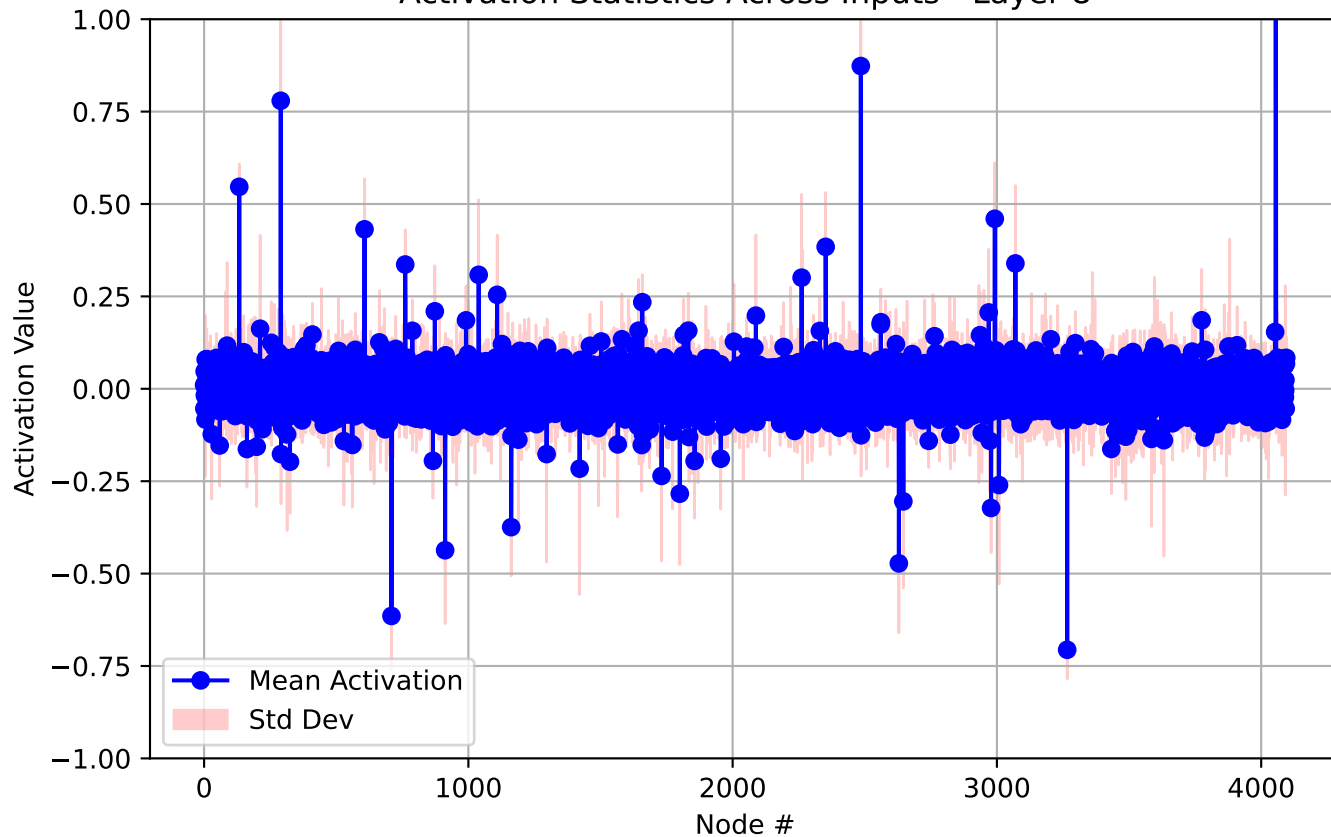
Activation Statistics Across Inputs - Layer 8
