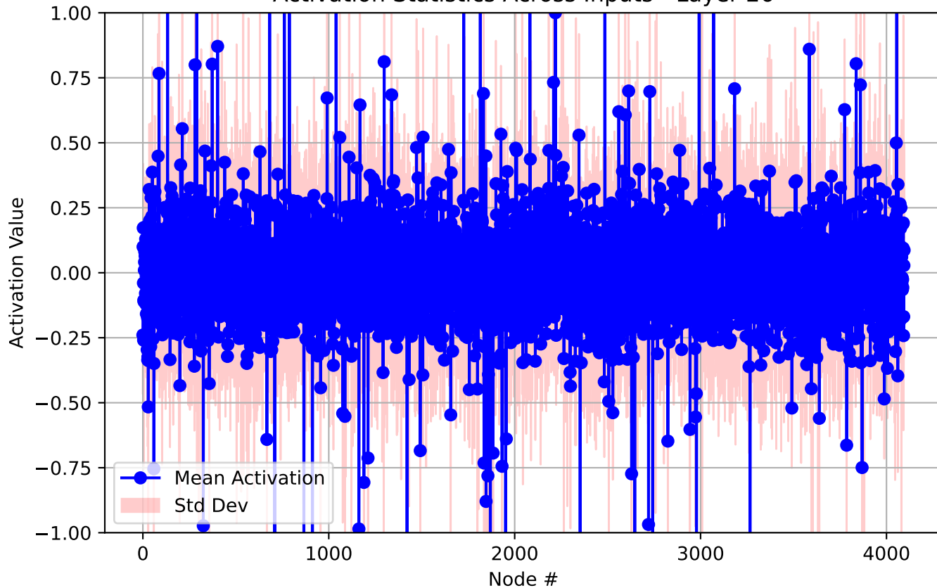
Activation Statistics Across Inputs - Layer 26
