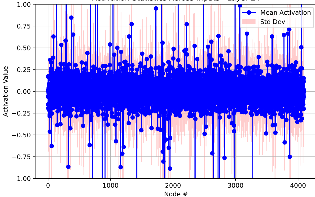
Activation Statistics Across Inputs - Layer 24
