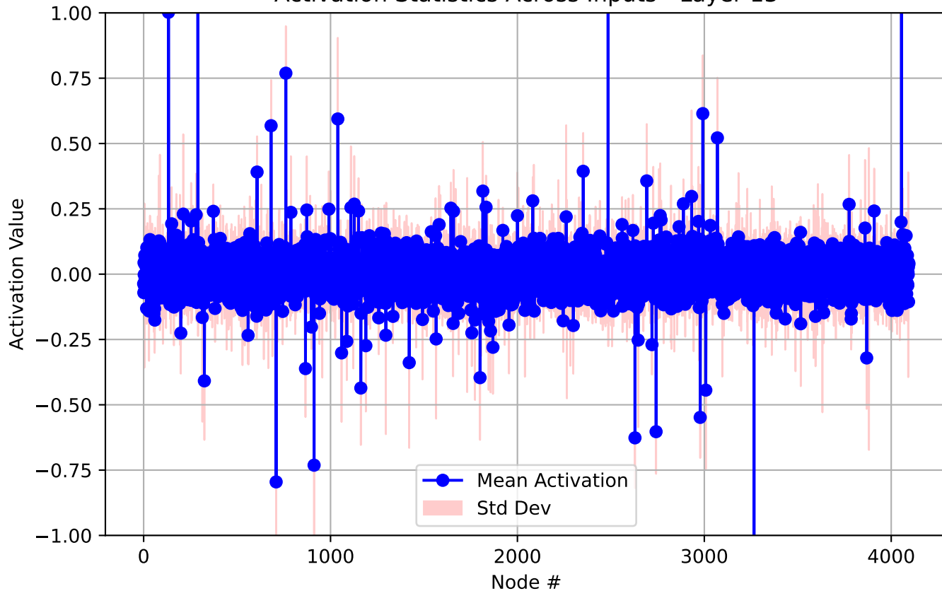
Activation Statistics Across Inputs - Layer 13
