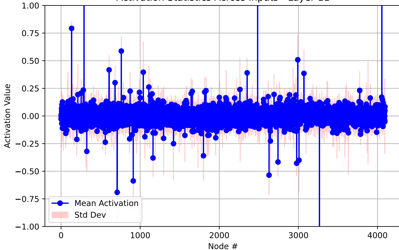
Activation Statistics Across Inputs - Layer 11
