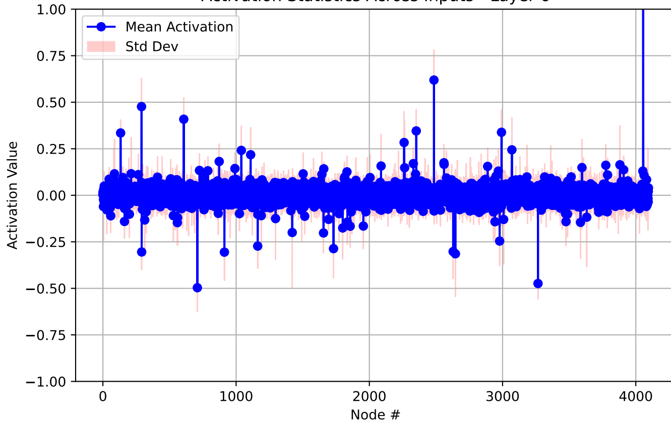
Activation Statistics Across Inputs - Layer 6
