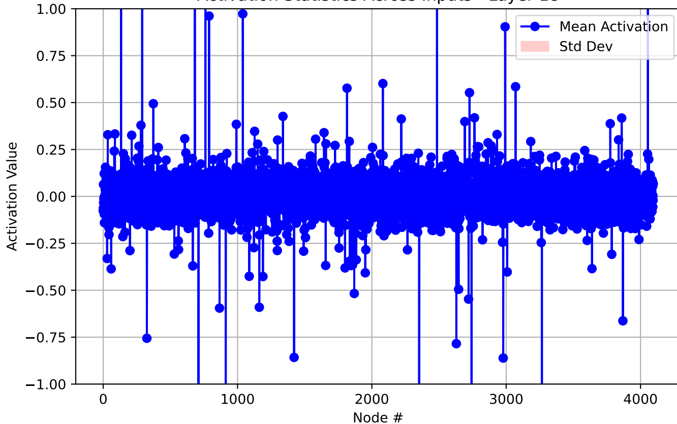
Activation Statistics Across Inputs - Layer 18
