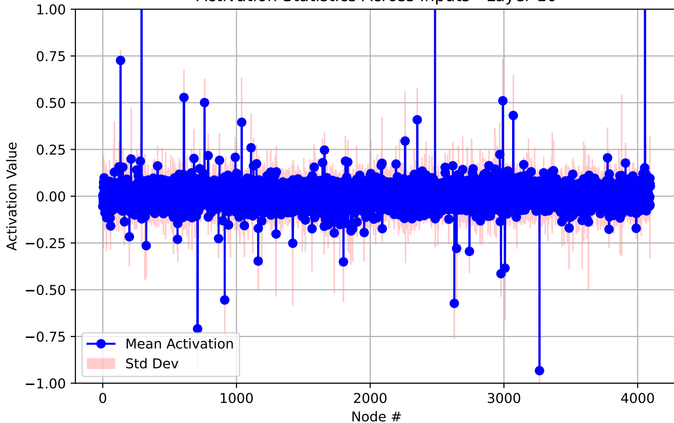
Activation Statistics Across Inputs - Layer 10
