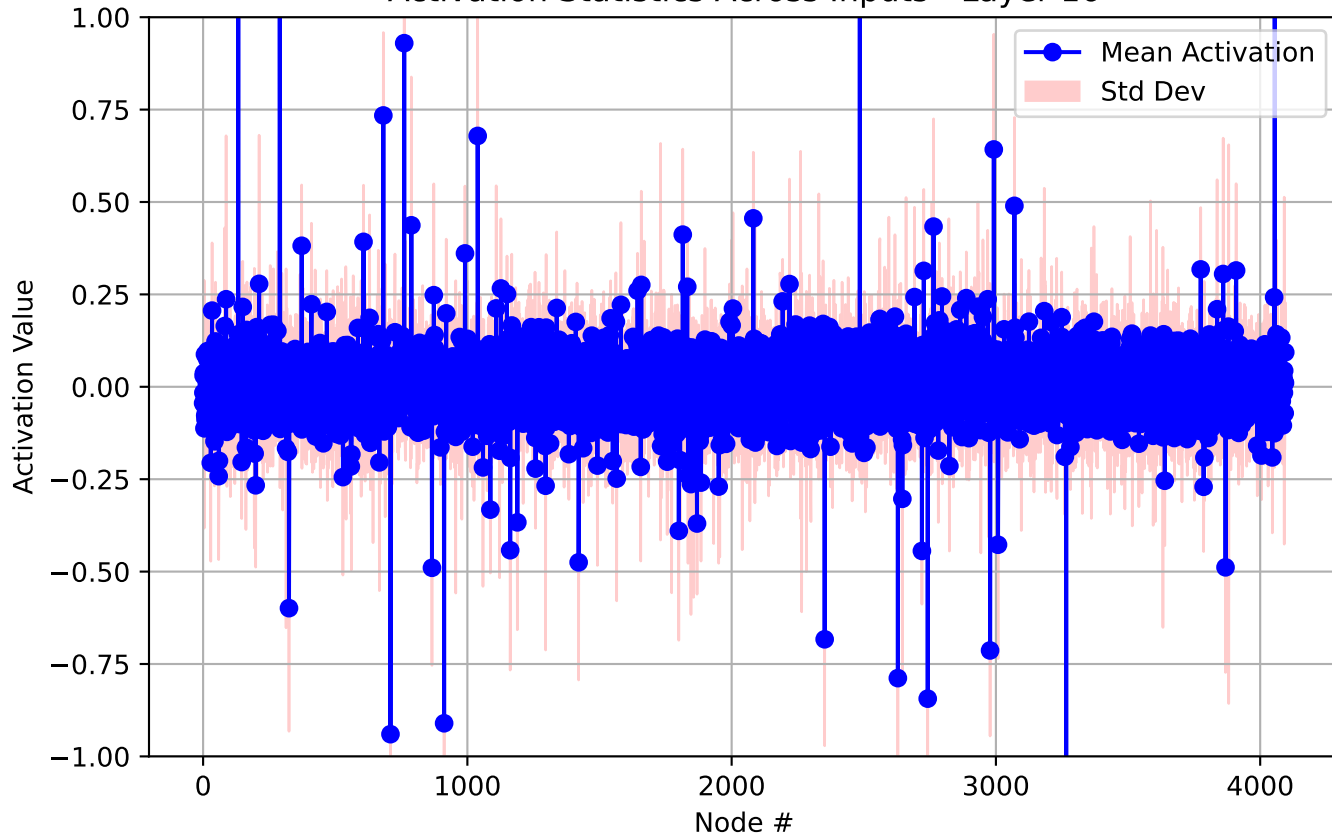
Activation Statistics Across Inputs - Layer 16
