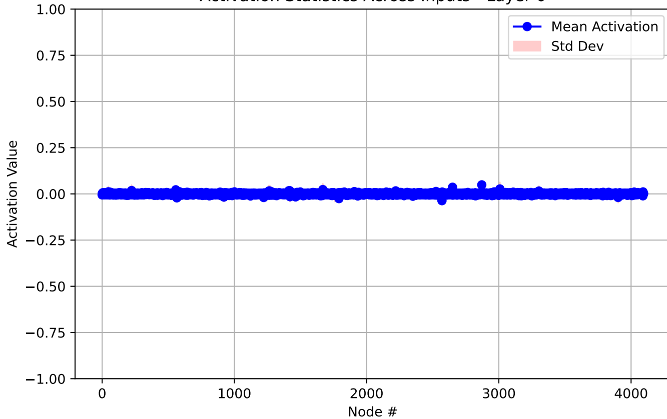
Activation Statistics Across Inputs - Layer 0
