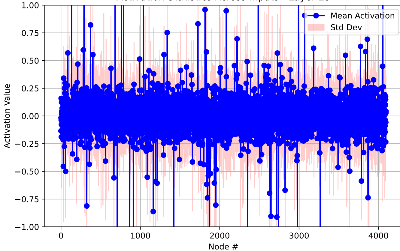
Activation Statistics Across Inputs - Layer 23
