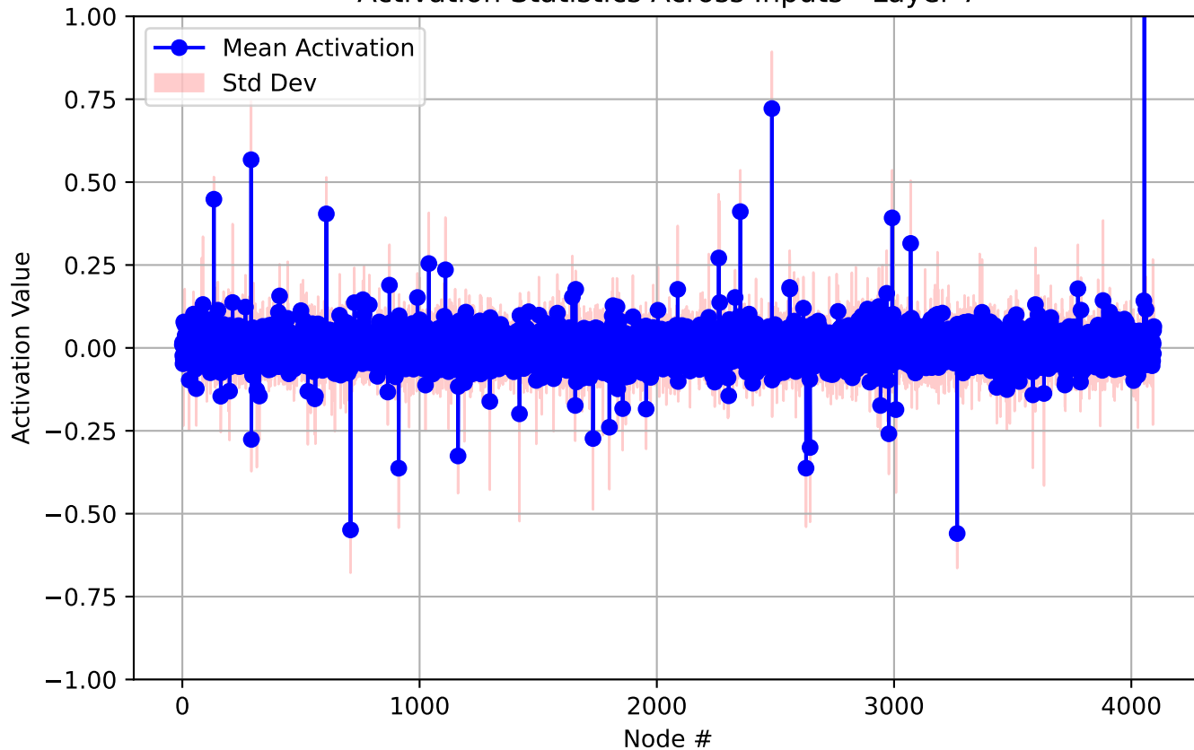
Activation Statistics Across Inputs - Layer 7
