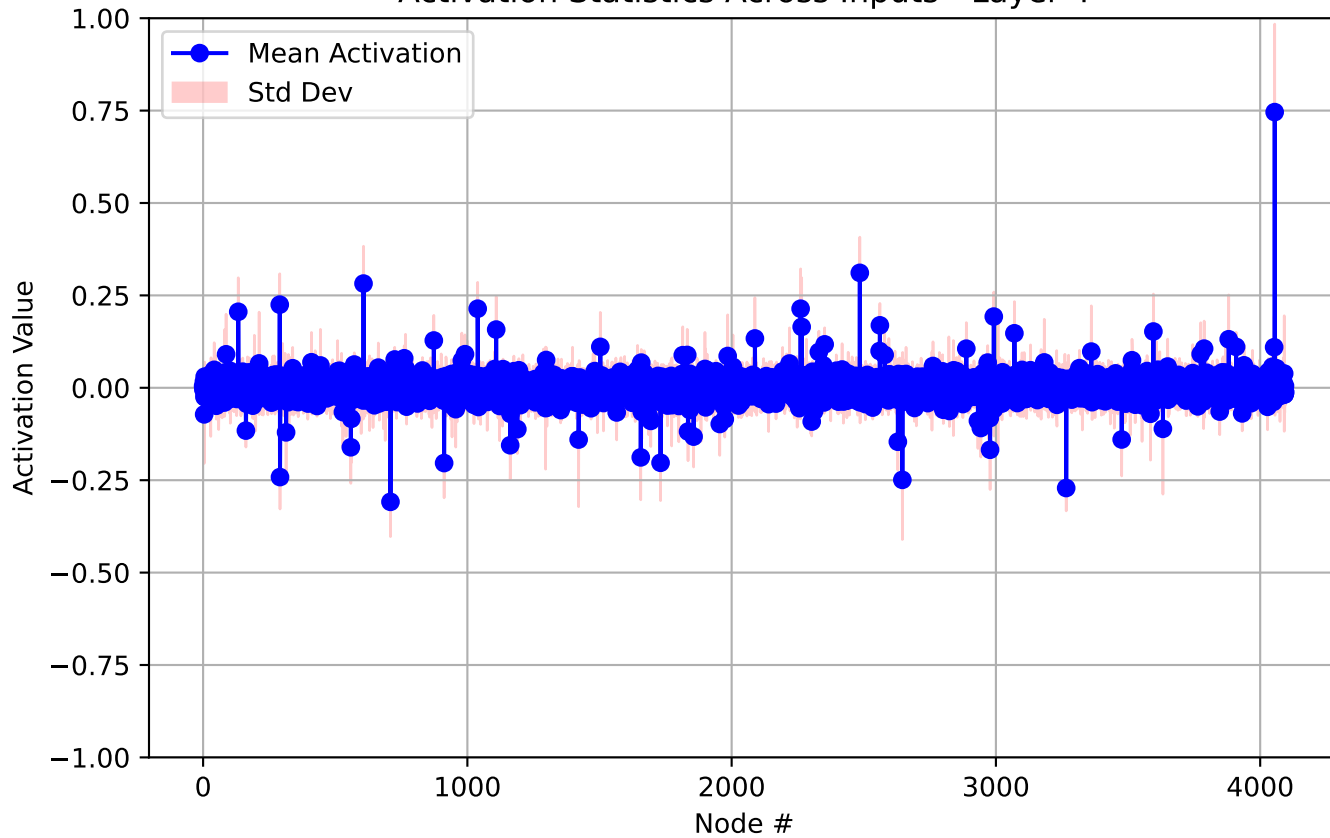
Activation Statistics Across Inputs - Layer 4
