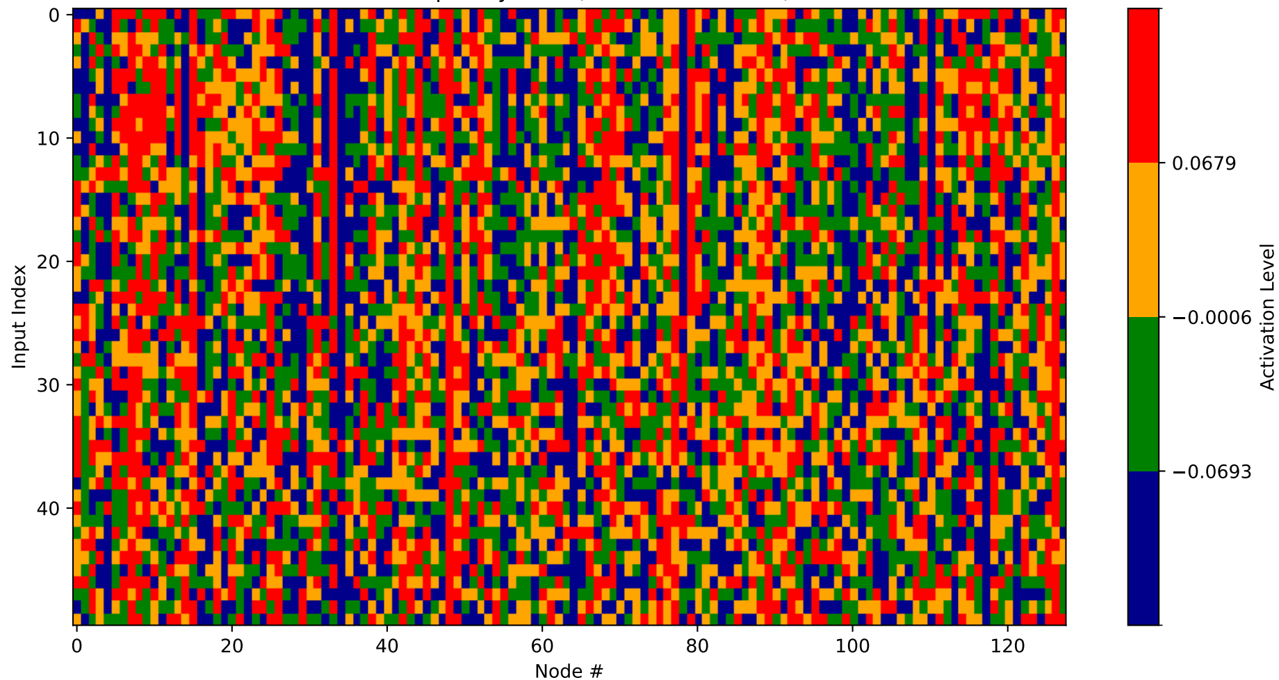
Heatmap - Layer 14 (Nodes 2944-3072)
