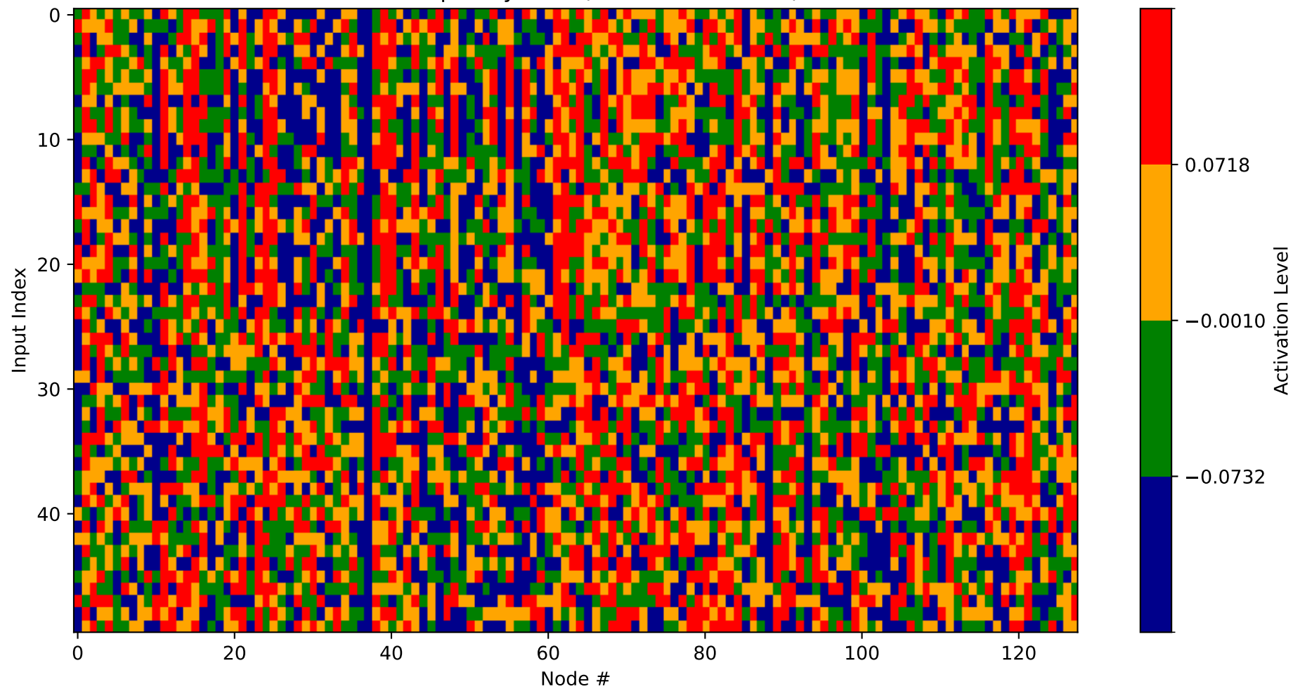
Heatmap - Layer 15 (Nodes 1152-1280)
