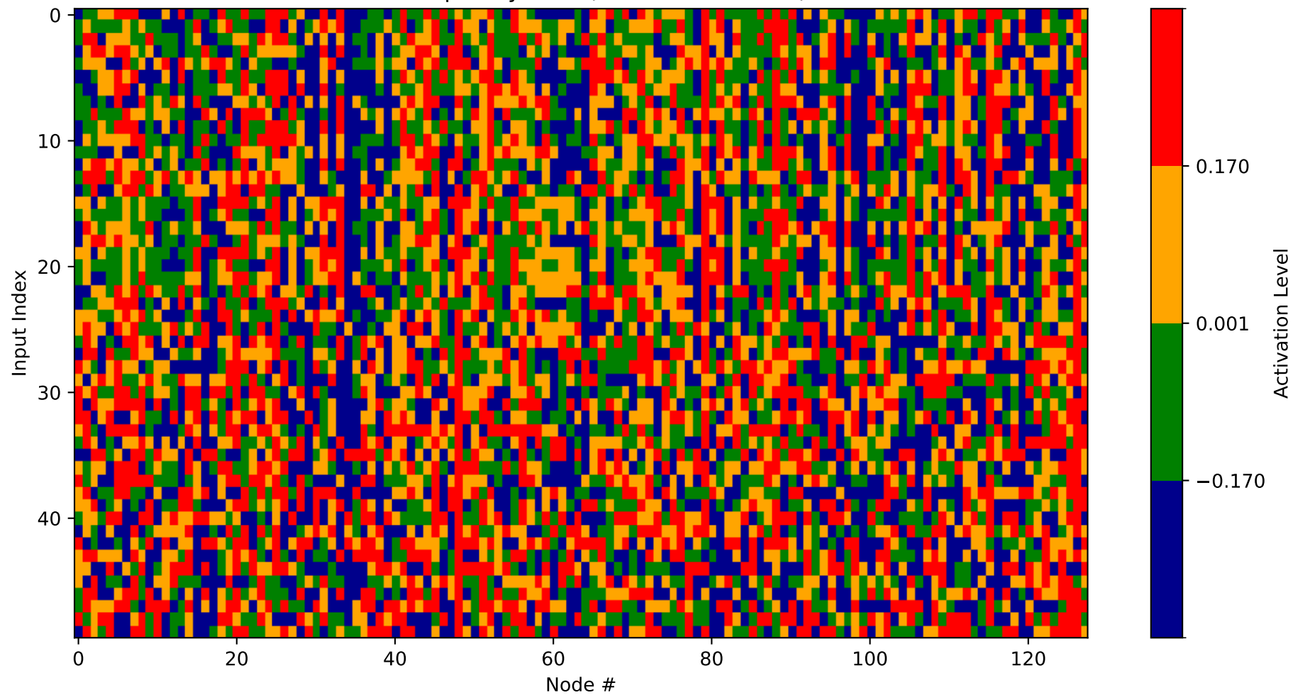
Heatmap - Layer 24 (Nodes 2944-3072)
