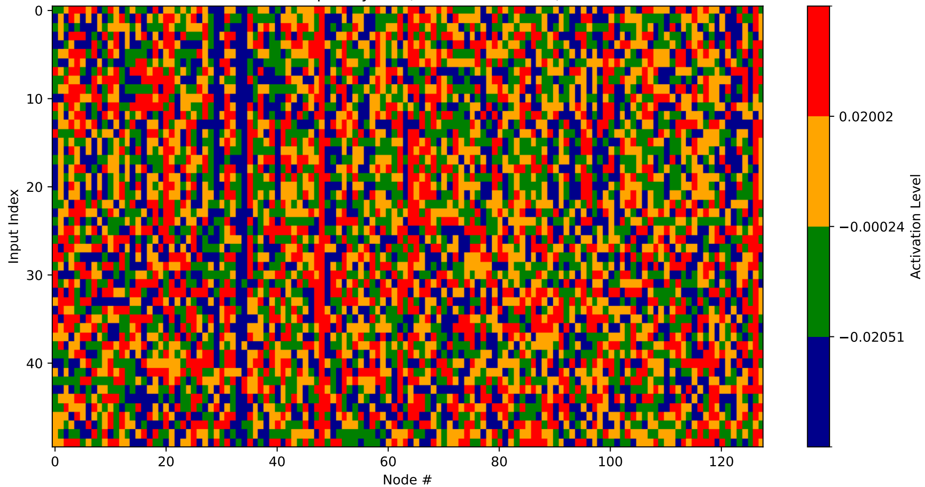
Heatmap - Layer 3 (Nodes 2944-3072)
