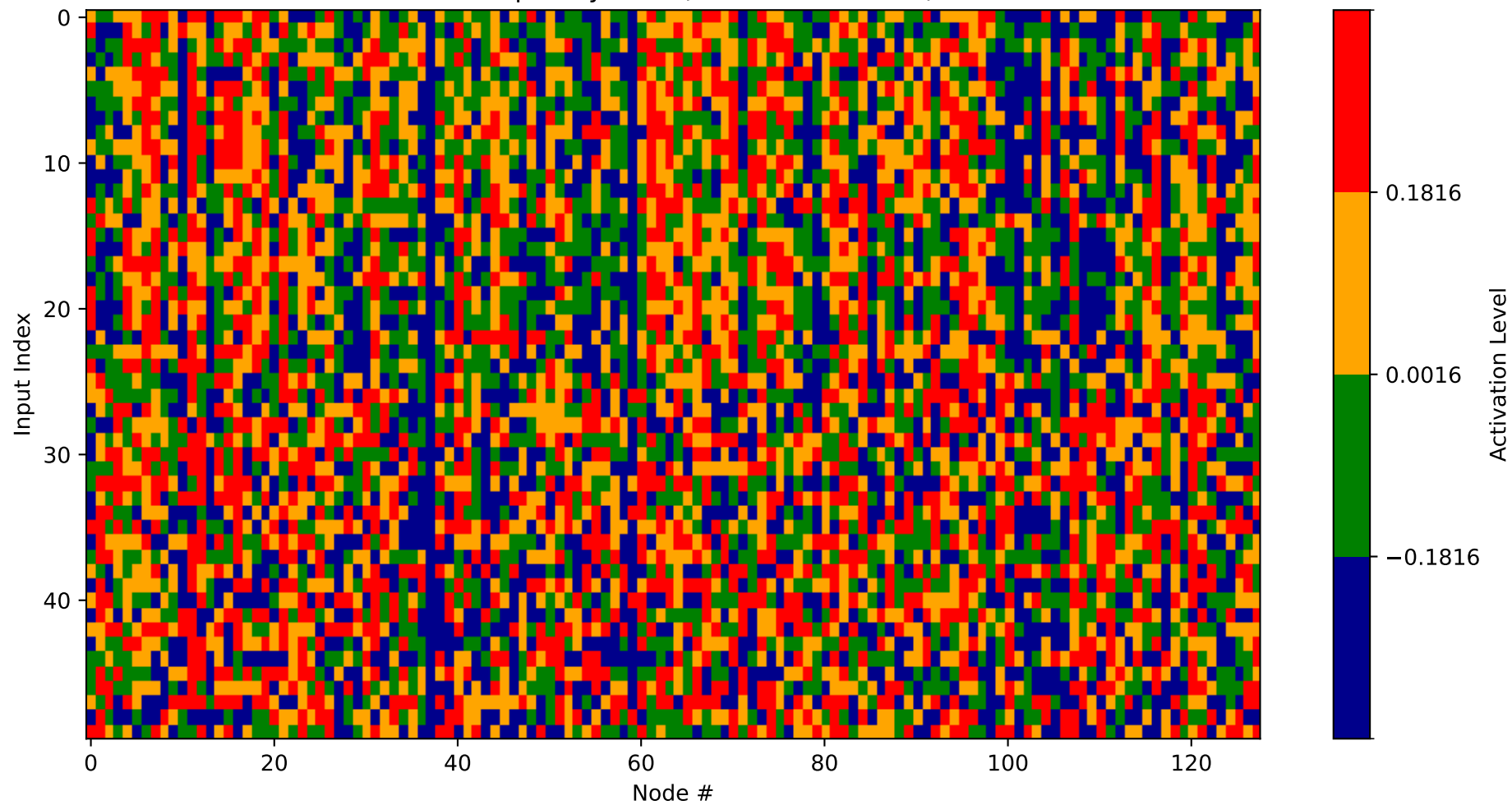
Heatmap - Layer 25 (Nodes 1152-1280)
