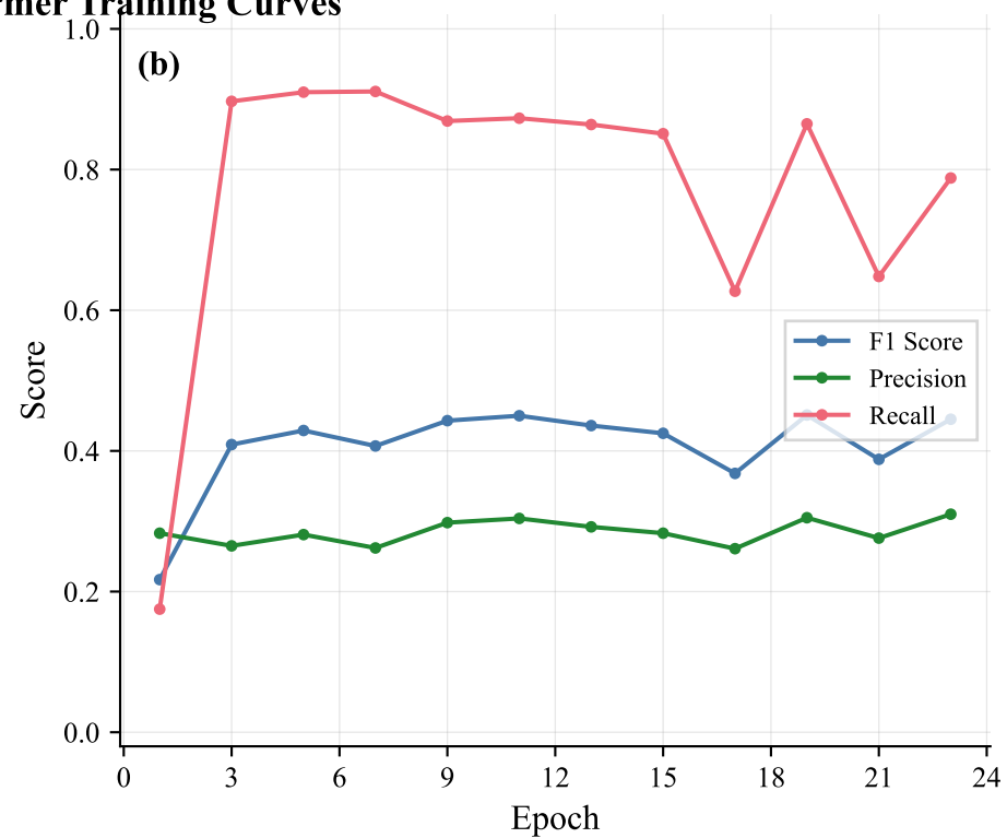
REFIT — CondiNILMformer Training Curves
