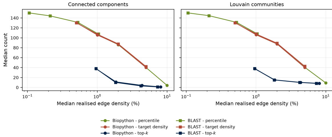
Figure 3: Median component and community counts against realised density for 12 graph settings and 50 reference-condition collections. Colour denotes rule family; marker denotes score method.
