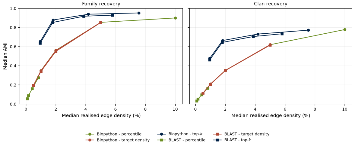
Figure 1: Median AMI against median realised density across 700 primary collections. Panels show family and clan recovery. Lines connect parameter values within each method and rule family.
