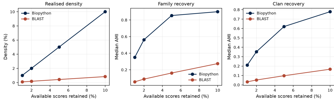
Figure 8: Median density, family AMI, and clan AMI under percentile rules. Horizontal position is fraction of available scores retained within each method. Summaries use 700 primary collections.
