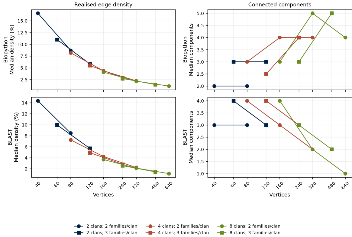
Figure 11: Top-5 graph structure across 14 primary composition conditions. Rows separate score methods. Colour gives clan count; marker gives families per clan. Lines connect domain counts.
