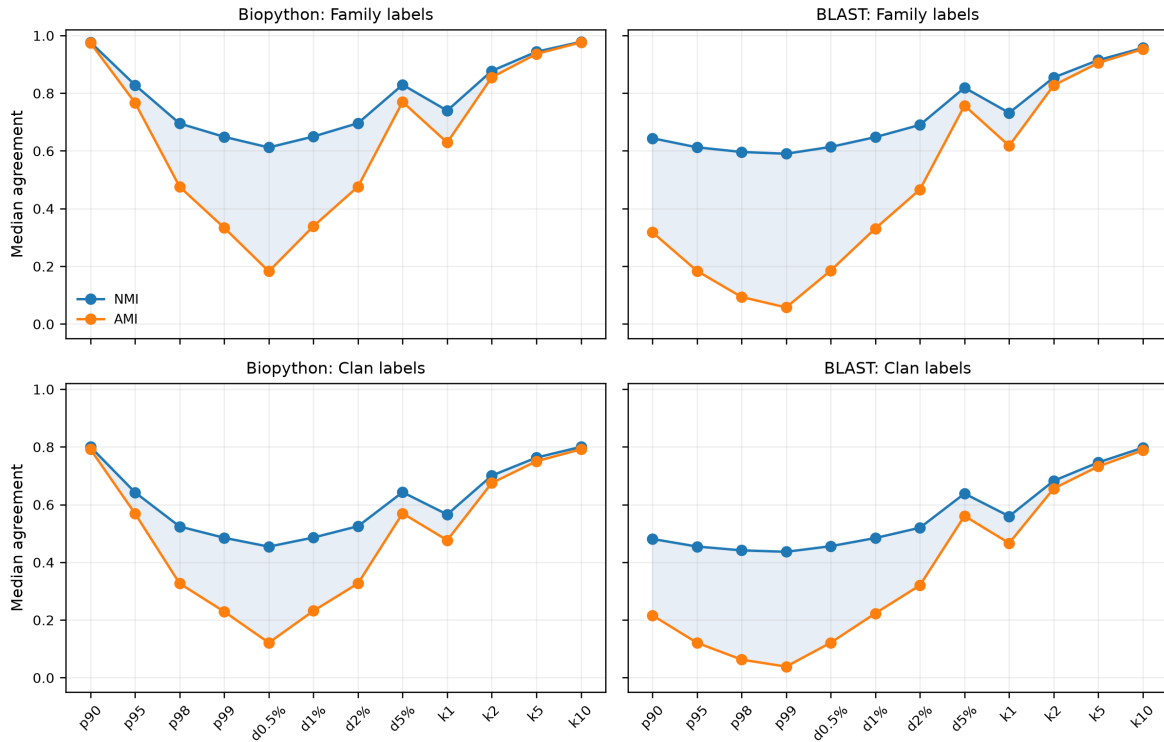
Figure 4: Median NMI and AMI for 12 graph settings in reference condition. Panels separate score method and withheld label level. Shading marks chance correction. Prefixes p , d , and k denote percentile, target density, and top- k .
