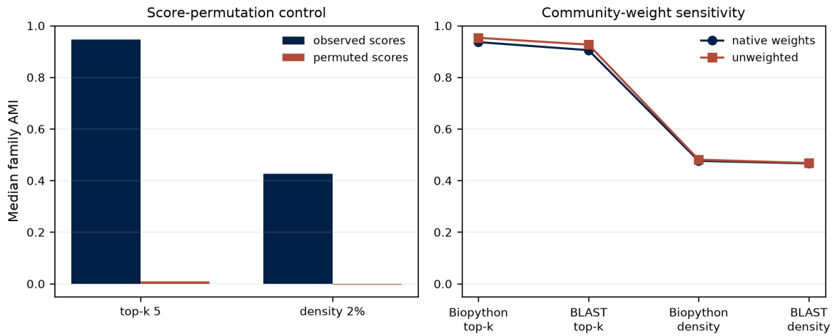
Figure 12: Sensitivity to score permutation and community weight.
