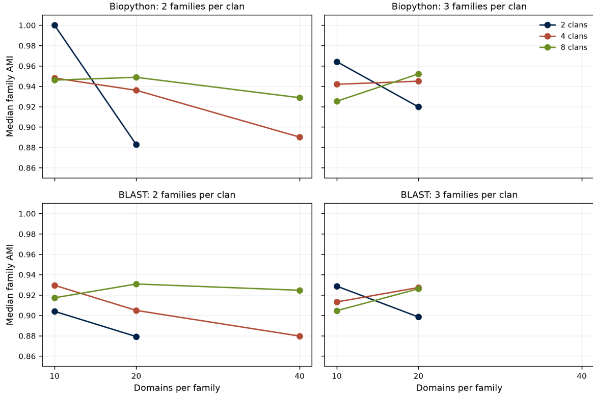
Figure 10: Median family AMI across 14 primary composition conditions under top-5 construction. Colour gives clan count; panels separate score method and families per clan. Lines connect domain counts.
