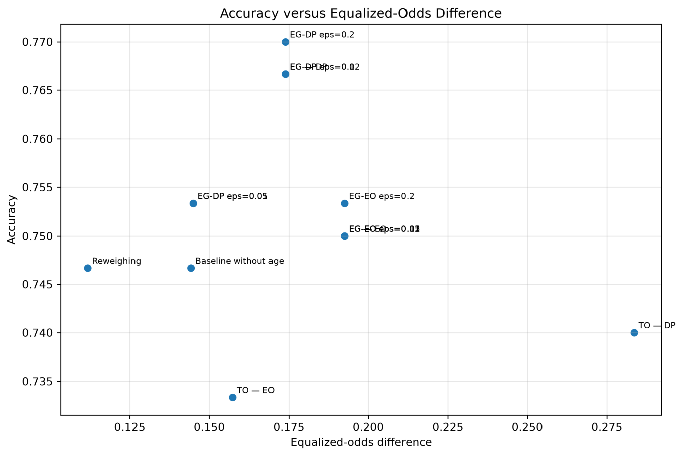
Figure 2: Accuracy versus equalized-odds difference
