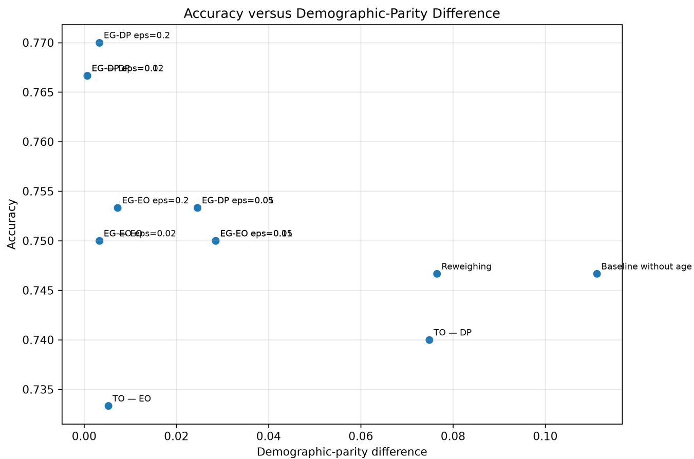
Figure 1: Accuracy versus demographic-parity difference
