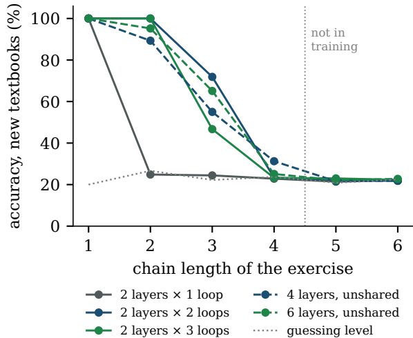
(a) final accuracy by chain length
