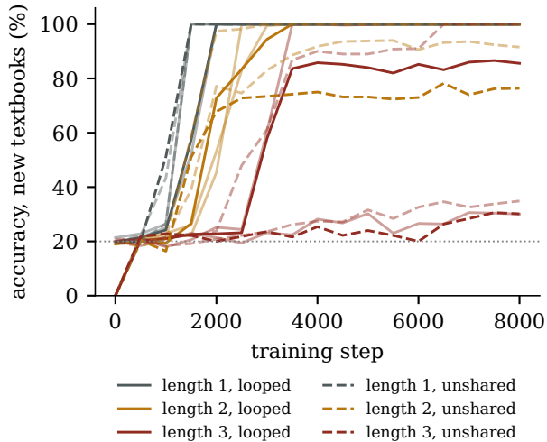
(b) four layer passes: looped vs. unshared
